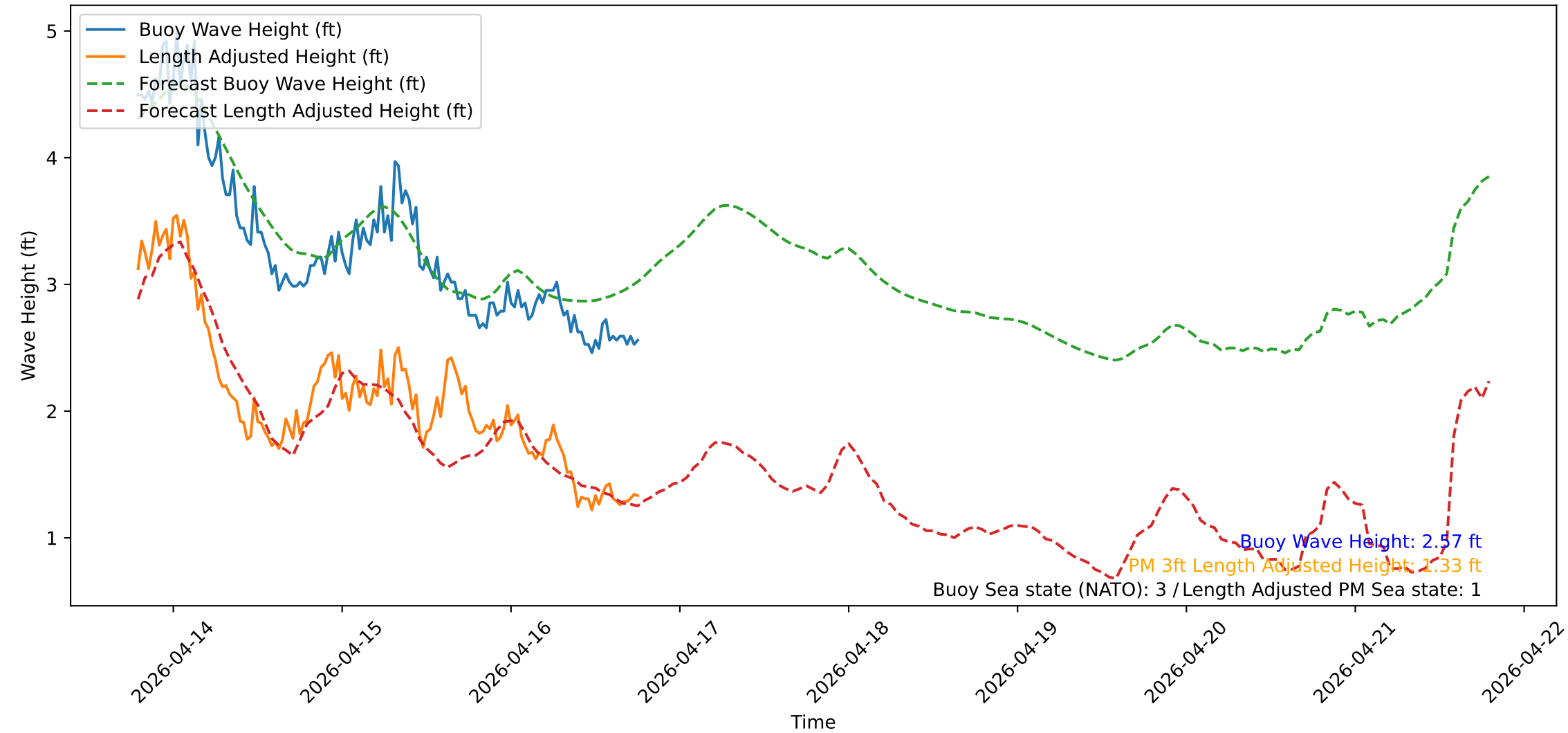
Wave Heights over Time for Green Beach at 2026-04-16 18:51:13
