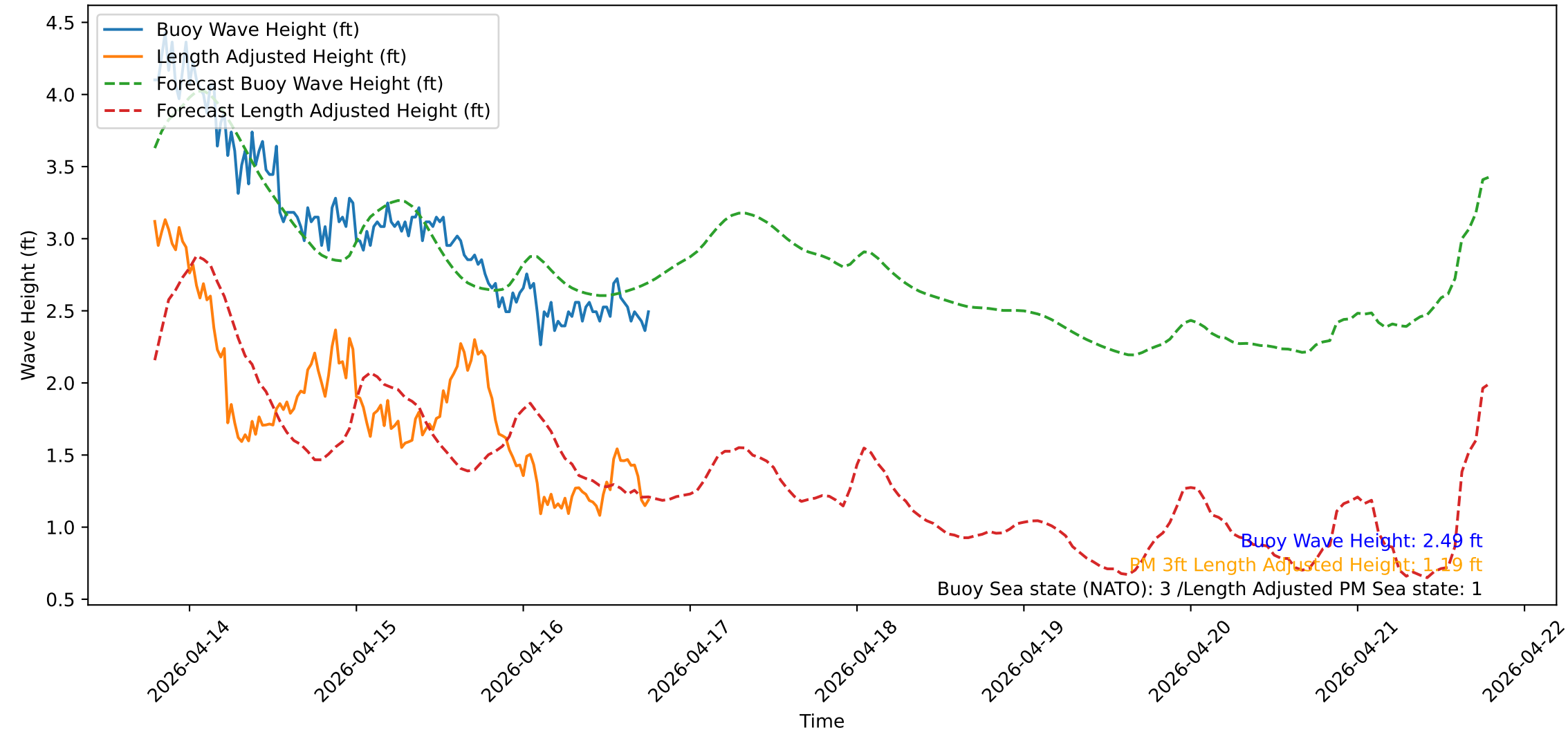
Wave Heights over Time for Red Beach at 2026-04-16 18:50:51
