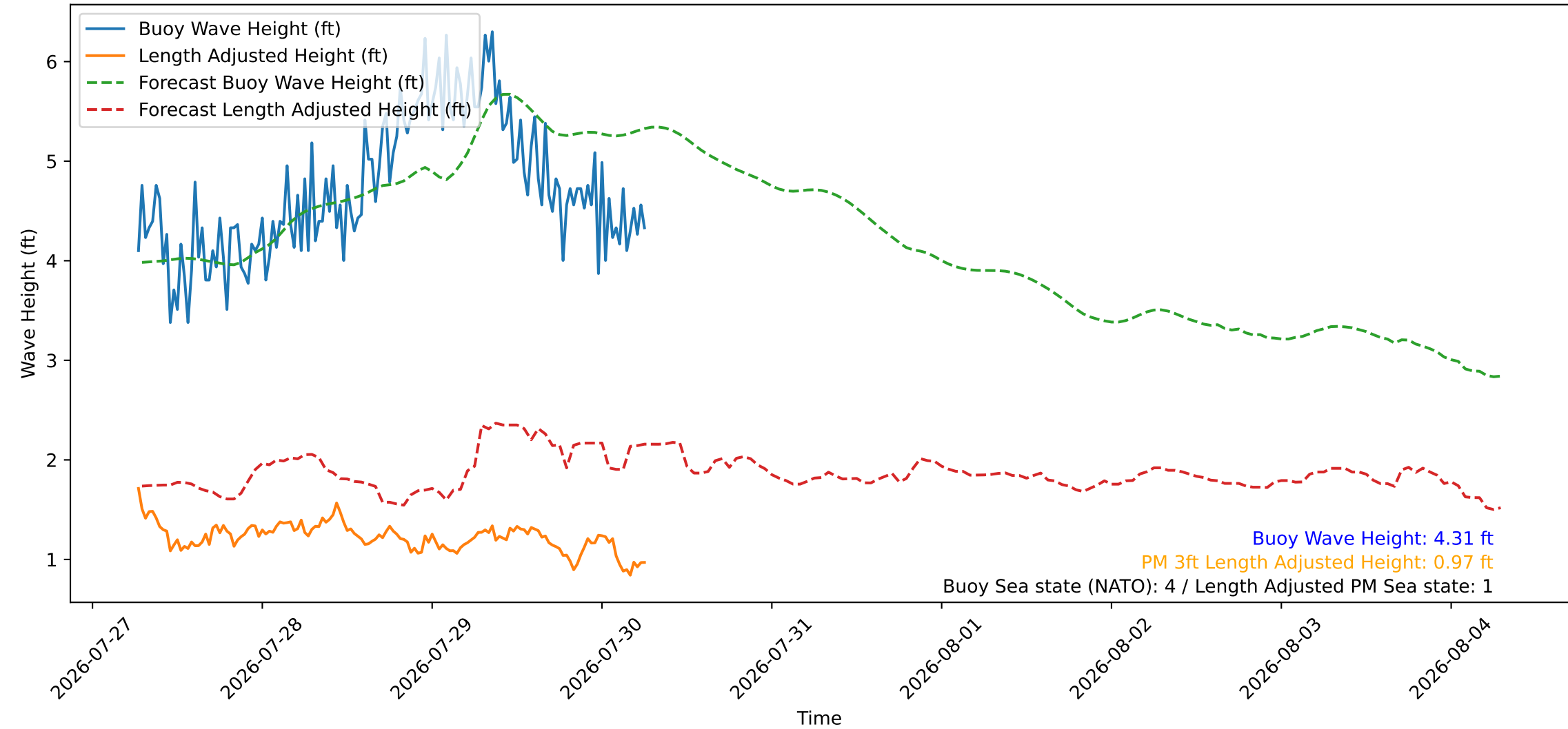
Wave Heights over Time for Green Beach at 2026-07-30 06:41:09
