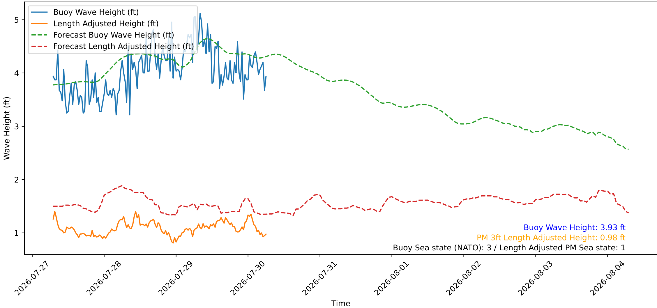
Wave Heights over Time for Red Beach at 2026-07-30 06:40:46
