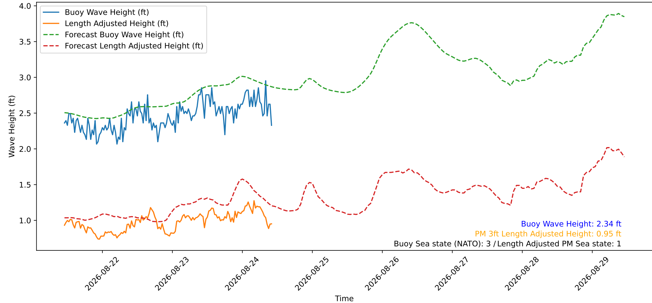
Wave Heights over Time for Red Beach at 2026-08-24 10:50:51
