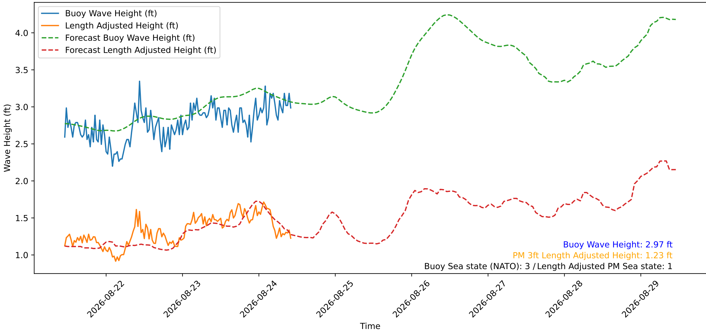
Wave Heights over Time for Oceanside Harbor at 2026-08-24 10:50:30
