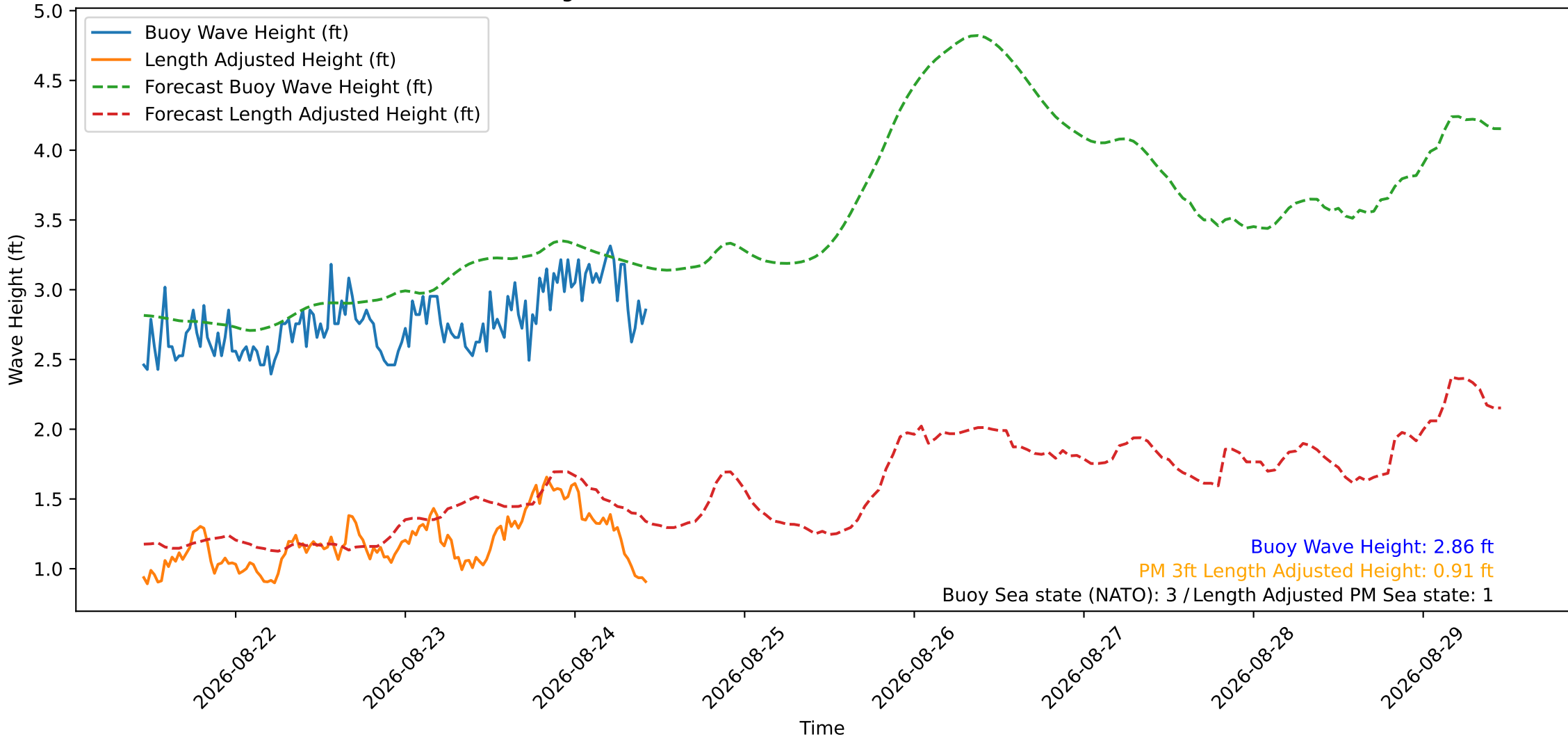
Wave Heights over Time for Green Beach at 2026-08-24 10:51:14
