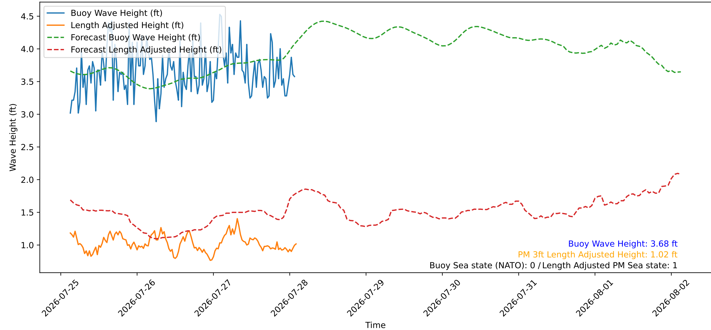
Wave Heights over Time for Red Beach at 2026-07-28 02:50:46
