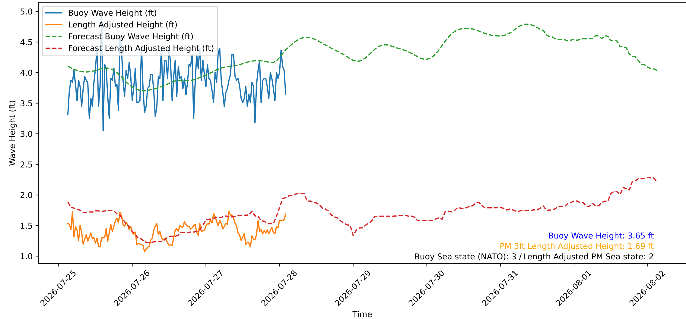
Wave Heights over Time for Oceanside Harbor at 2026-07-28 02:50:26
