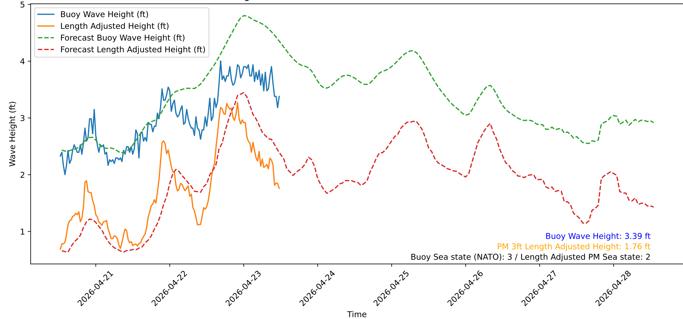
Wave Heights over Time for Green Beach at 2026-04-23 12:31:11
