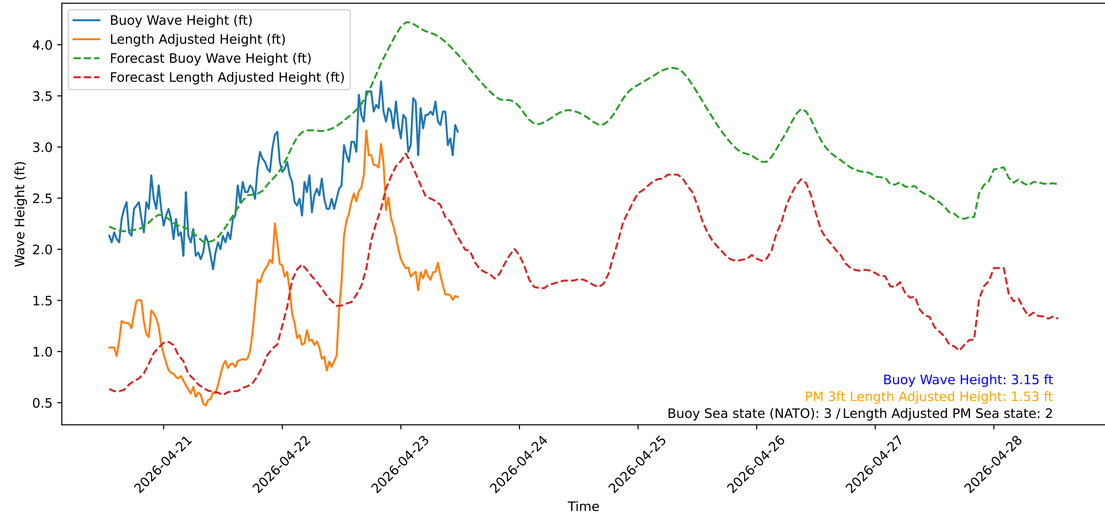
Wave Heights over Time for Red Beach at 2026-04-23 12:30:50
