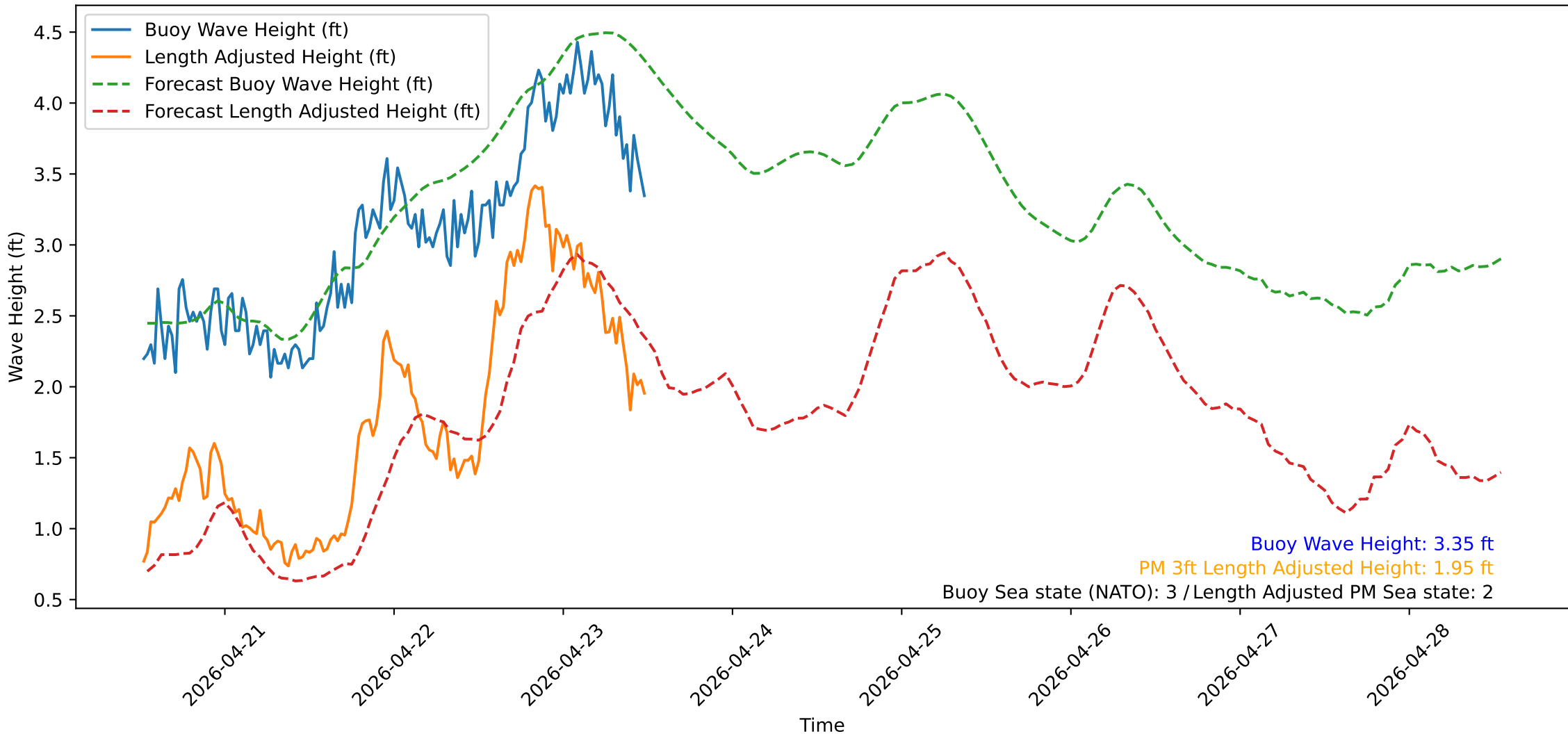
Wave Heights over Time for Oceanside Harbor at 2026-04-23 12:30:31
