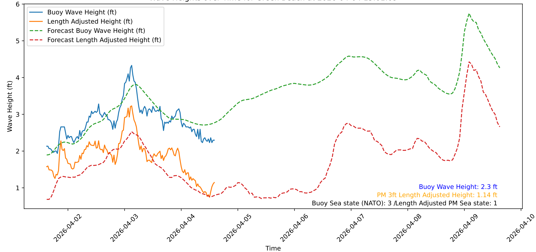
Wave Heights over Time for Green Beach at 2026-04-04 15:01:09
