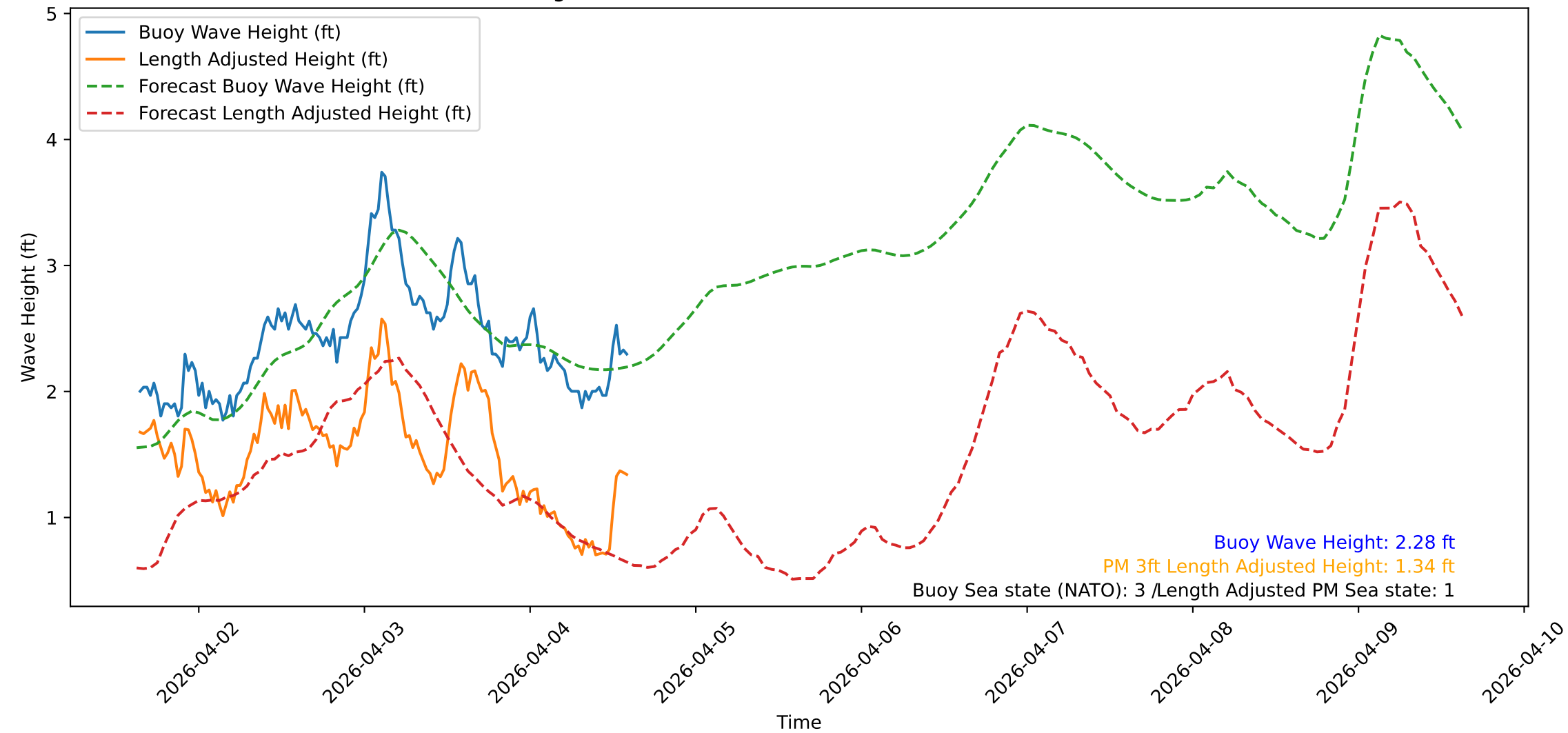
Wave Heights over Time for Red Beach at 2026-04-04 15:00:47
