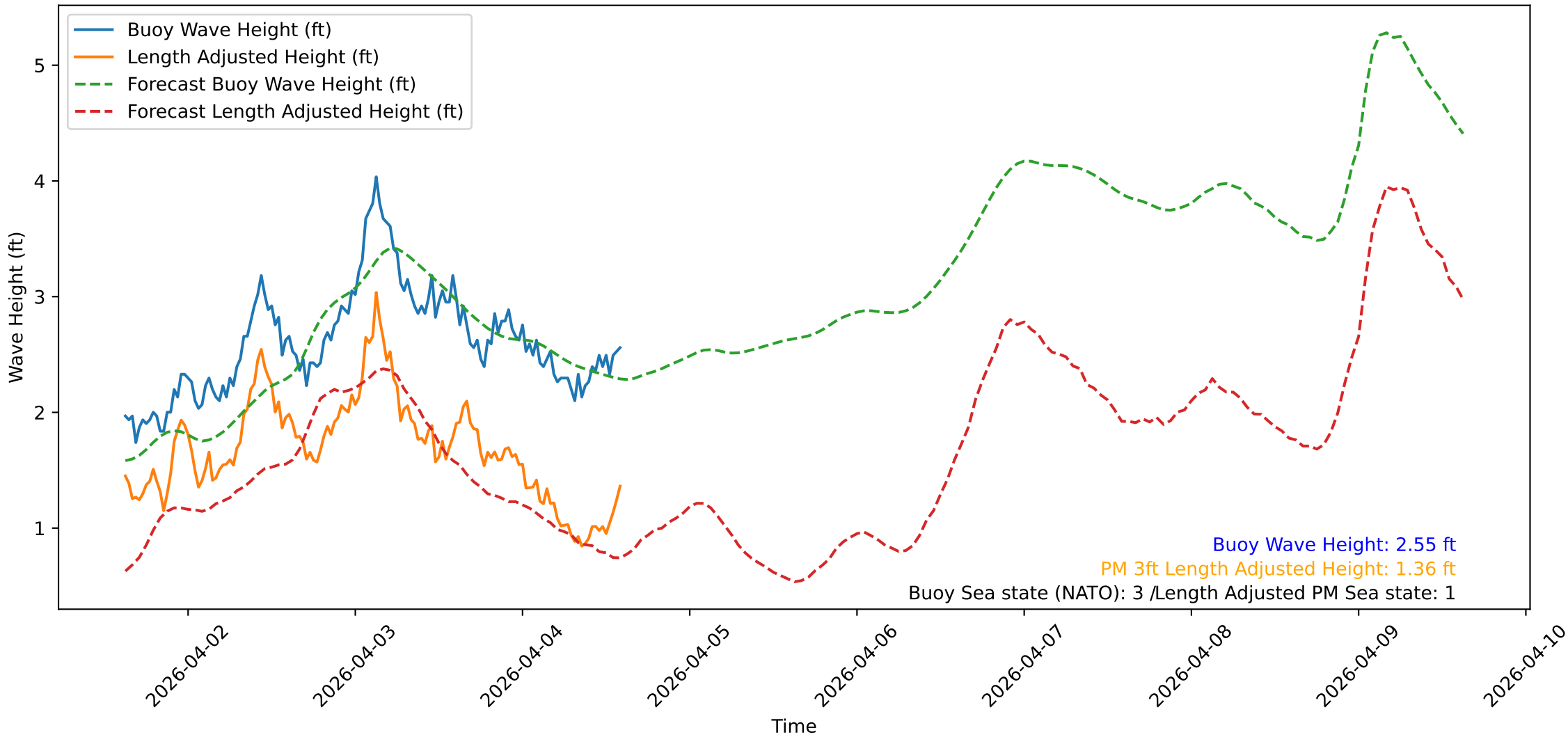
Wave Heights over Time for Oceanside Harbor at 2026-04-04 15:00:31
