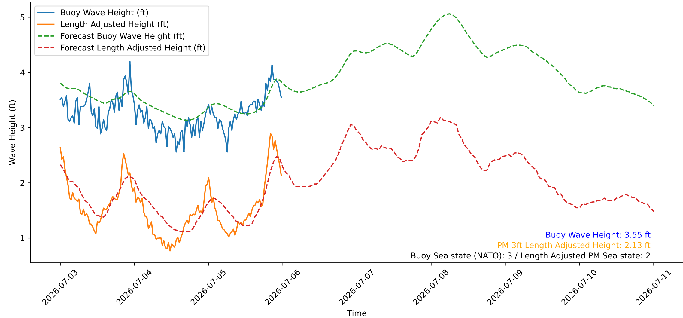
Wave Heights over Time for Green Beach at 2026-07-06 00:11:08
