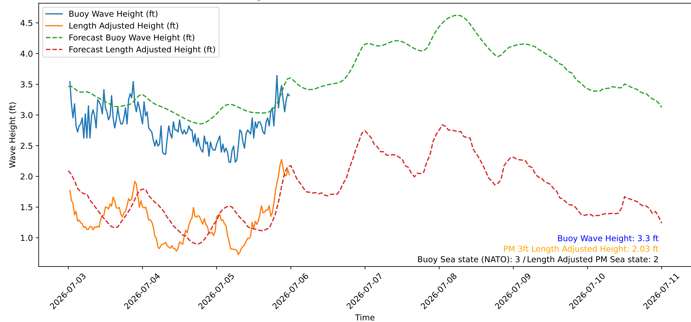
Wave Heights over Time for Red Beach at 2026-07-06 00:10:46
