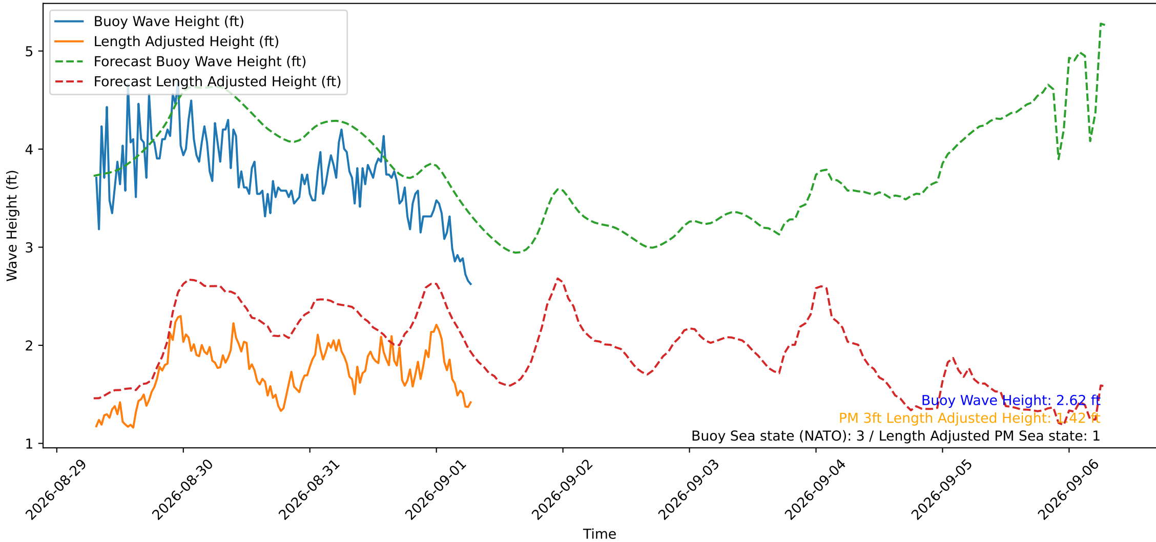
Wave Heights over Time for Red Beach at 2026-09-01 07:10:50
