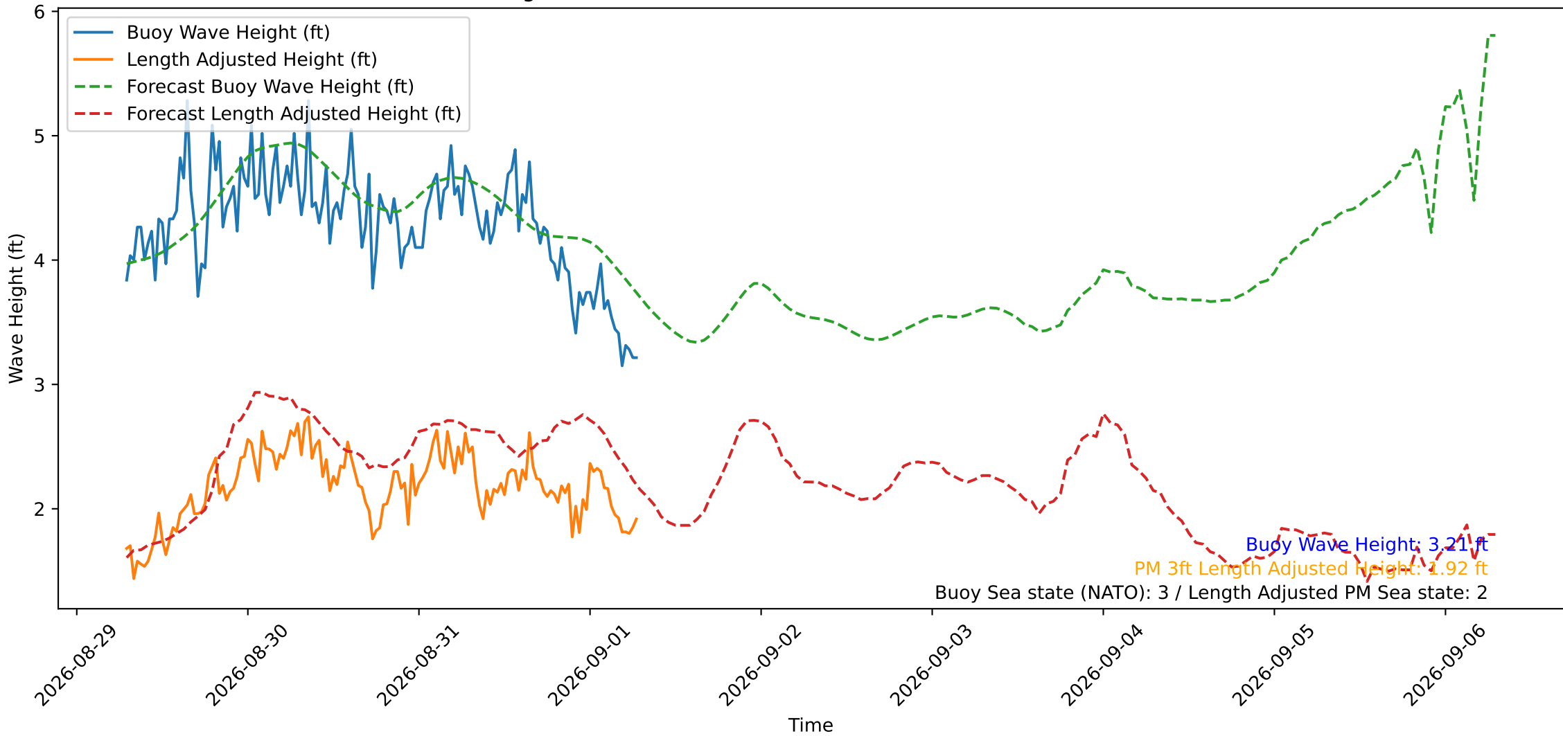
Wave Heights over Time for Oceanside Harbor at 2026-09-01 07:10:30
