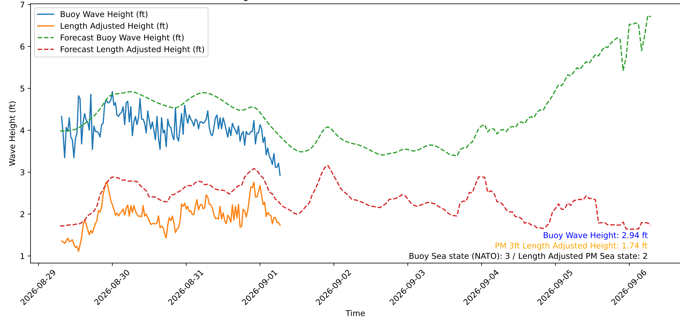
Wave Heights over Time for Green Beach at 2026-09-01 07:11:12
