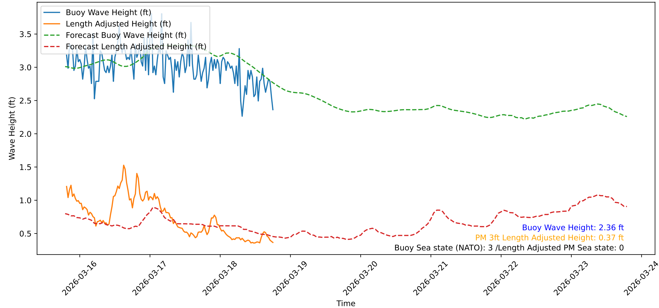
Wave Heights over Time for Red Beach at 2026-03-18 19:00:48
