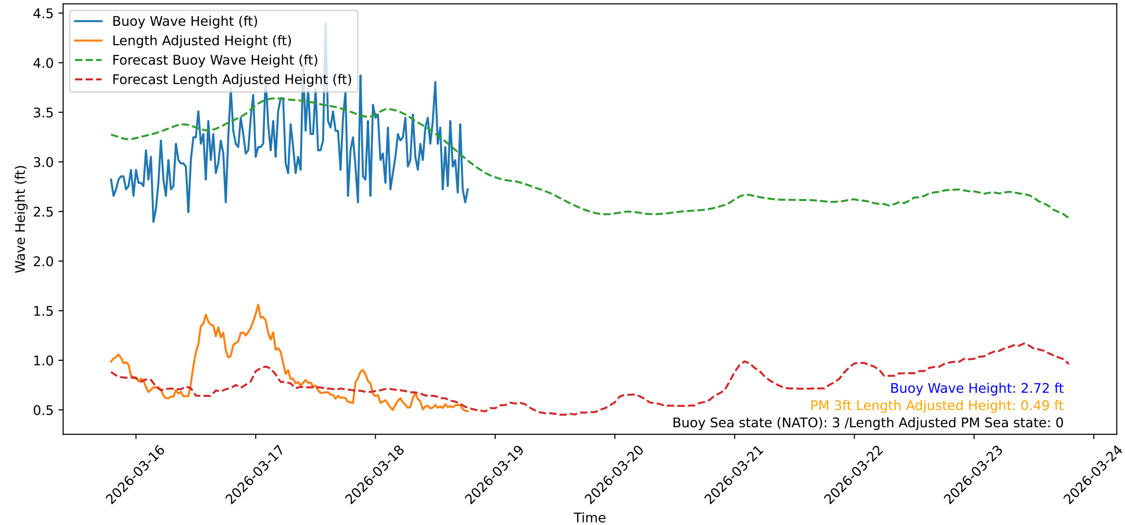
Wave Heights over Time for Oceanside Harbor at 2026-03-18 19:00:32
