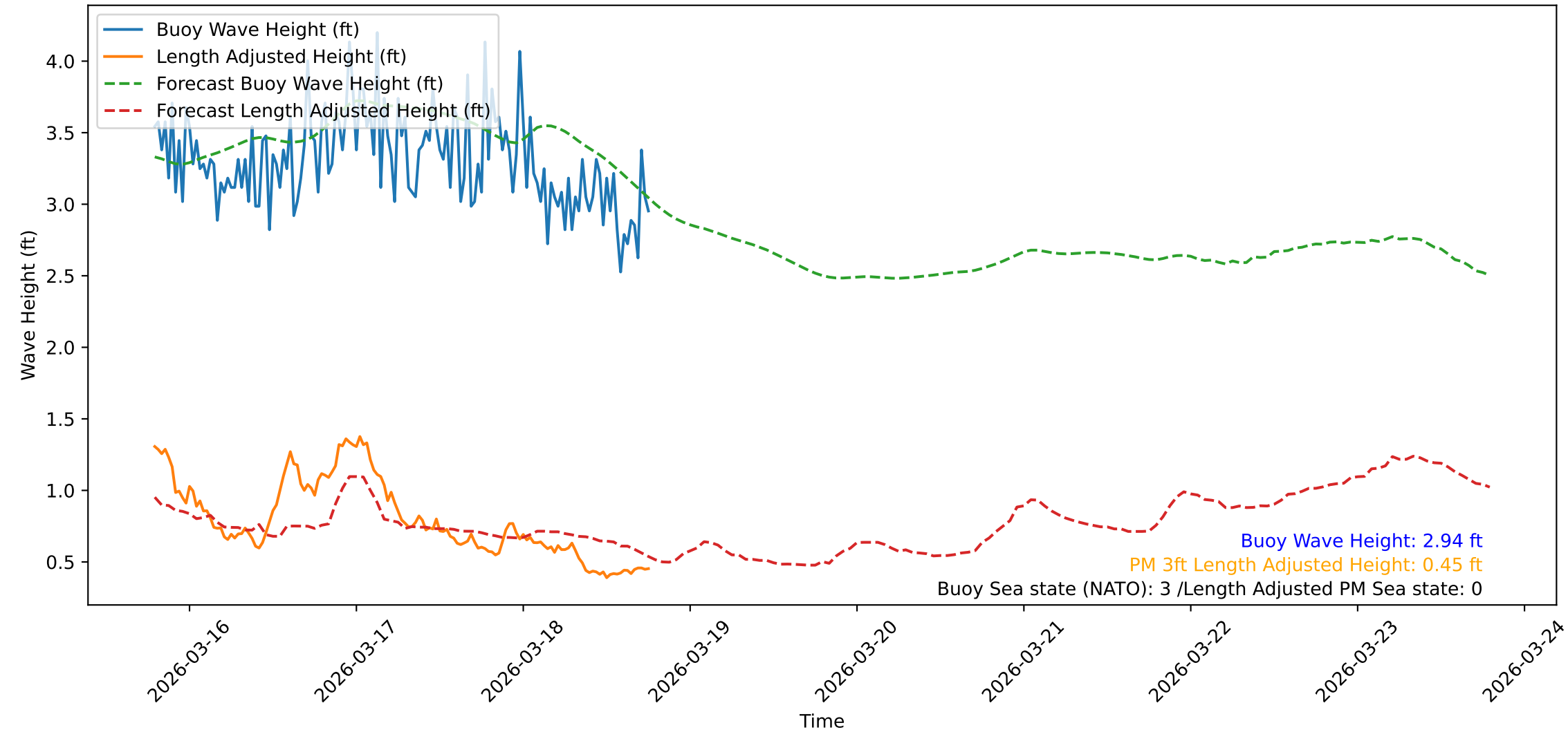
Wave Heights over Time for Green Beach at 2026-03-18 19:01:10
