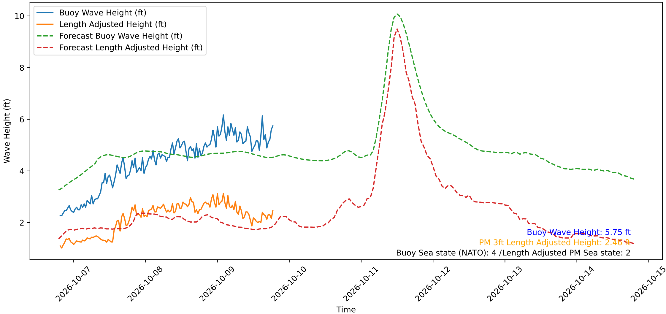
Wave Heights over Time for Green Beach at 2026-10-09 19:11:12
