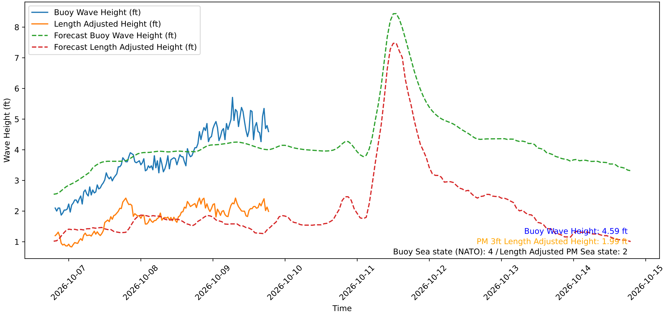
Wave Heights over Time for Red Beach at 2026-10-09 19:10:50
