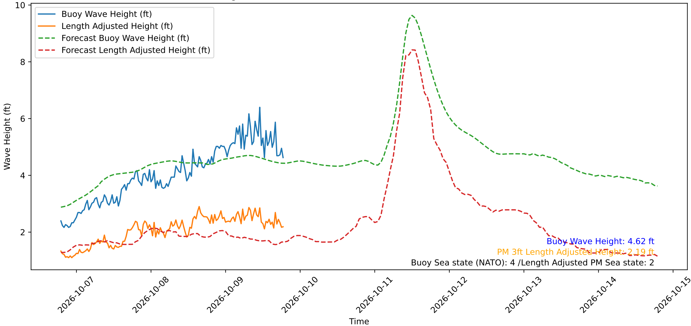
Wave Heights over Time for Oceanside Harbor at 2026-10-09 19:10:30
