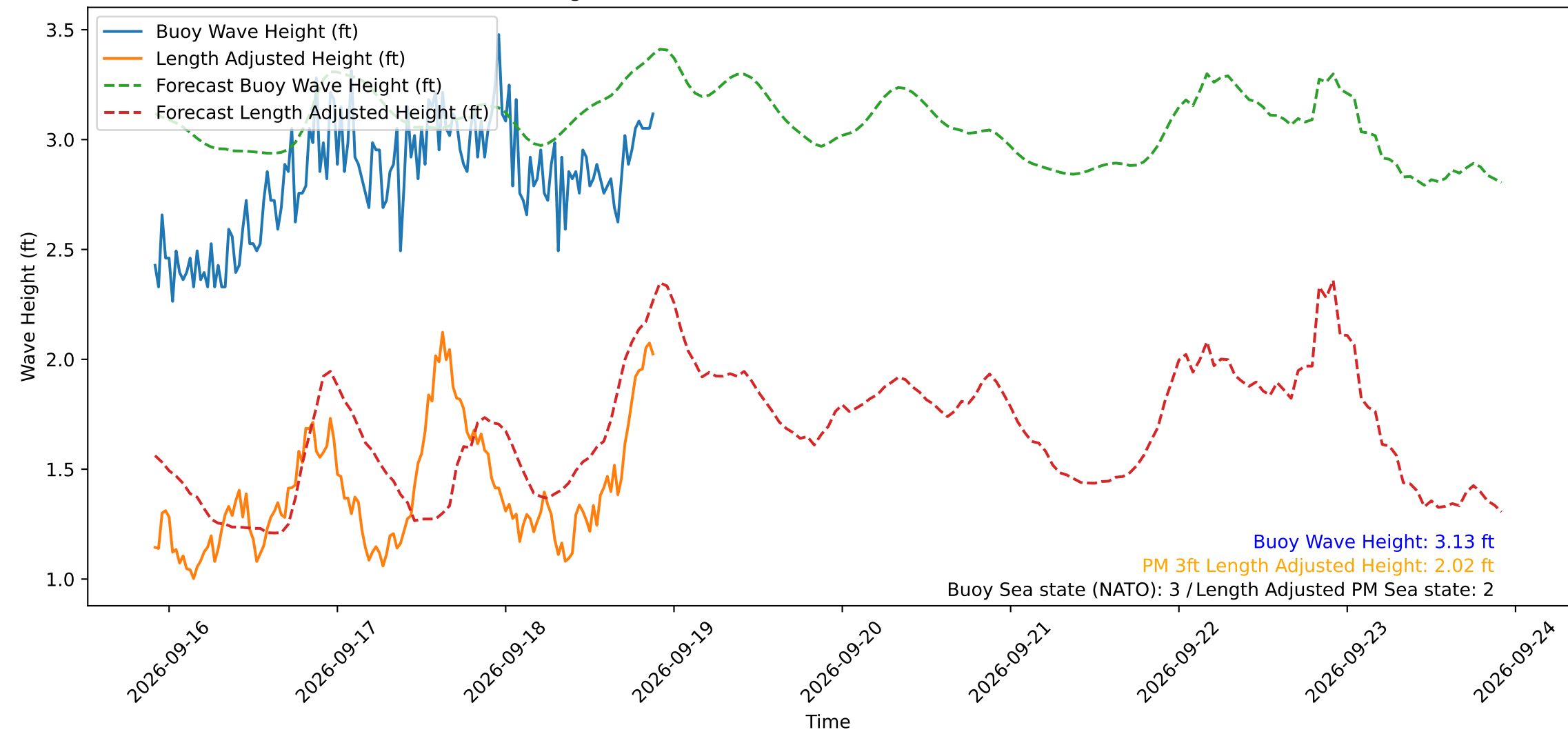
Wave Heights over Time for Green Beach at 2026-09-18 21:51:13
