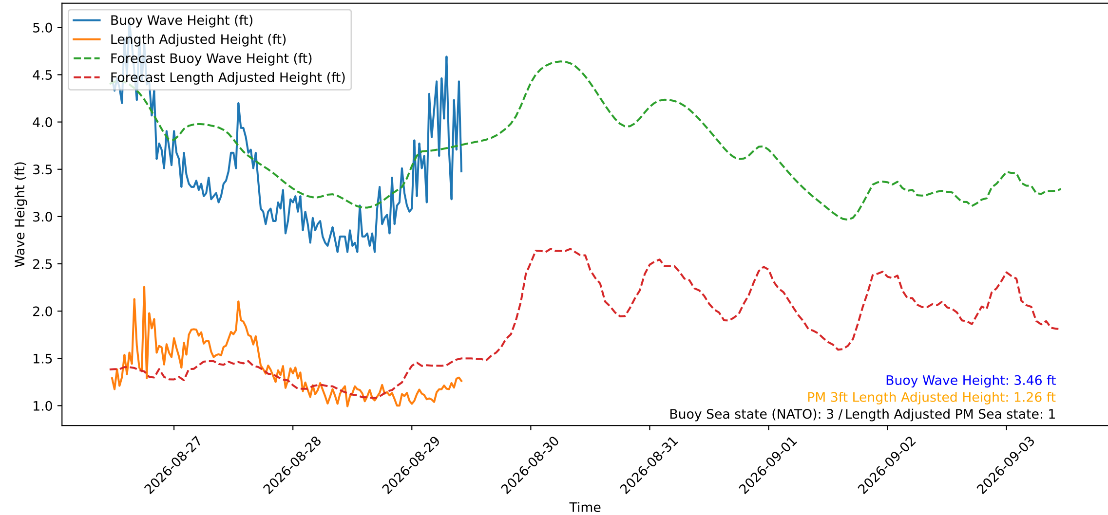
Wave Heights over Time for Red Beach at 2026-08-29 11:00:49
