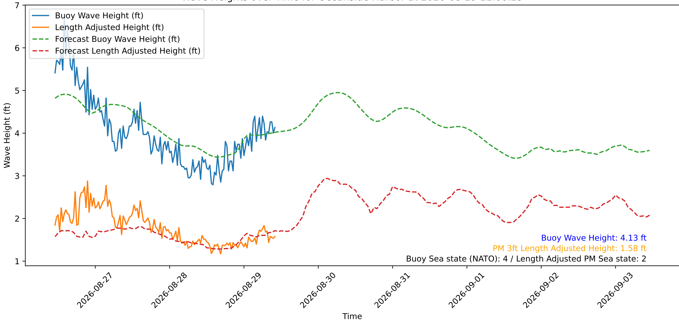
Wave Heights over Time for Oceanside Harbor at 2026-08-29 11:00:29
