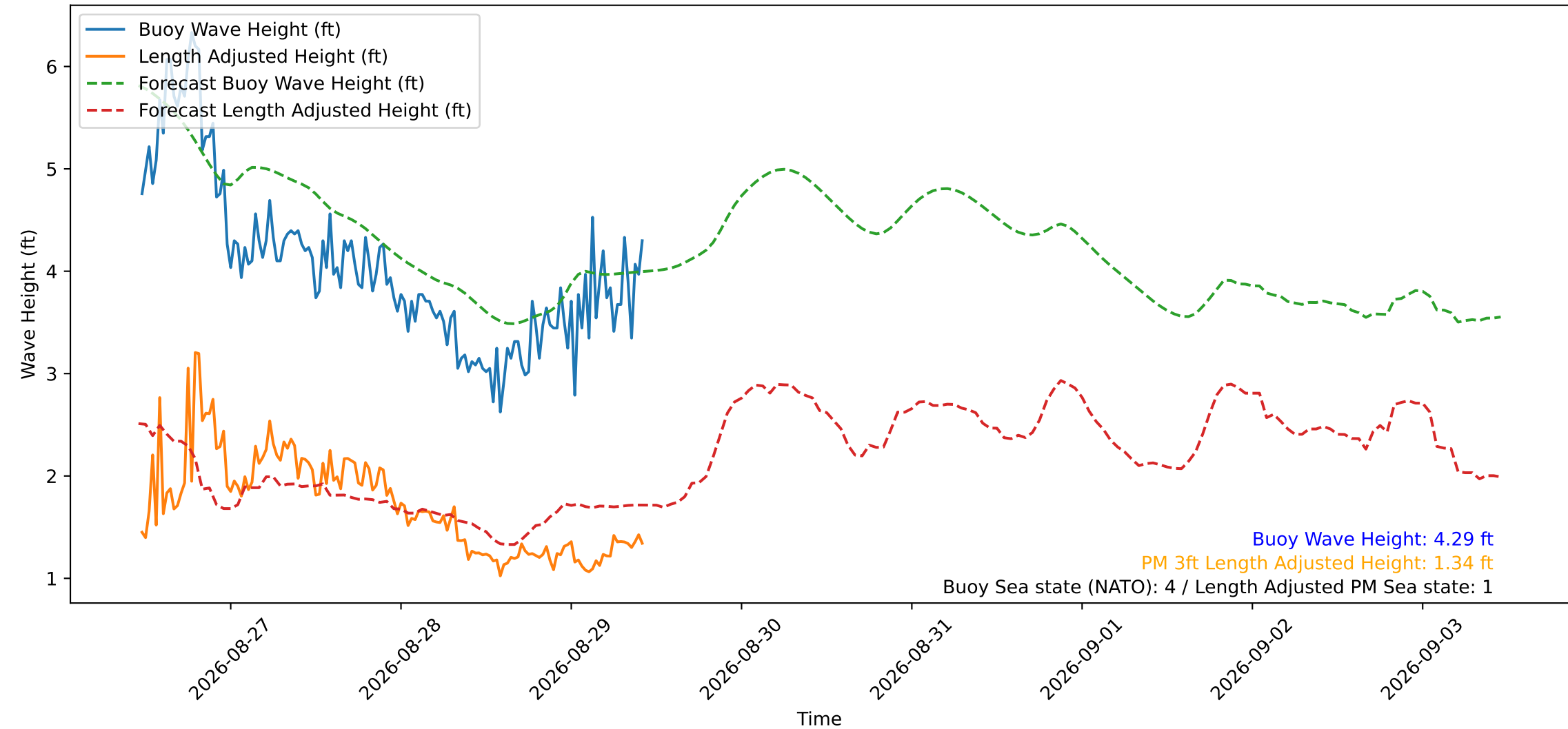
Wave Heights over Time for Green Beach at 2026-08-29 11:01:12
