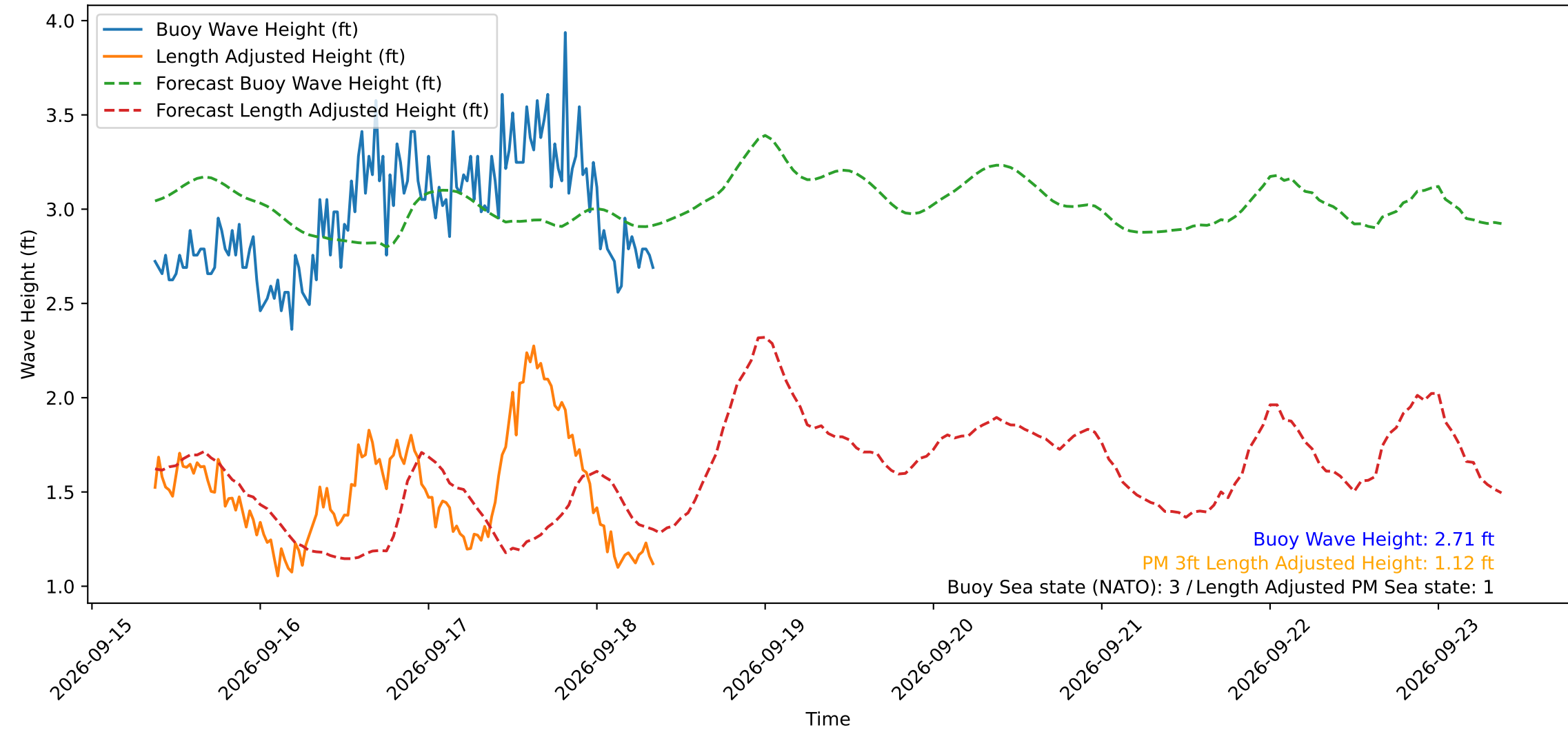
Wave Heights over Time for Oceanside Harbor at 2026-09-18 08:50:30
