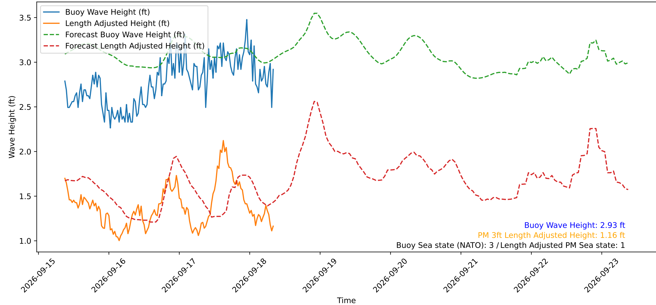
Wave Heights over Time for Green Beach at 2026-09-18 08:51:14
