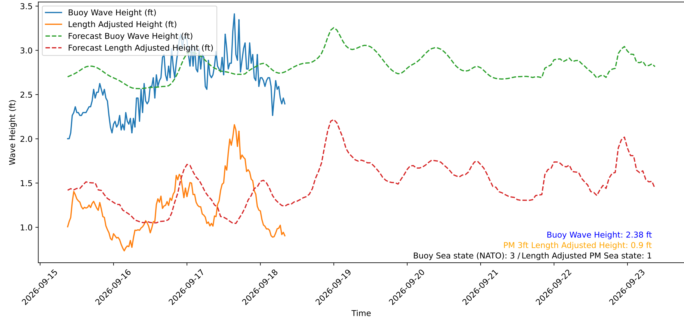
Wave Heights over Time for Red Beach at 2026-09-18 08:50:50
