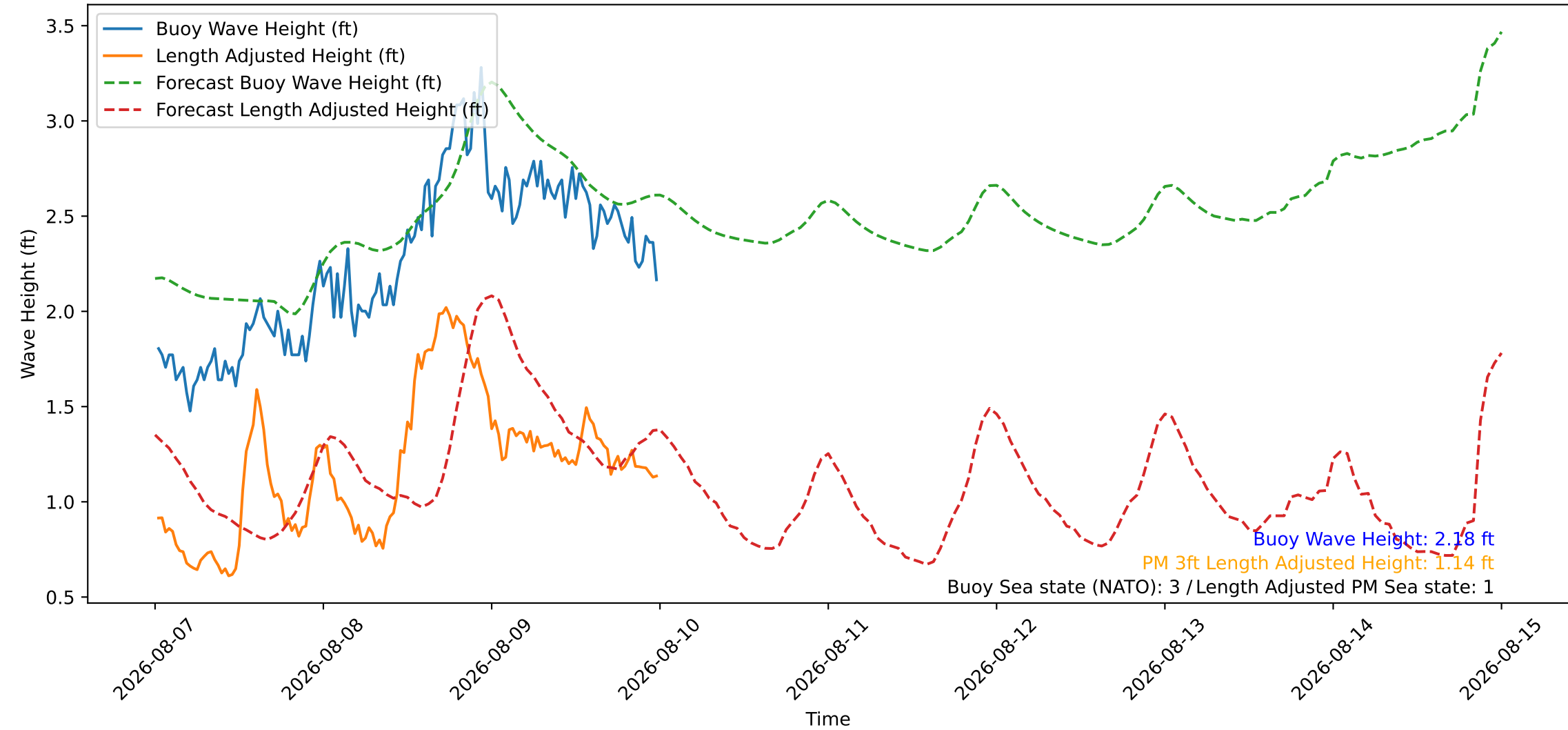
Wave Heights over Time for Red Beach at 2026-08-10 00:10:45
