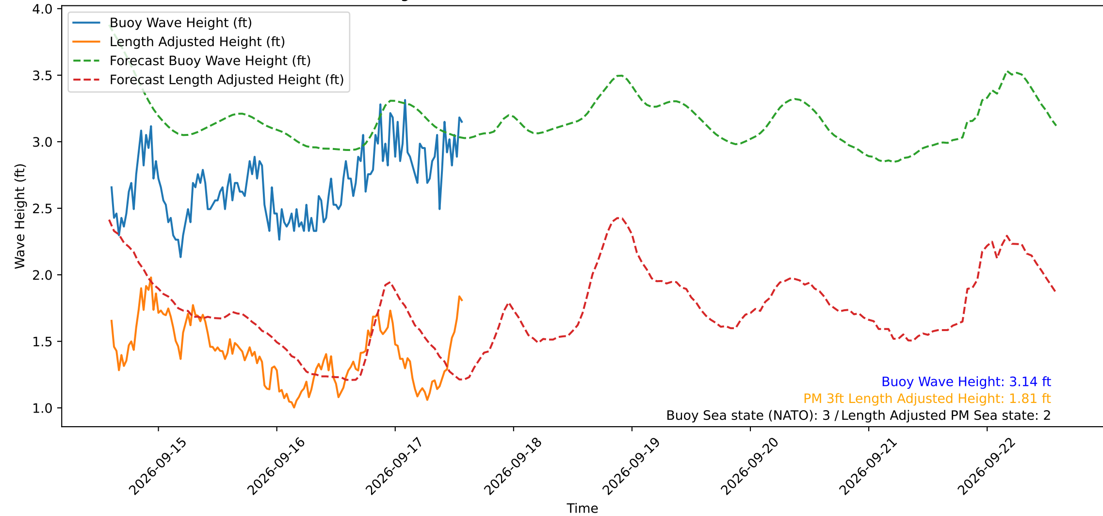
Wave Heights over Time for Green Beach at 2026-09-17 14:11:12
