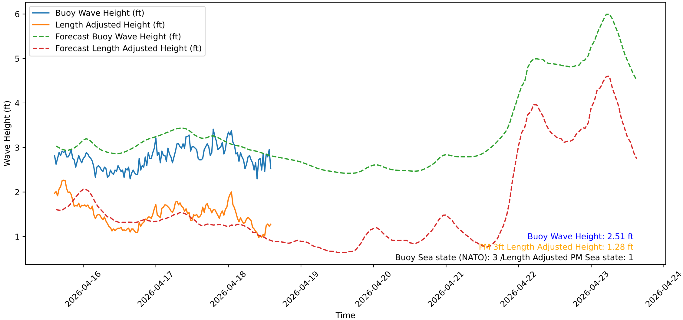
Wave Heights over Time for Oceanside Harbor at 2026-04-18 14:30:31
