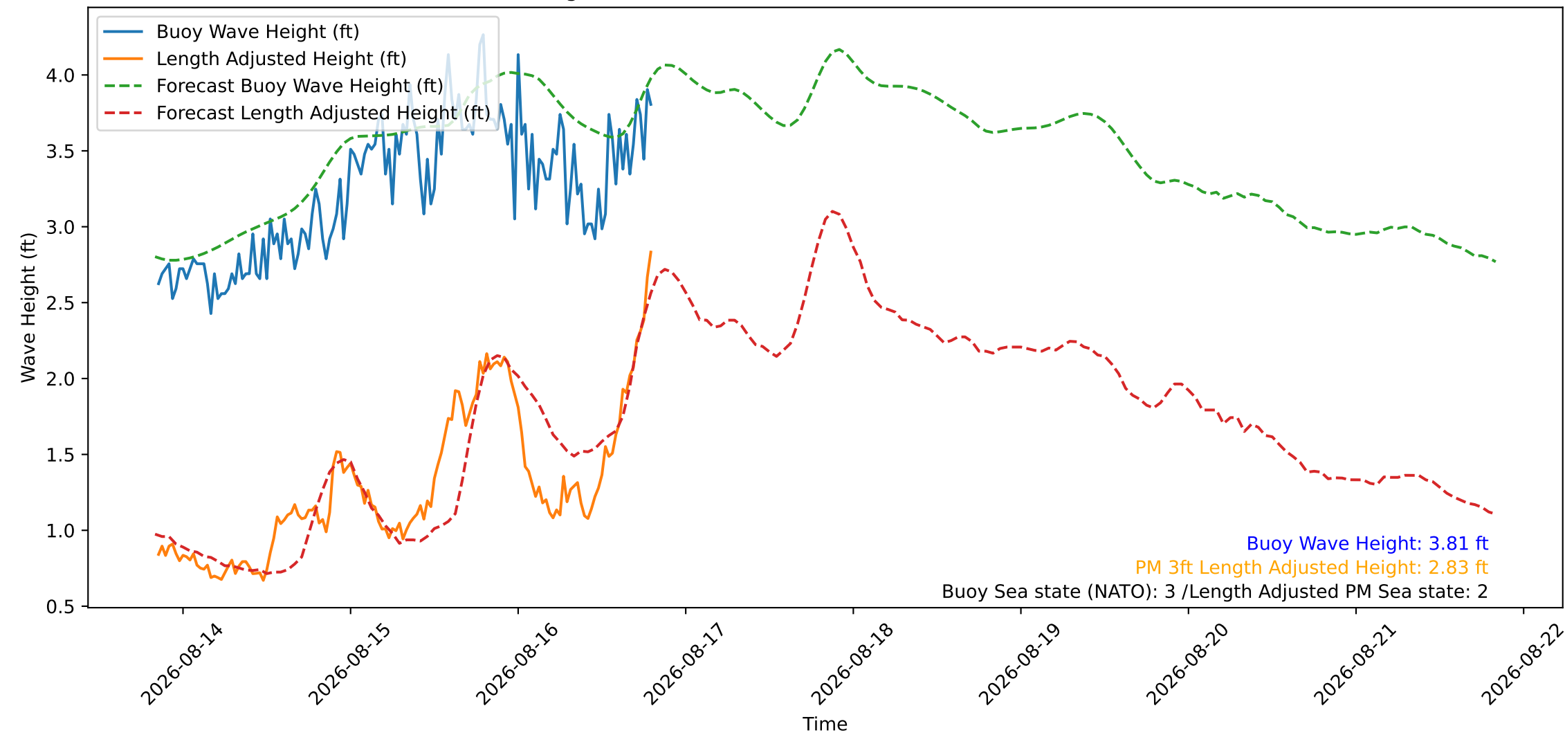
Wave Heights over Time for Green Beach at 2026-08-16 20:01:08
