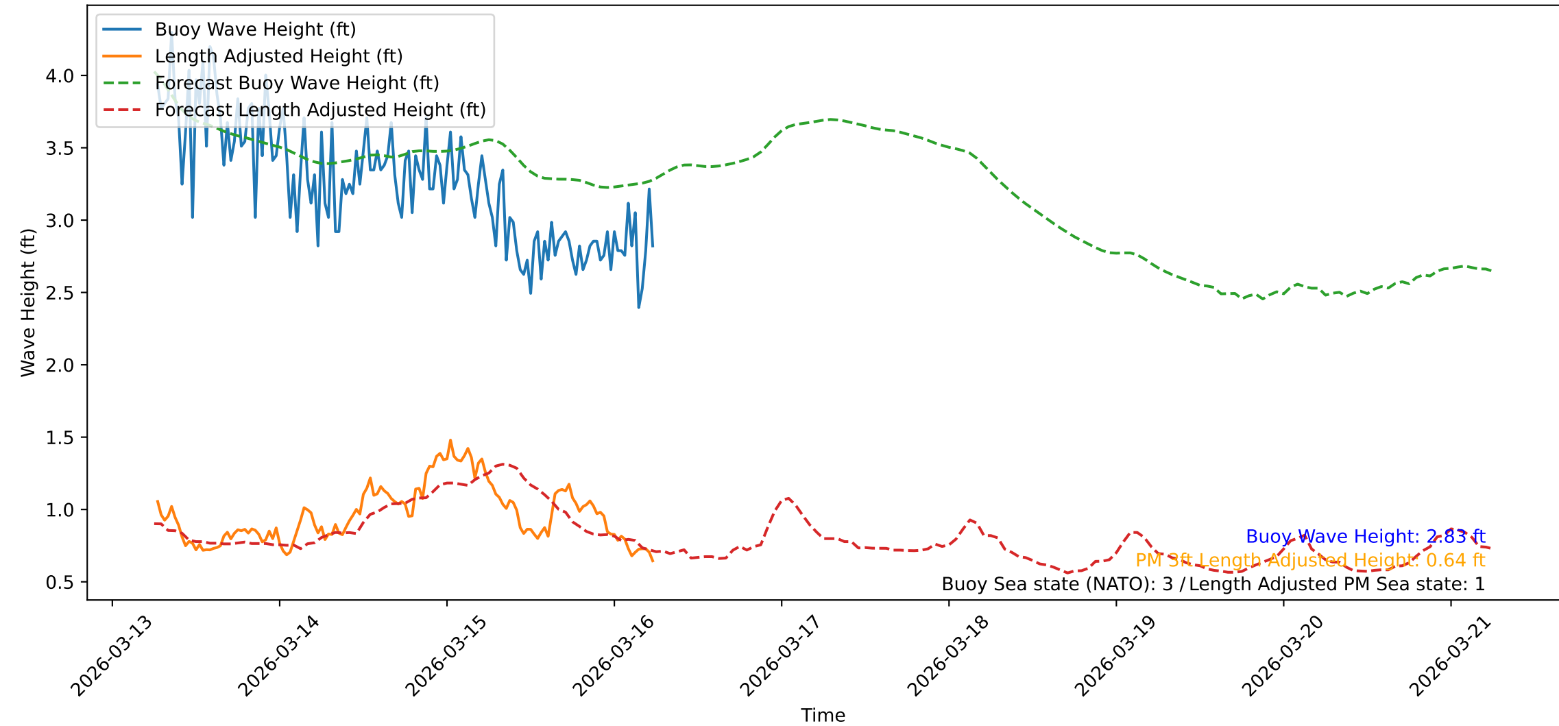
Wave Heights over Time for Oceanside Harbor at 2026-03-16 06:20:42
