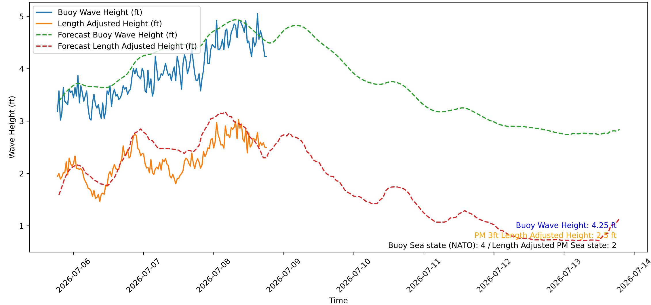
Wave Heights over Time for Oceanside Harbor at 2026-07-08 18:40:27
