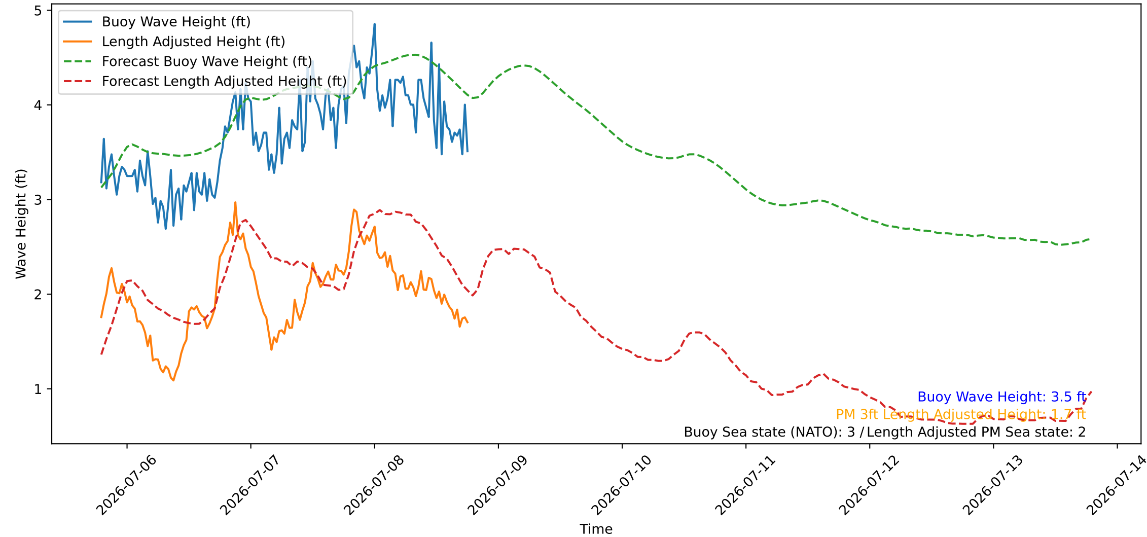
Wave Heights over Time for Red Beach at 2026-07-08 18:40:46
