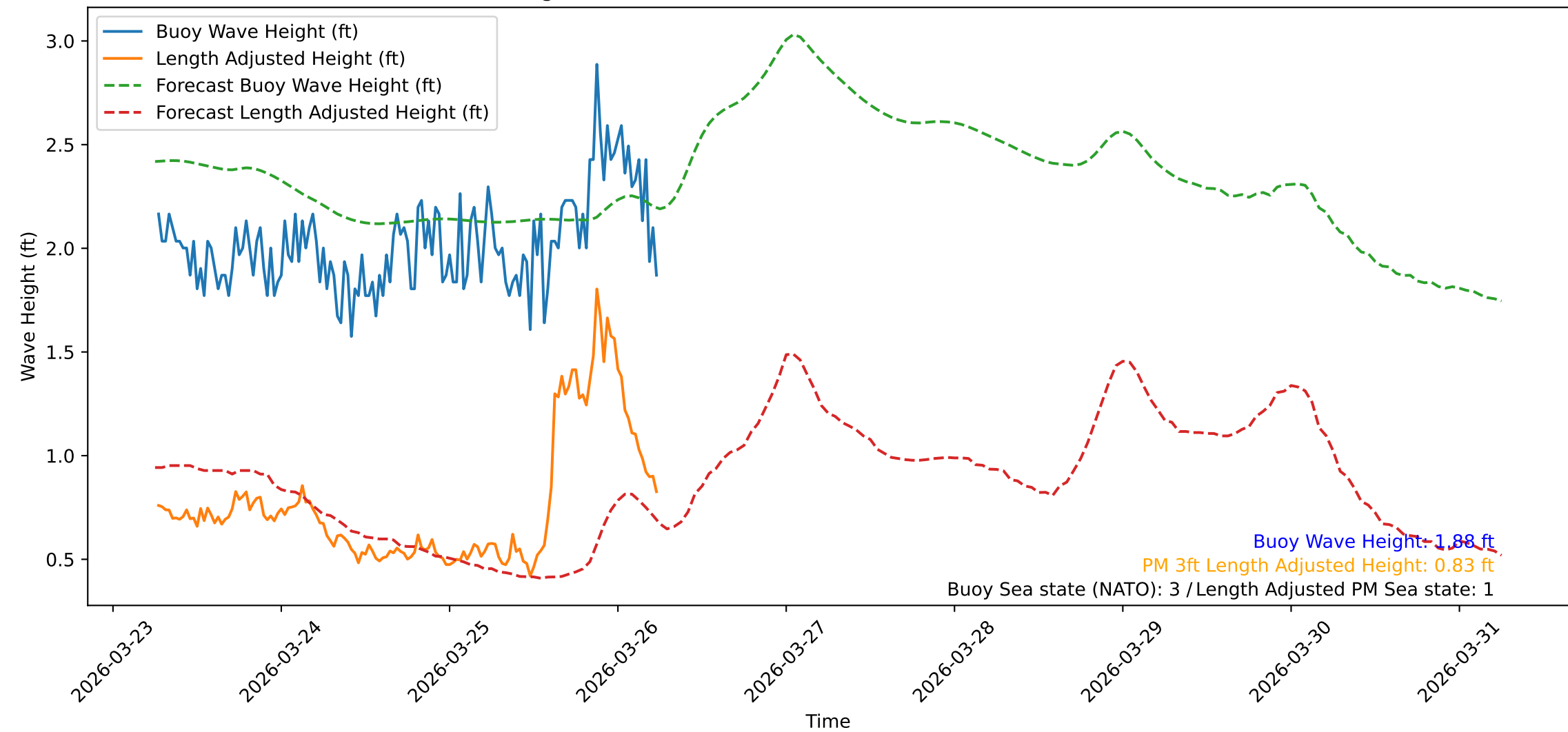
Wave Heights over Time for Oceanside Harbor at 2026-03-26 06:20:32
