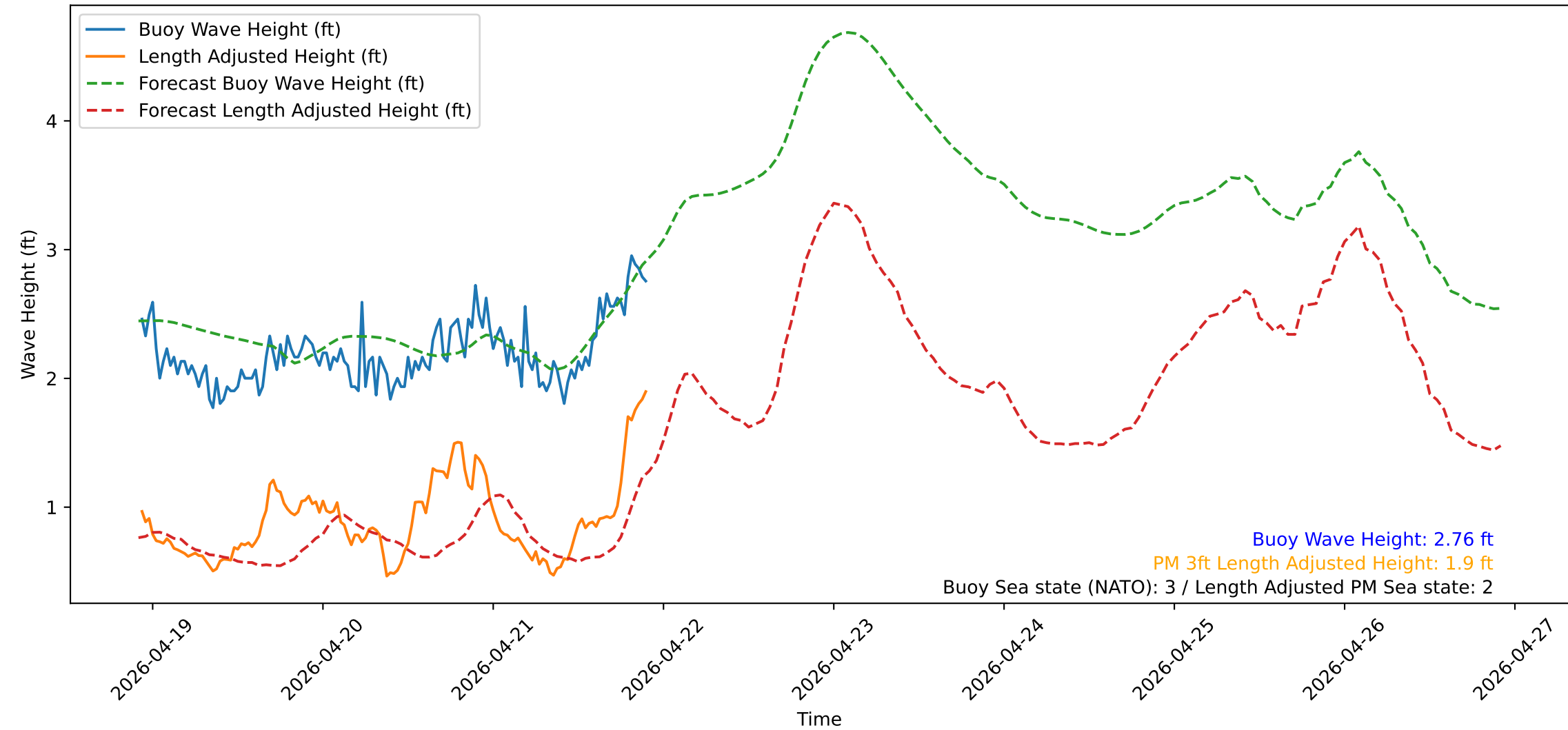
Wave Heights over Time for Red Beach at 2026-04-21 22:10:51
