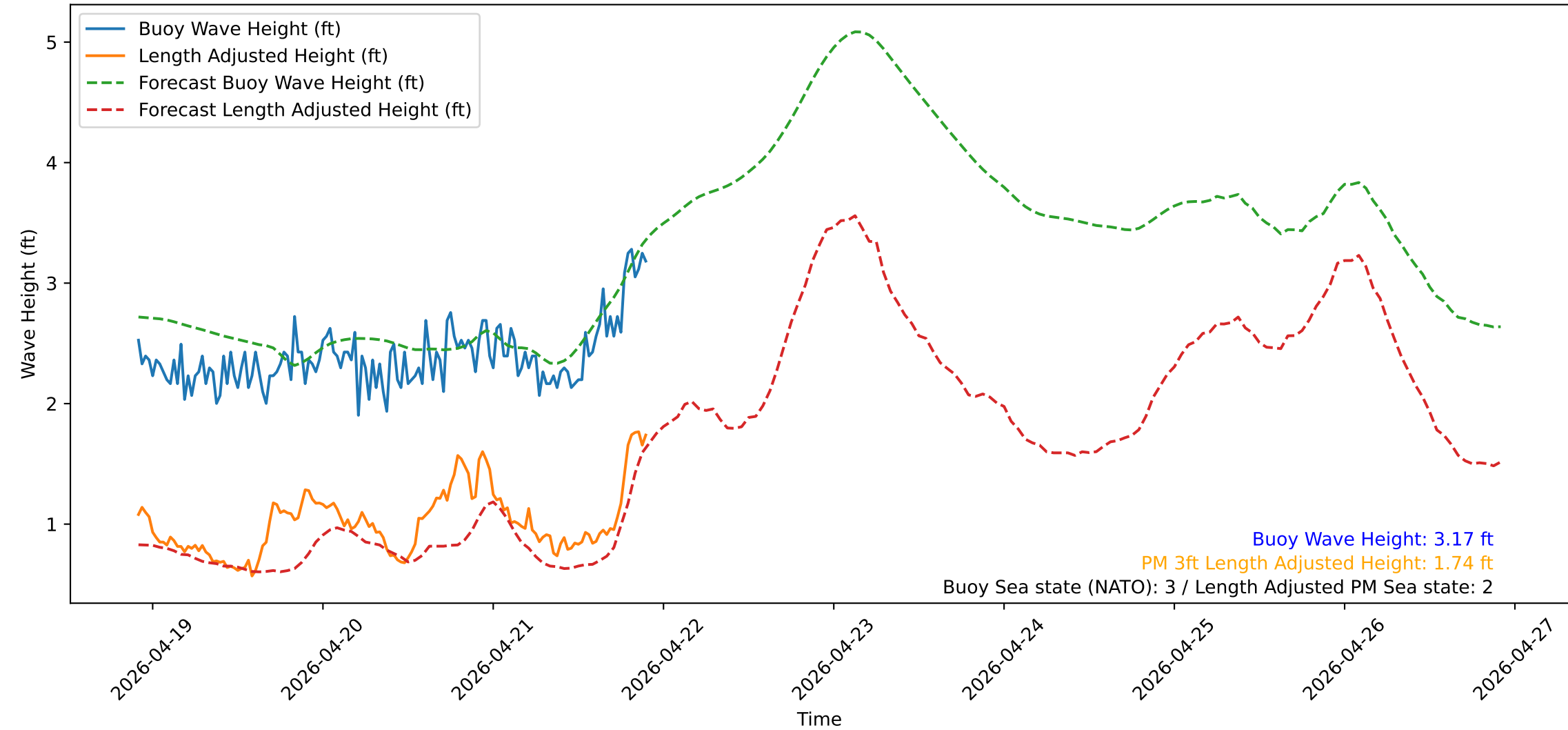
Wave Heights over Time for Oceanside Harbor at 2026-04-21 22:10:31
