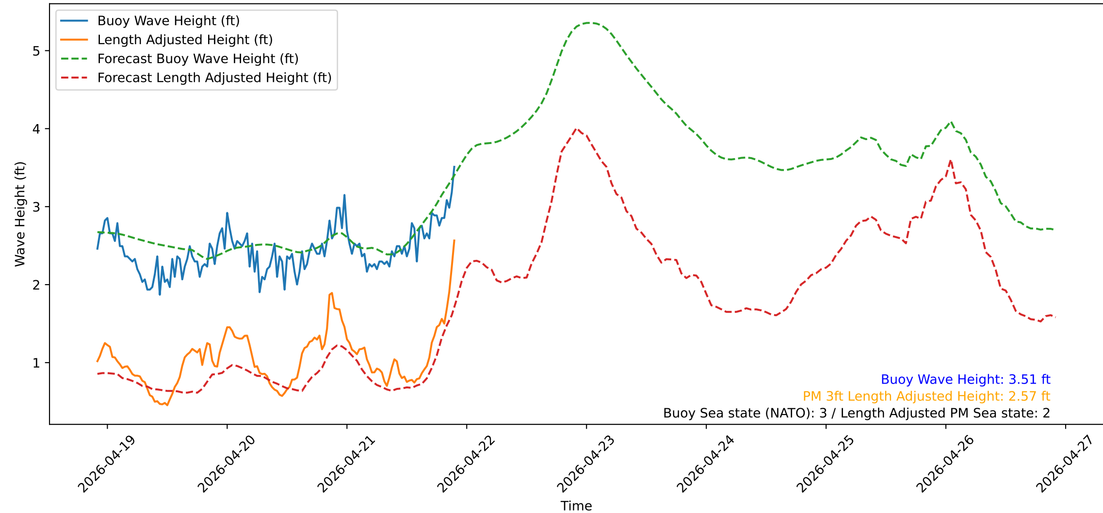
Wave Heights over Time for Green Beach at 2026-04-21 22:11:13
