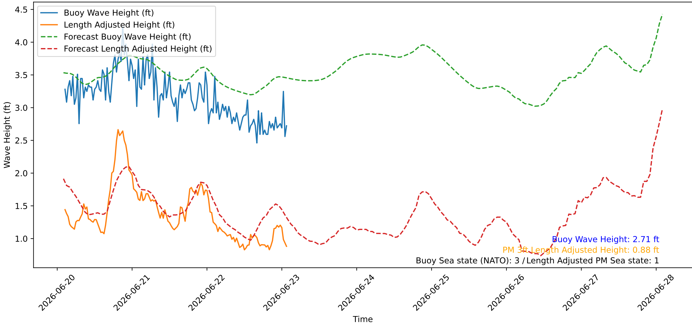
Wave Heights over Time for Green Beach at 2026-06-23 02:21:09
