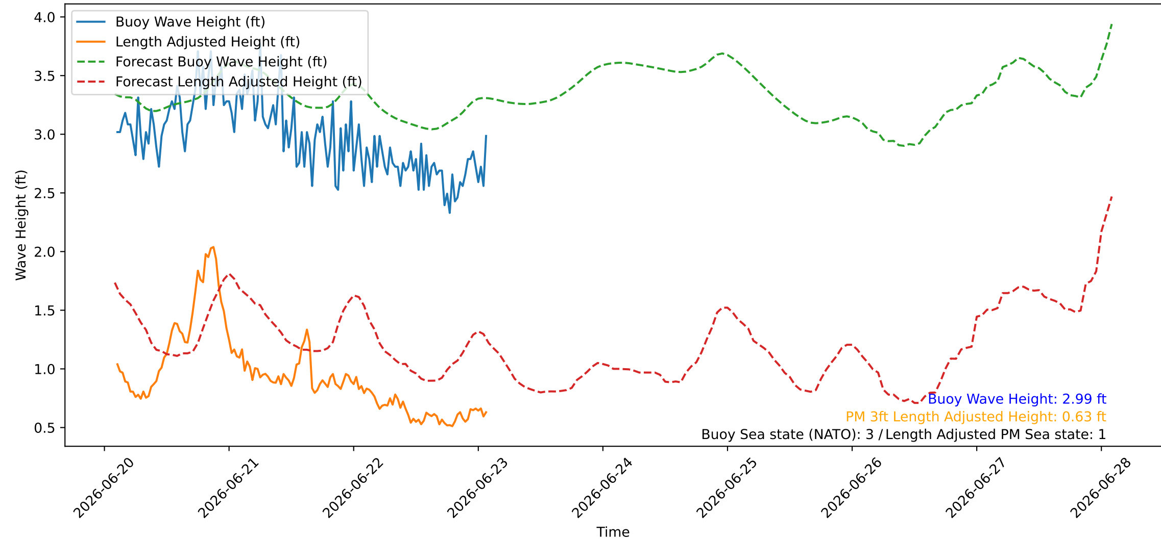
Wave Heights over Time for Red Beach at 2026-06-23 02:20:46
