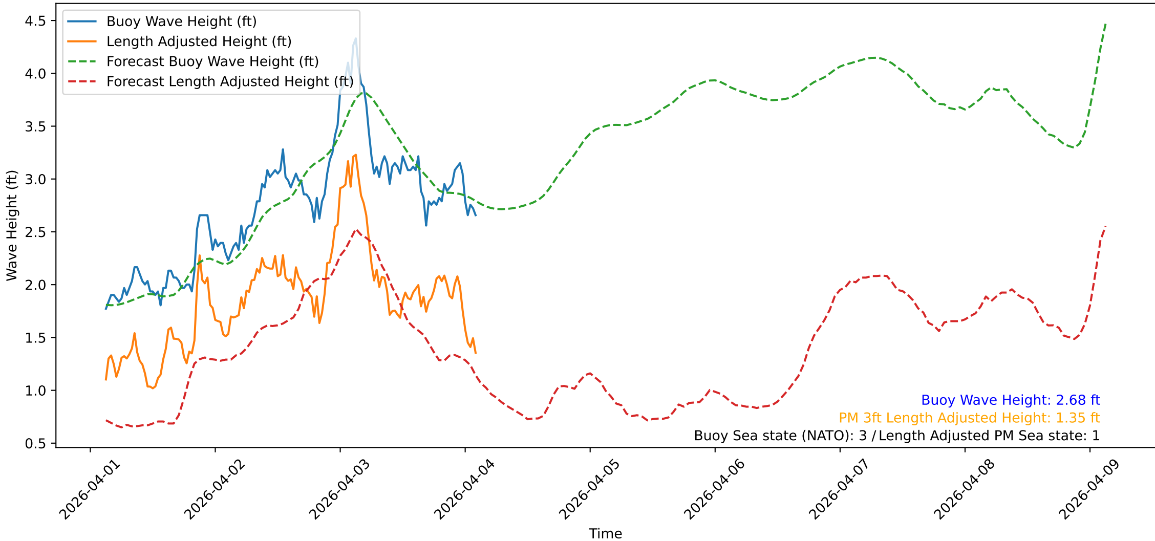
Wave Heights over Time for Green Beach at 2026-04-04 02:51:10
