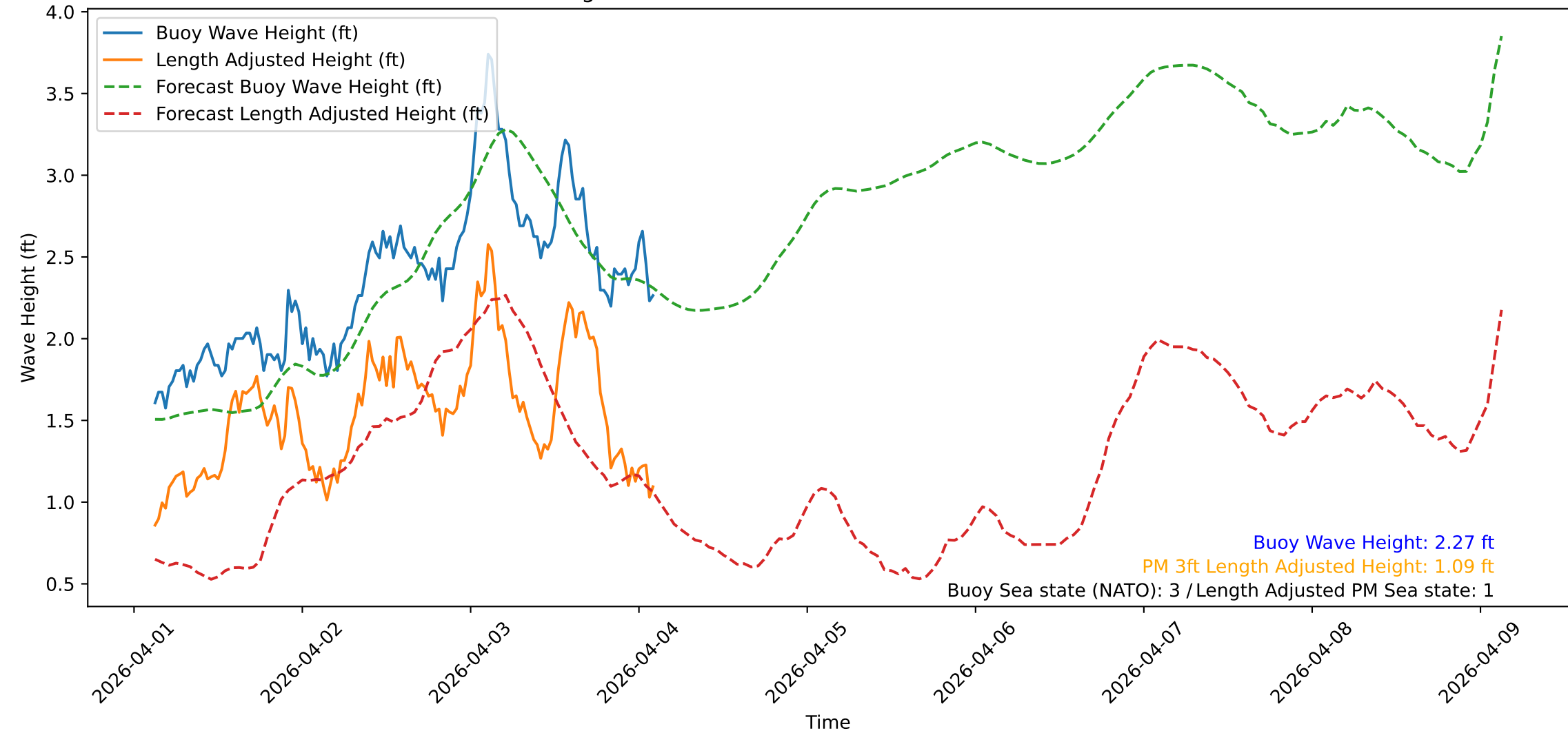
Wave Heights over Time for Red Beach at 2026-04-04 02:50:48
