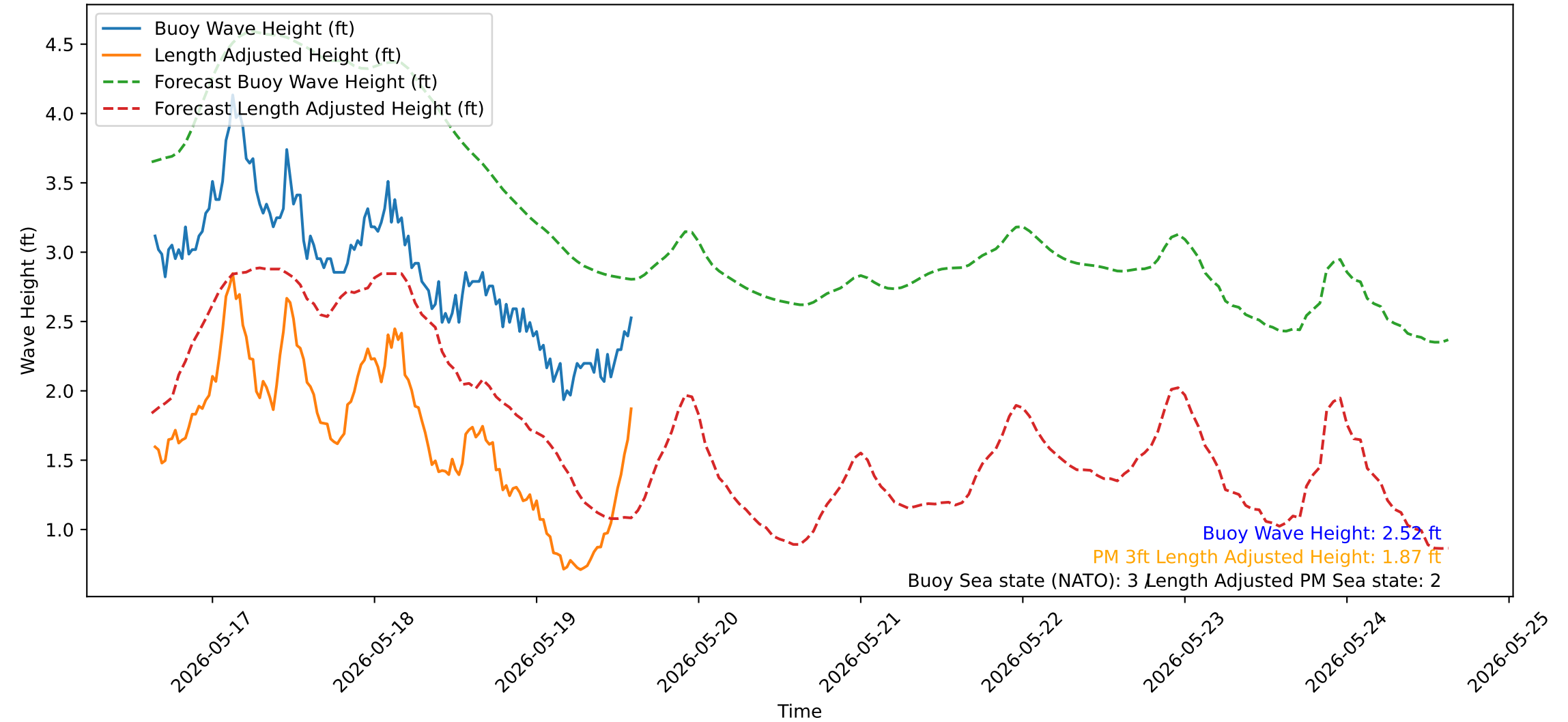
Wave Heights over Time for Red Beach at 2026-05-19 15:10:51
