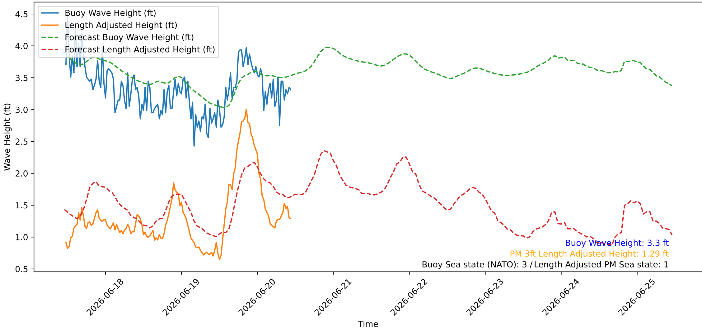
Wave Heights over Time for Green Beach at 2026-06-20 11:21:08
