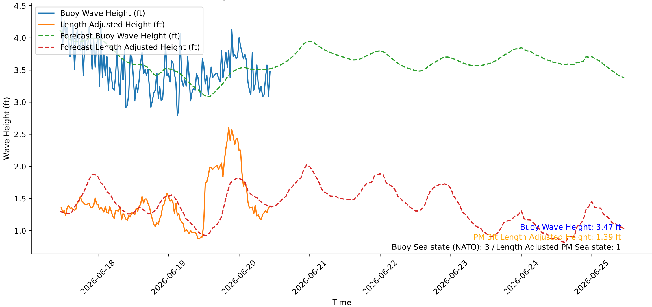
Wave Heights over Time for Oceanside Harbor at 2026-06-20 11:20:25
