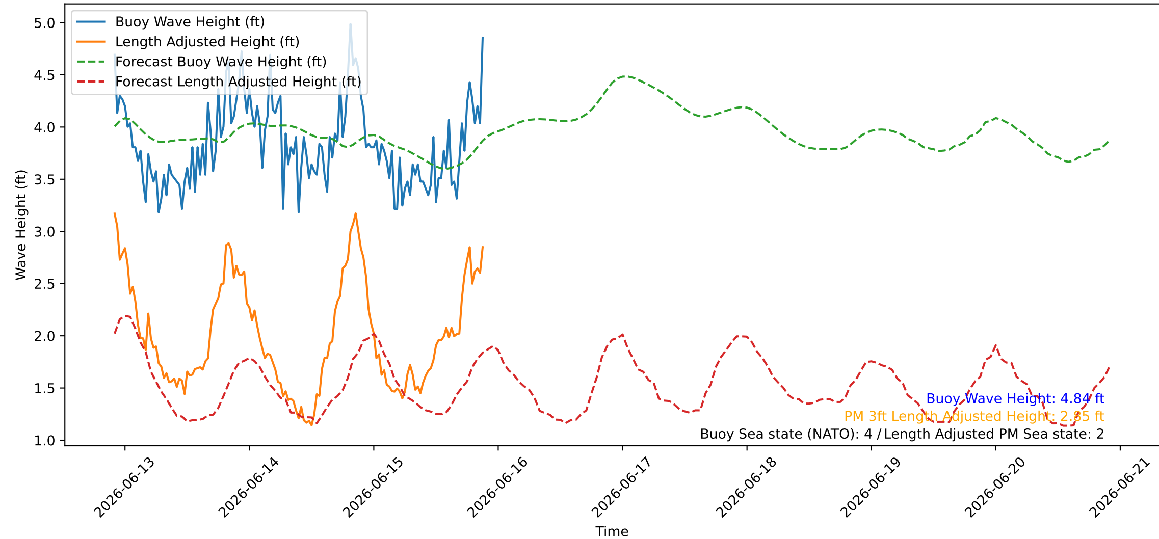
Wave Heights over Time for Oceanside Harbor at 2026-06-15 22:00:25
