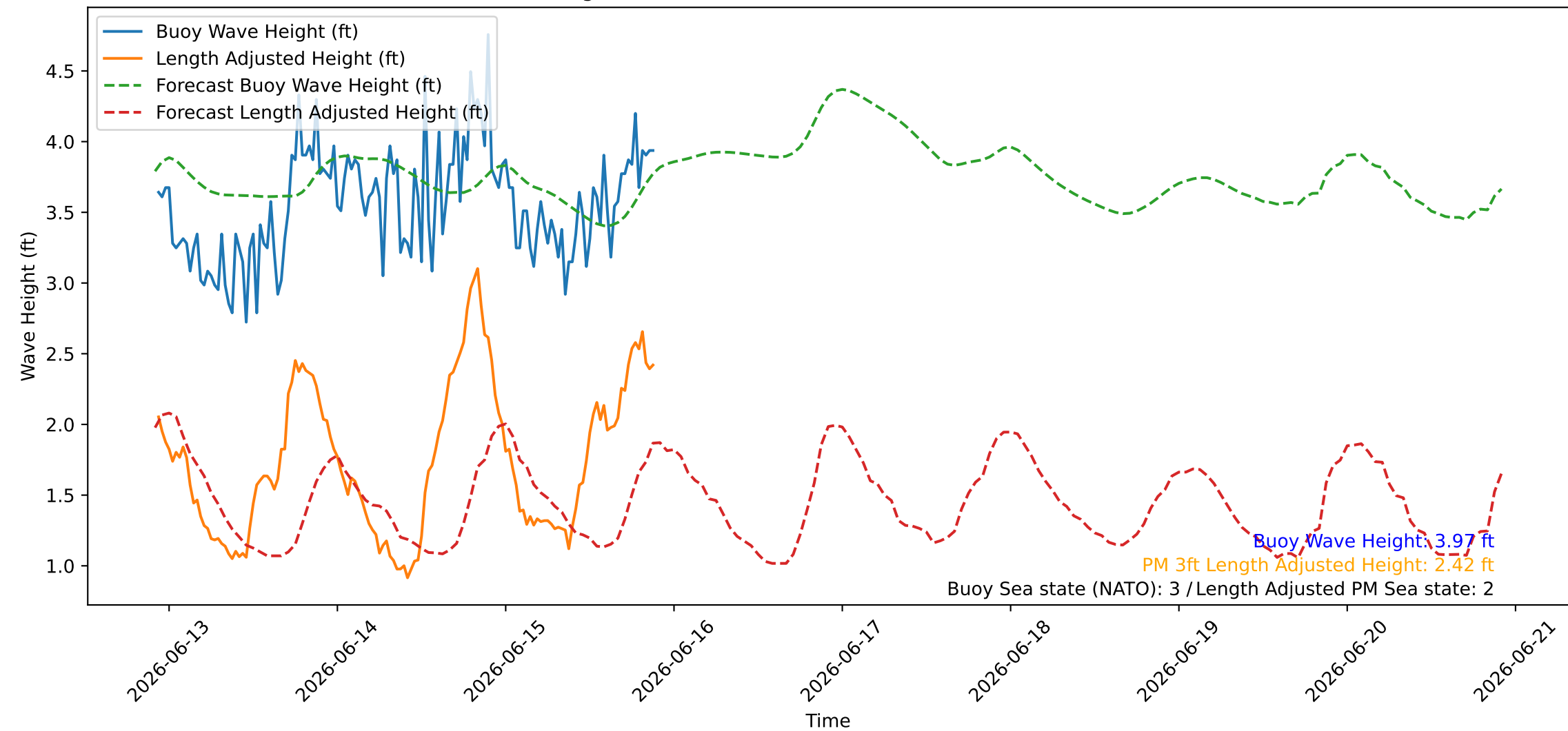
Wave Heights over Time for Red Beach at 2026-06-15 22:00:45
