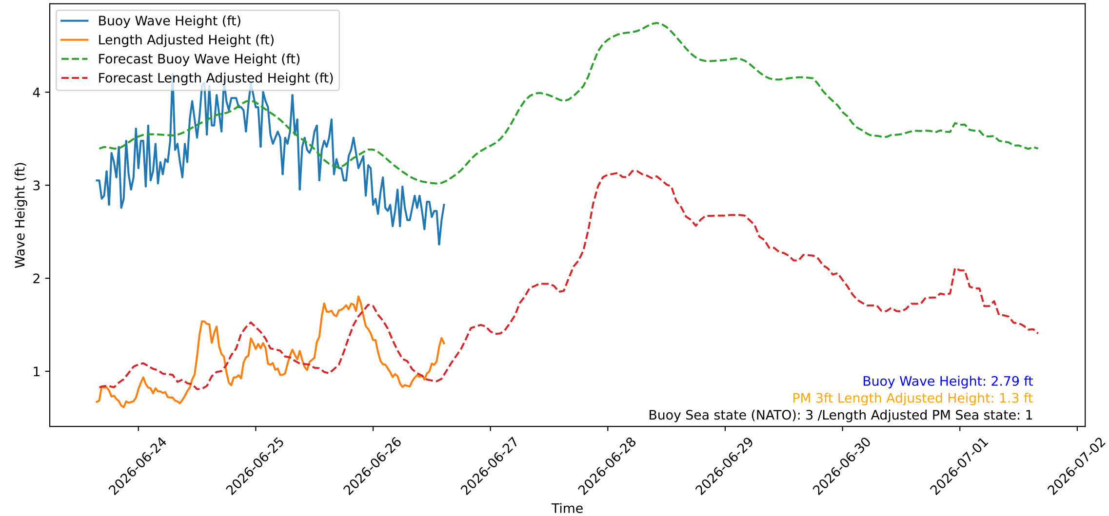
Wave Heights over Time for Green Beach at 2026-06-26 15:31:09
