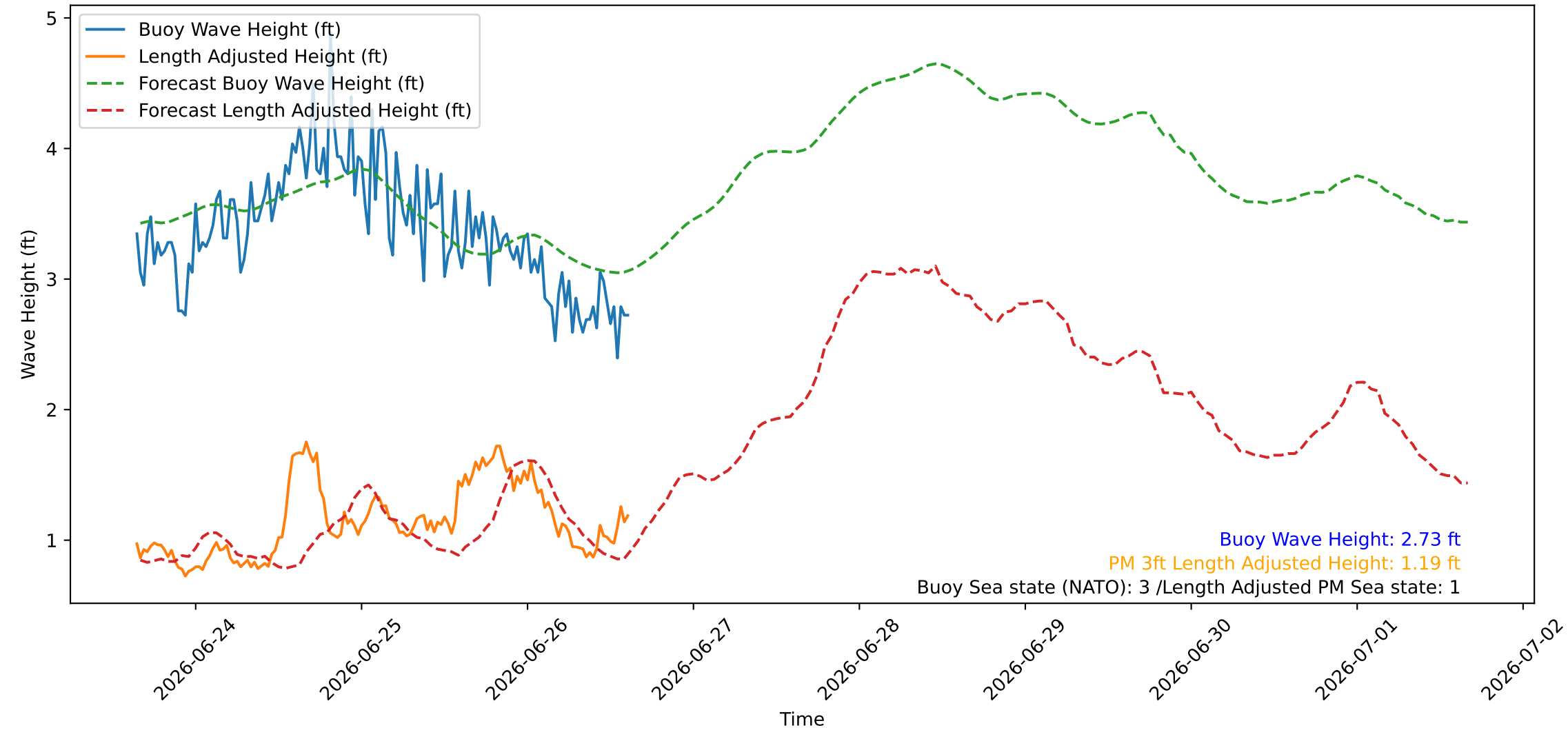
Wave Heights over Time for Oceanside Harbor at 2026-06-26 15:30:27
