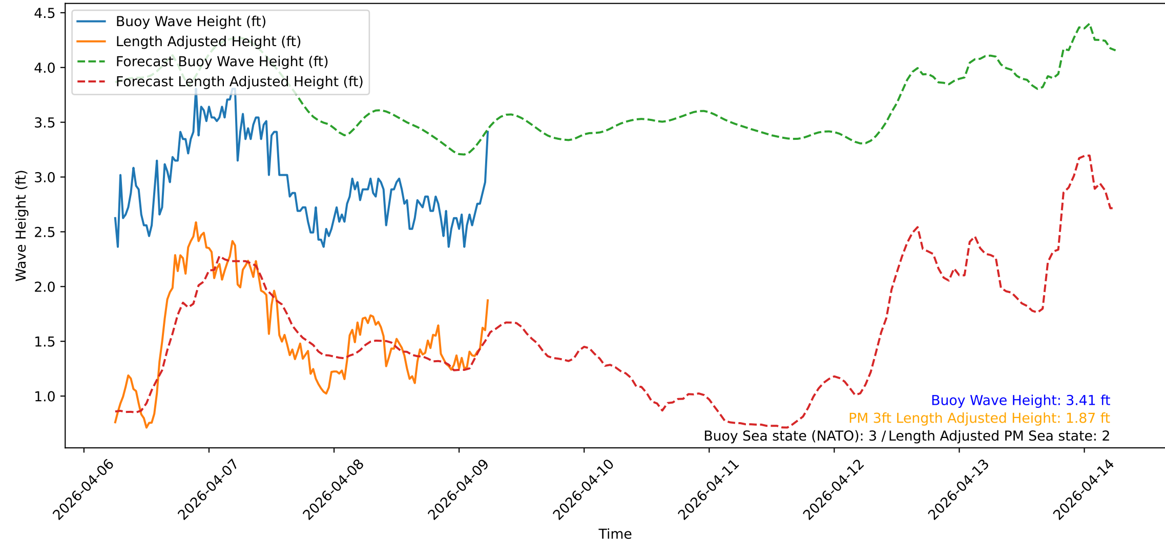
Wave Heights over Time for Green Beach at 2026-04-09 06:11:13
