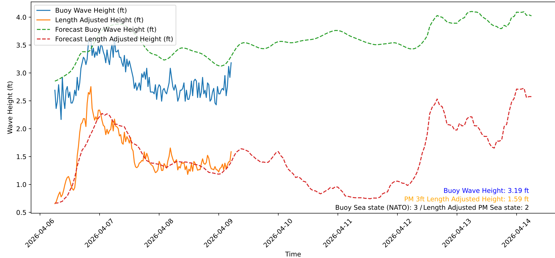
Wave Heights over Time for Oceanside Harbor at 2026-04-09 06:10:33
