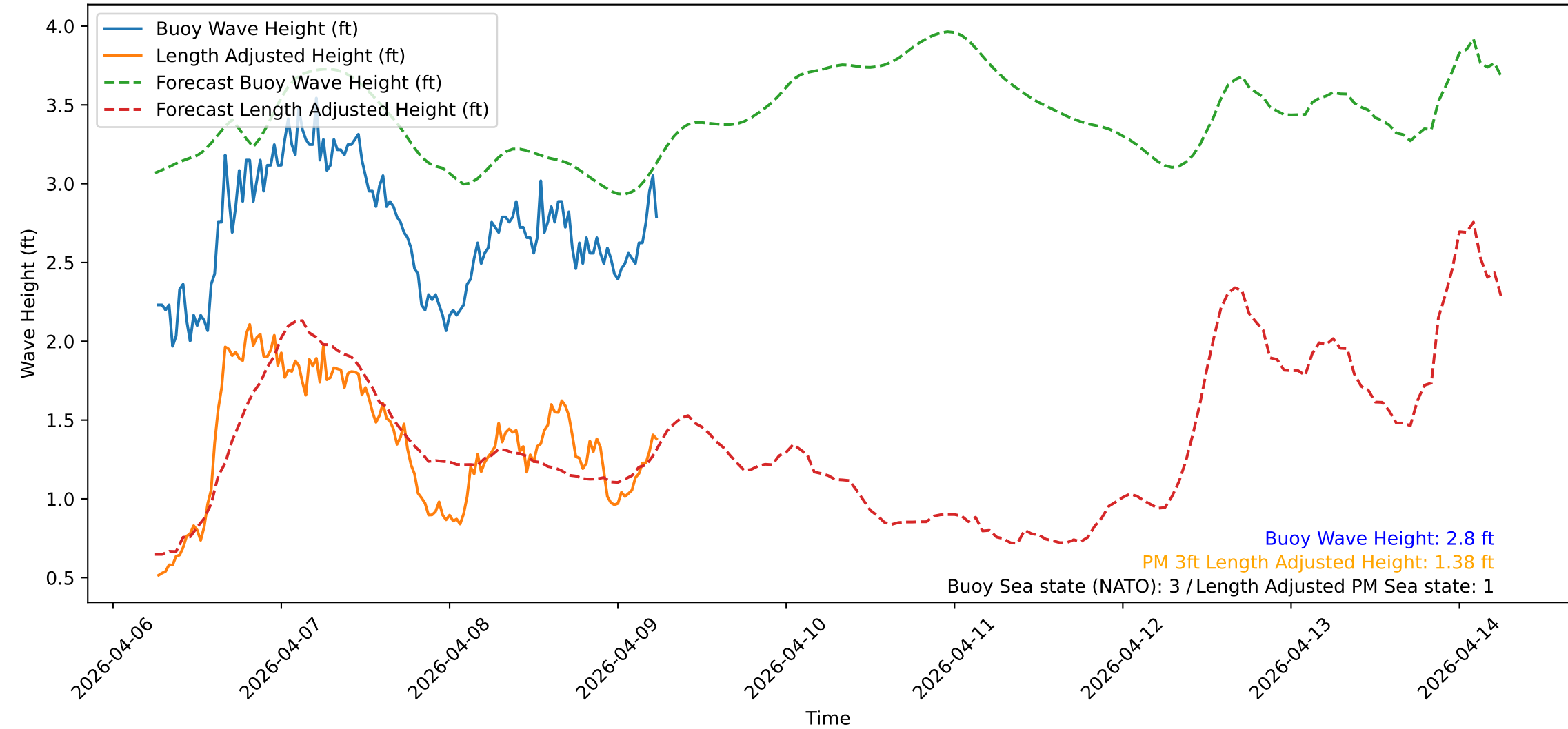
Wave Heights over Time for Red Beach at 2026-04-09 06:10:49
