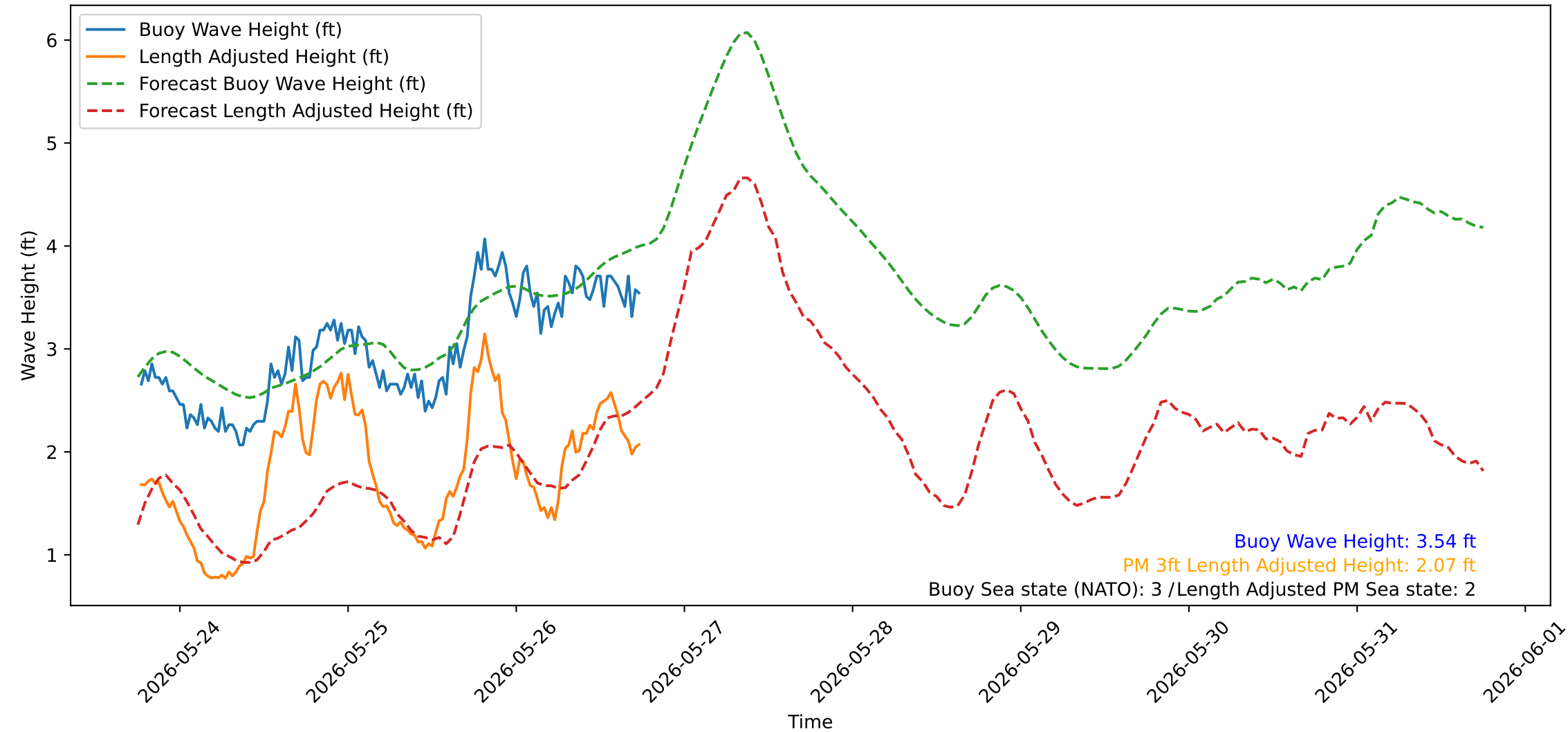
Wave Heights over Time for Green Beach at 2026-05-26 18:21:10
