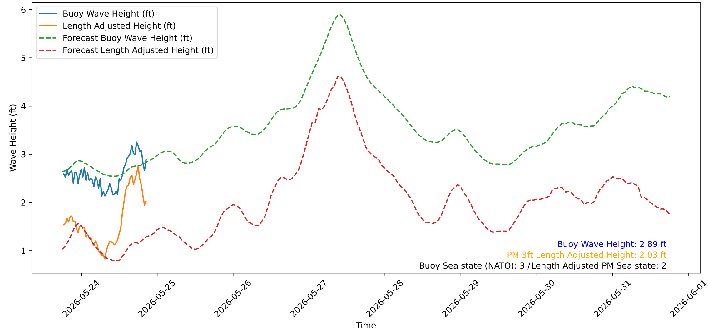
Wave Heights over Time for Oceanside Harbor at 2026-05-26 18:20:26
