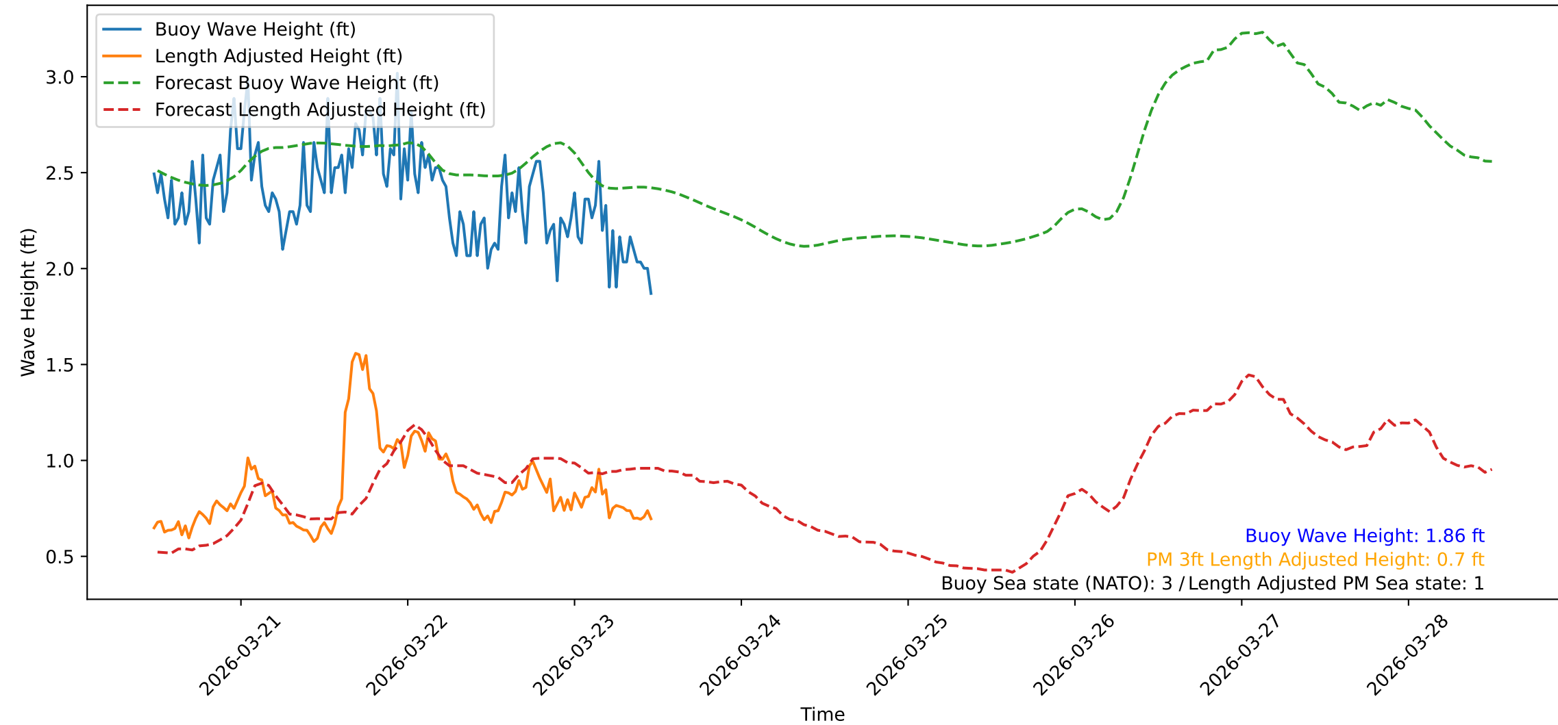
Wave Heights over Time for Oceanside Harbor at 2026-03-23 11:40:31
