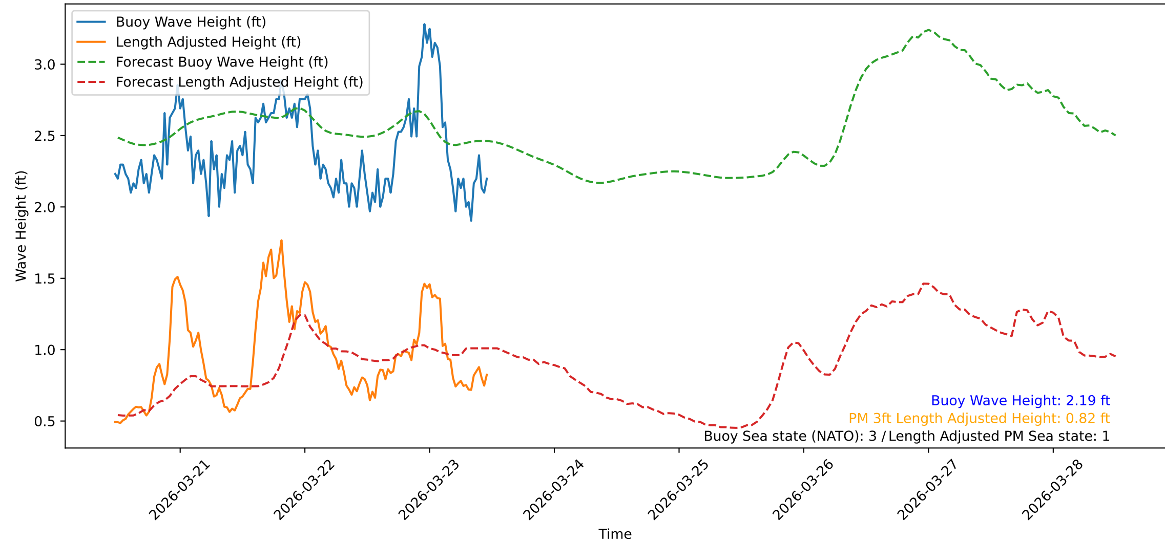
Wave Heights over Time for Green Beach at 2026-03-23 11:41:10
