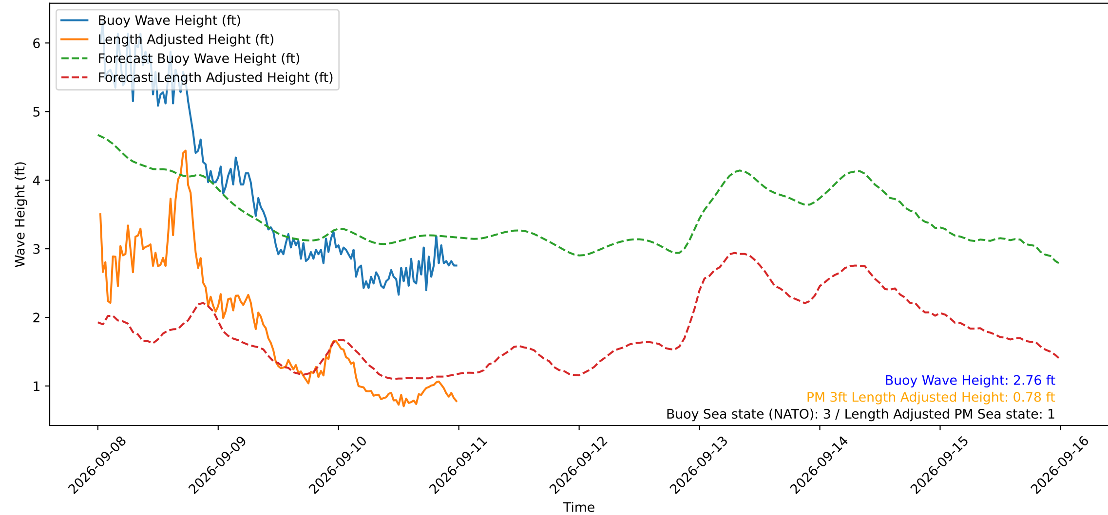
Wave Heights over Time for Red Beach at 2026-09-11 00:20:50
