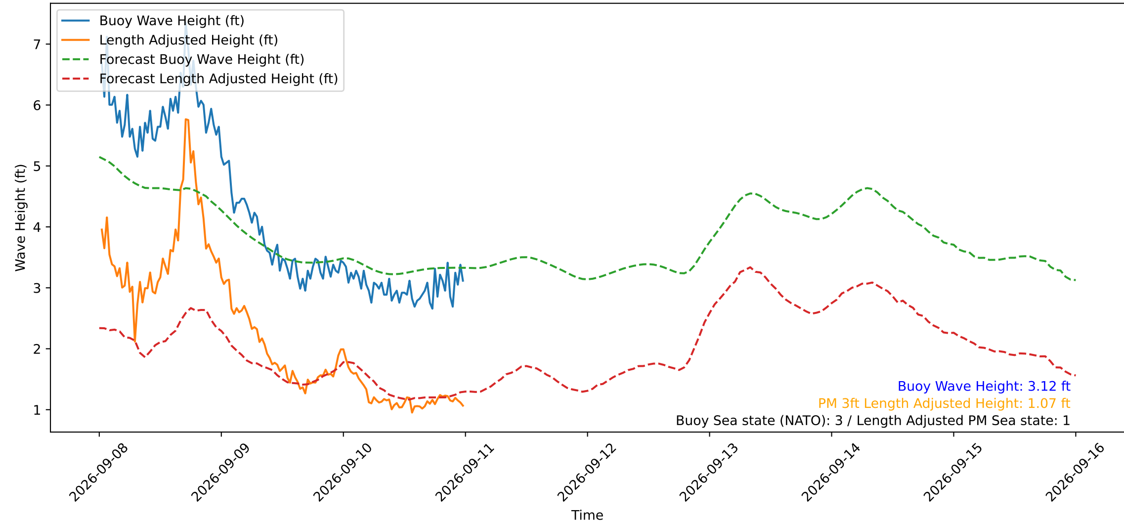
Wave Heights over Time for Oceanside Harbor at 2026-09-11 00:20:29
