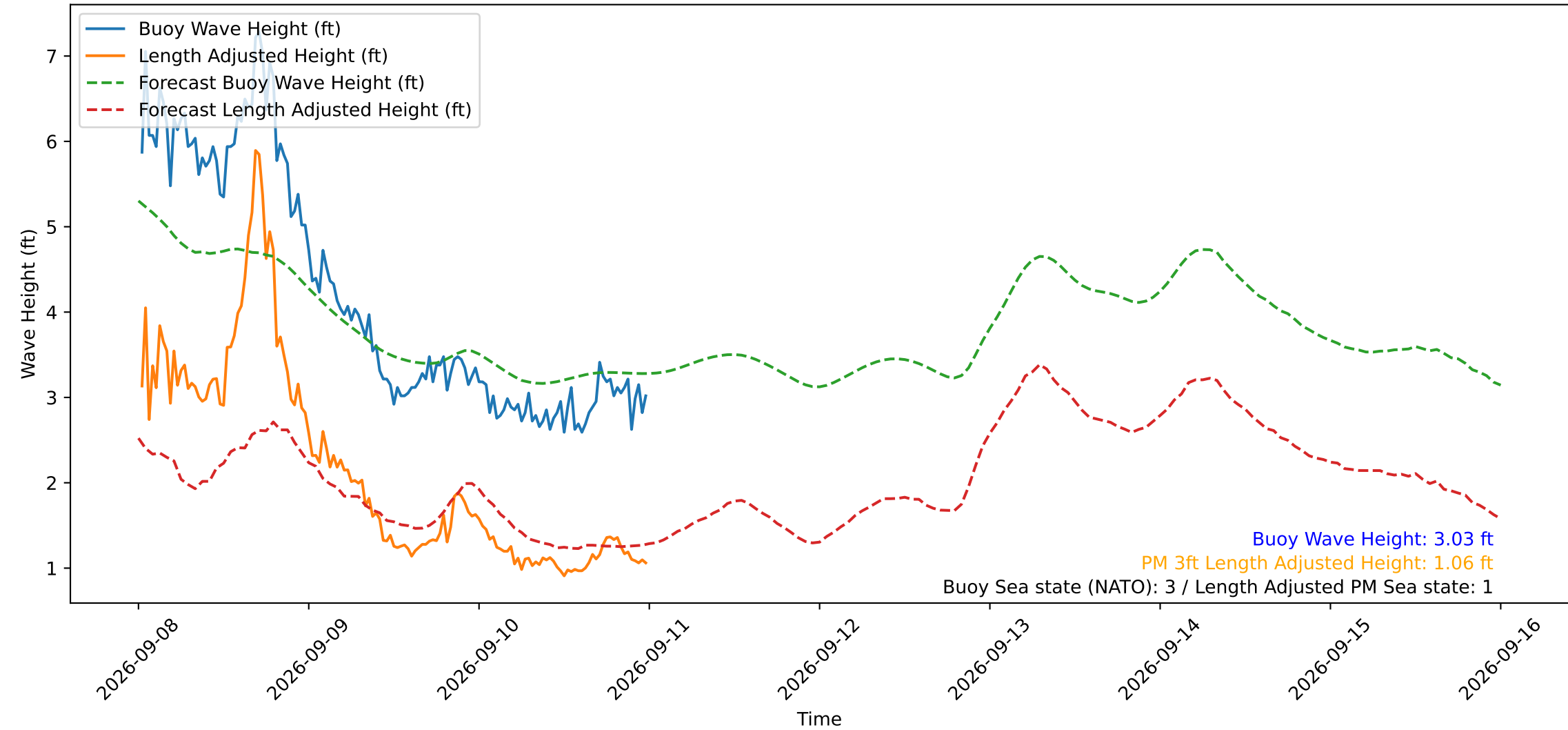
Wave Heights over Time for Green Beach at 2026-09-11 00:21:14
