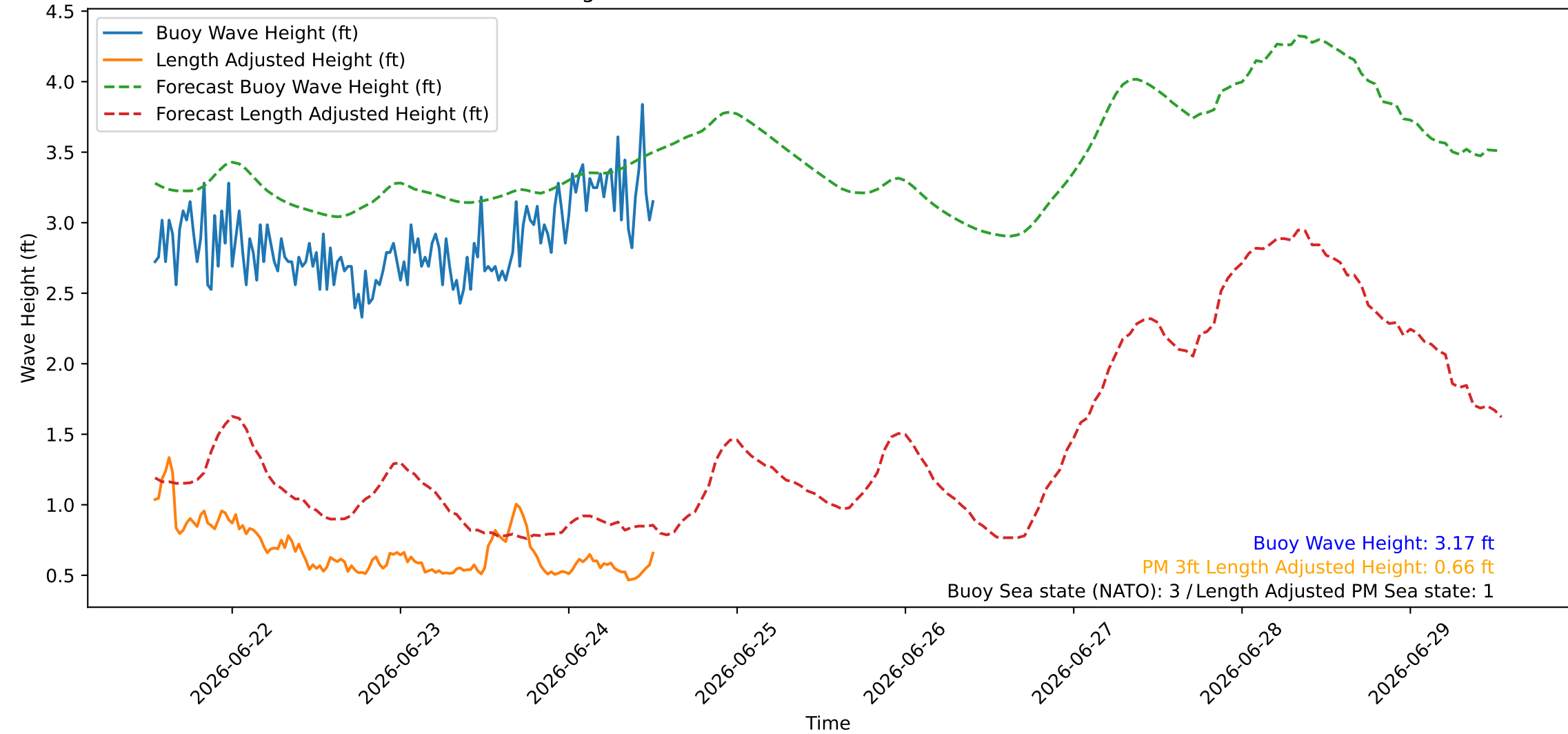
Wave Heights over Time for Red Beach at 2026-06-24 12:40:45
