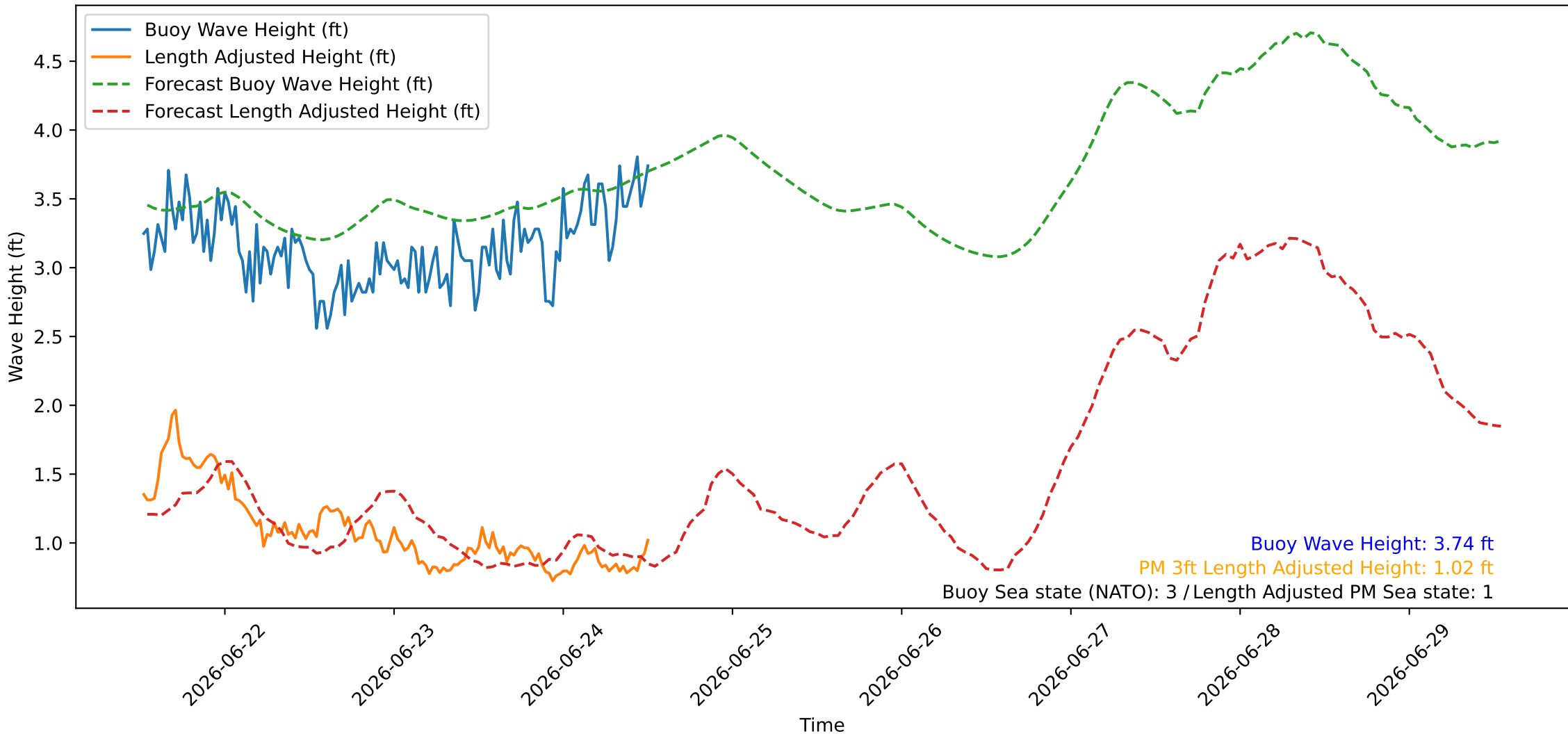
Wave Heights over Time for Oceanside Harbor at 2026-06-24 12:40:26
