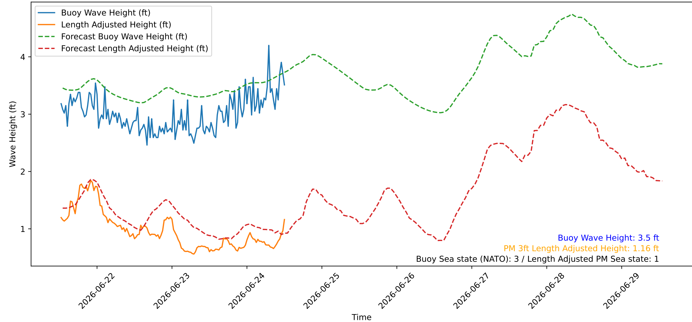
Wave Heights over Time for Green Beach at 2026-06-24 12:41:08
