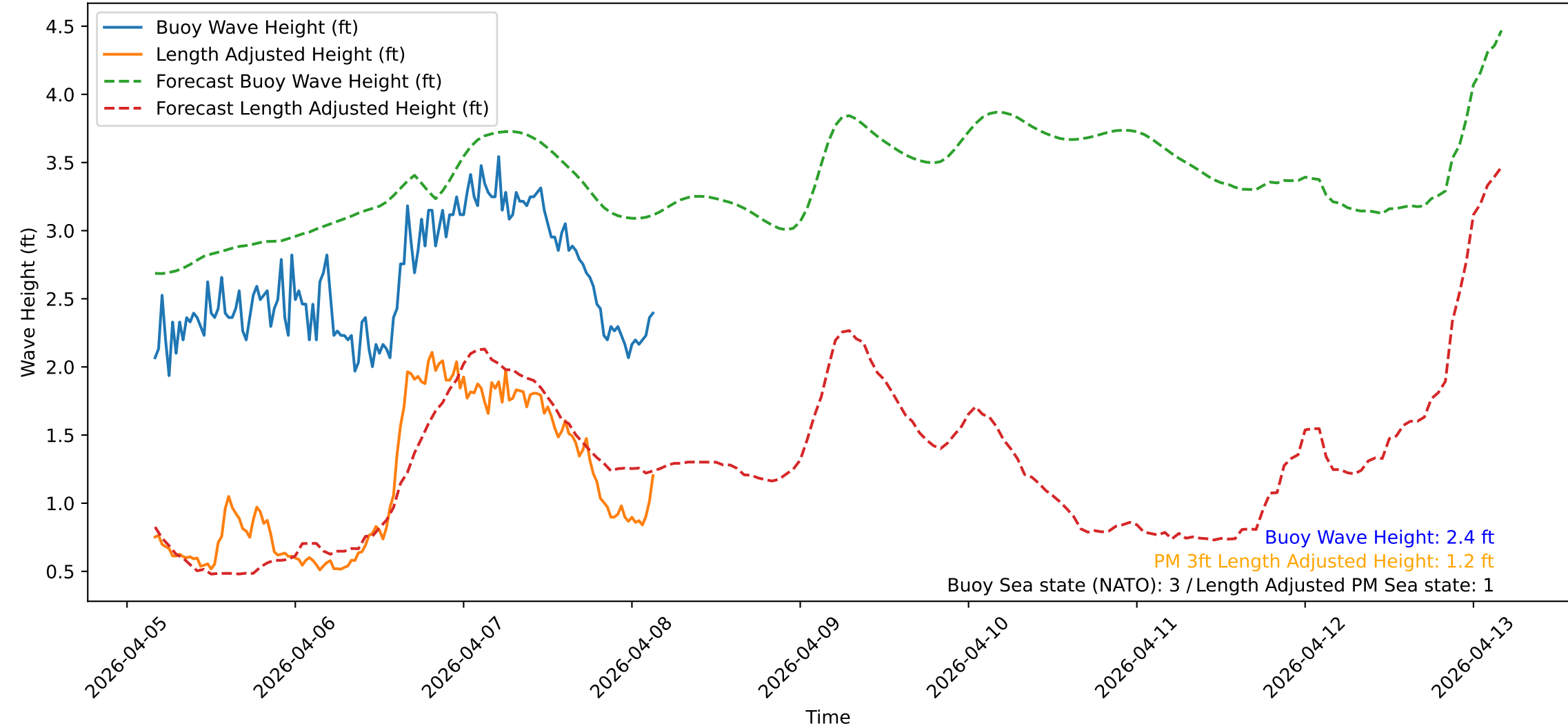
Wave Heights over Time for Red Beach at 2026-04-08 03:40:47
