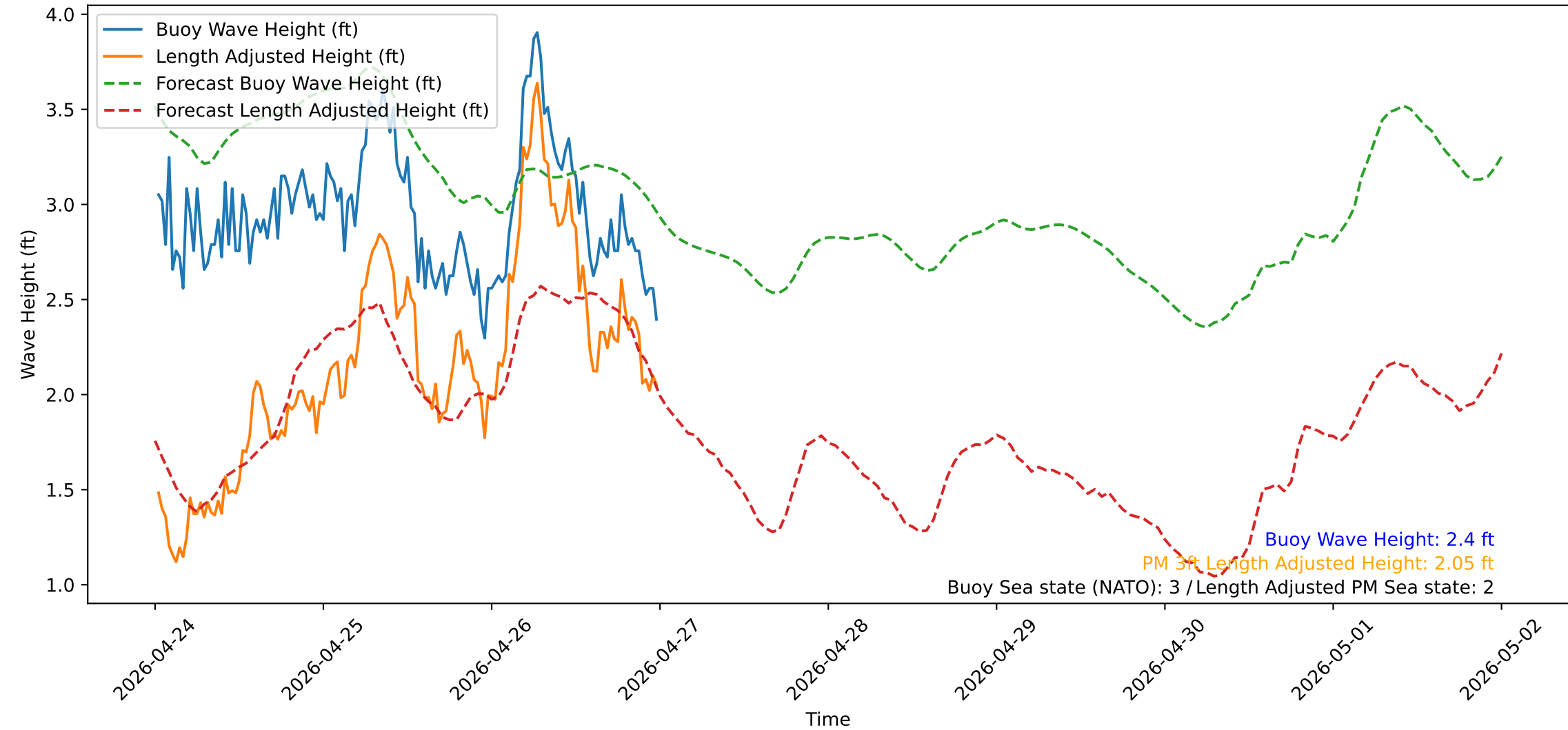
Wave Heights over Time for Oceanside Harbor at 2026-04-27 00:20:32
