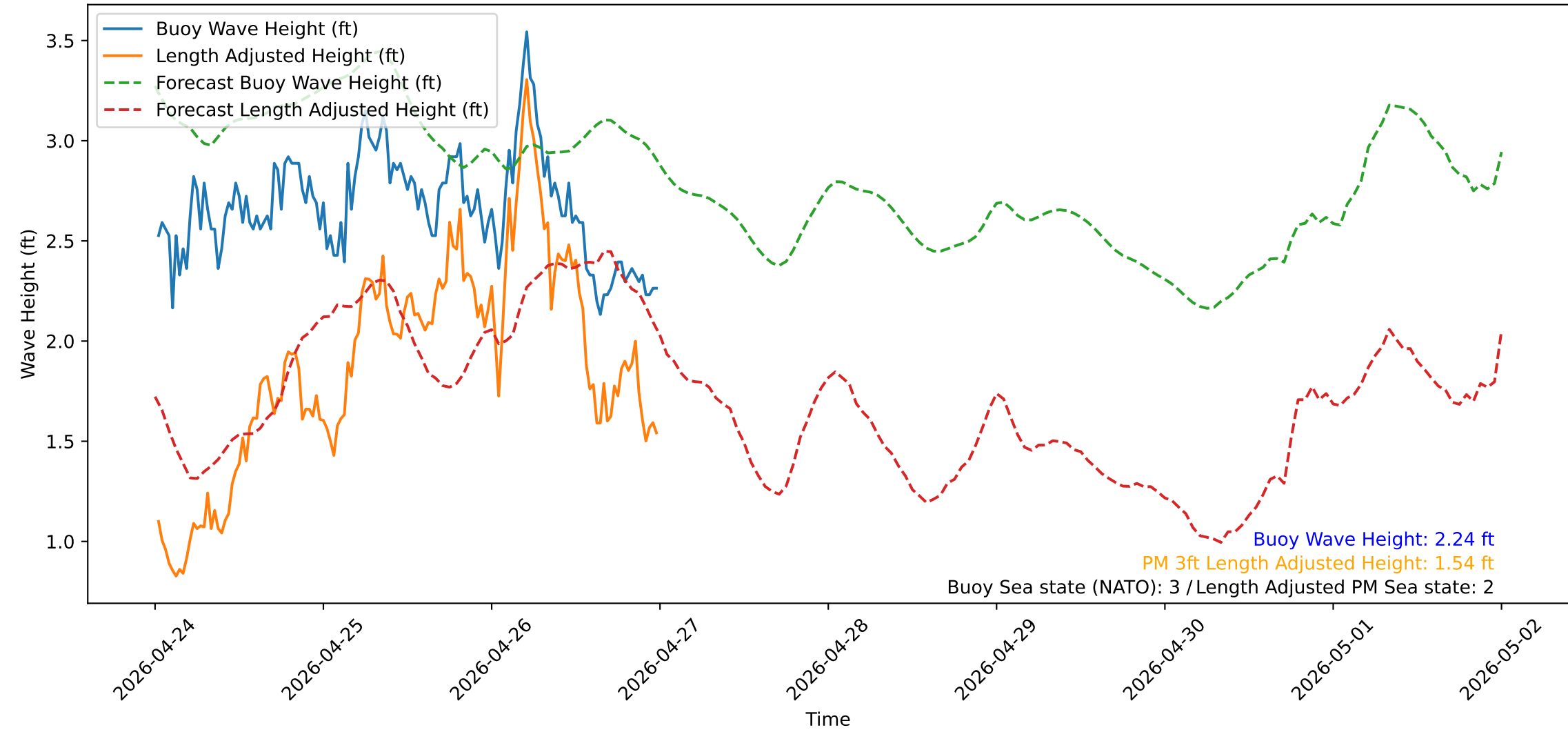
Wave Heights over Time for Red Beach at 2026-04-27 00:20:52
