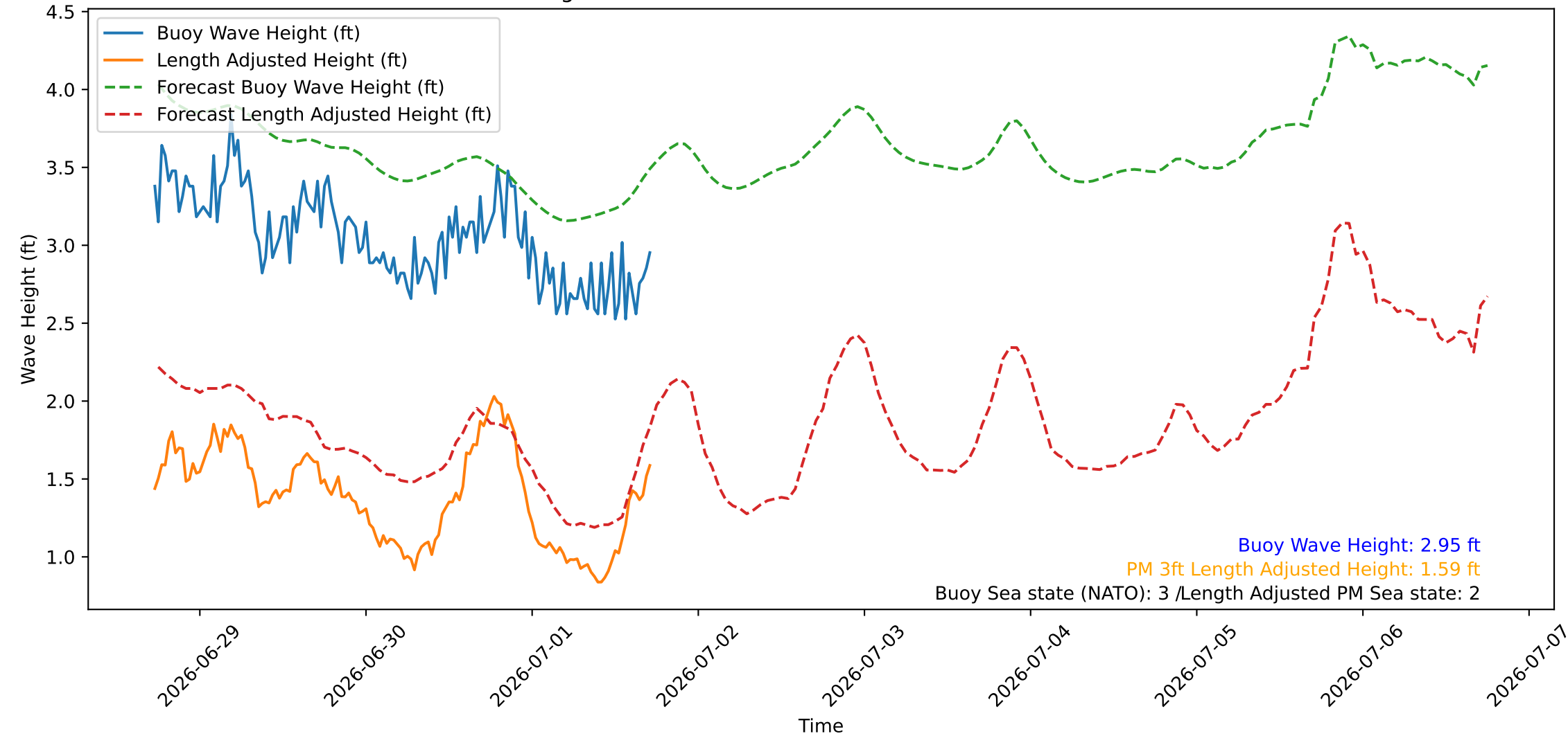
Wave Heights over Time for Green Beach at 2026-07-01 17:41:08
