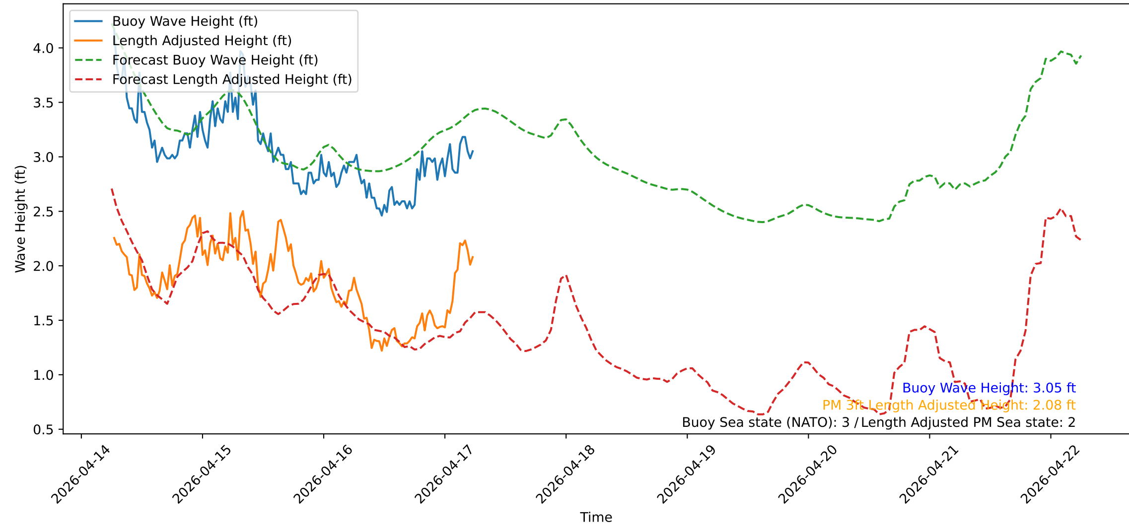
Wave Heights over Time for Green Beach at 2026-04-17 06:21:16
