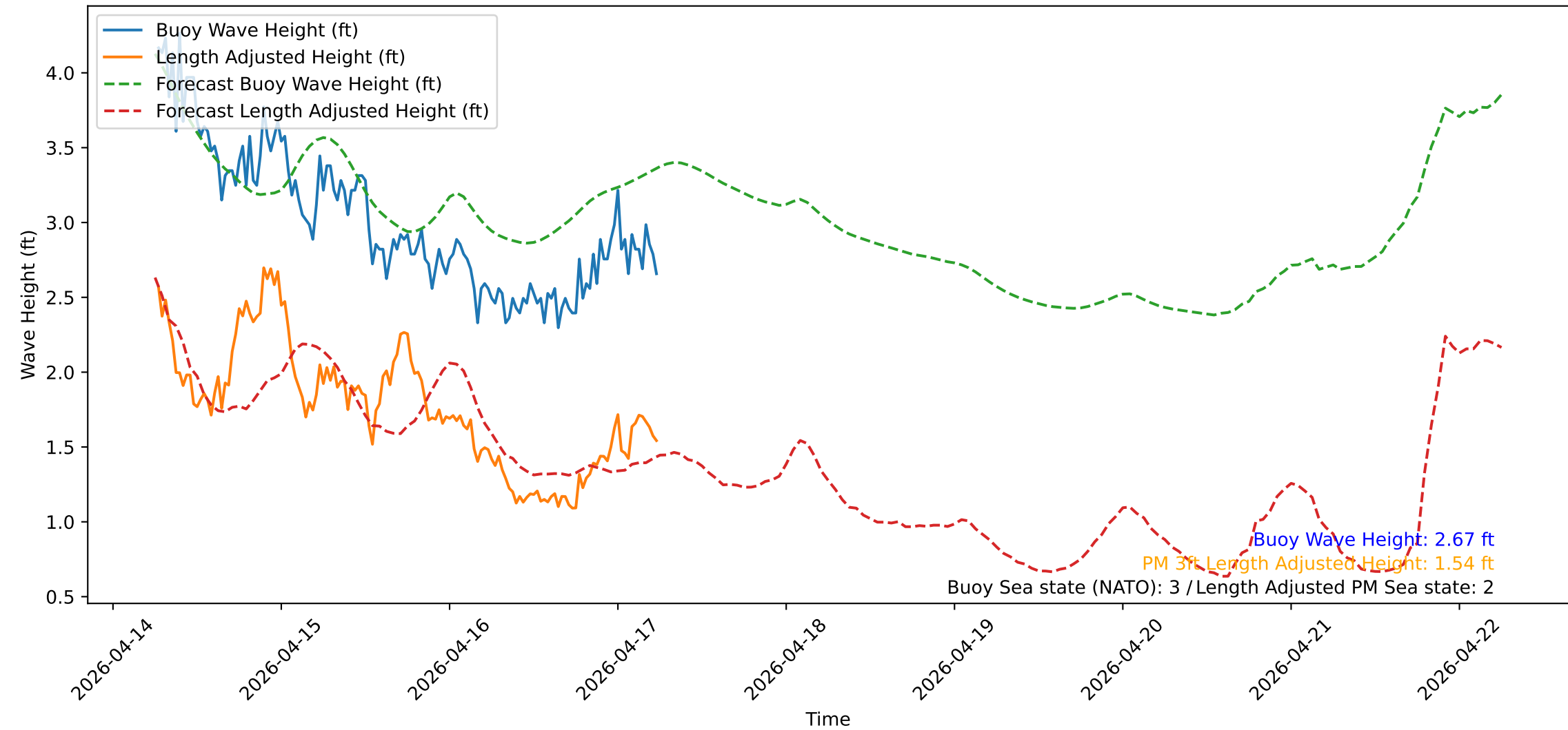
Wave Heights over Time for Oceanside Harbor at 2026-04-17 06:20:31
