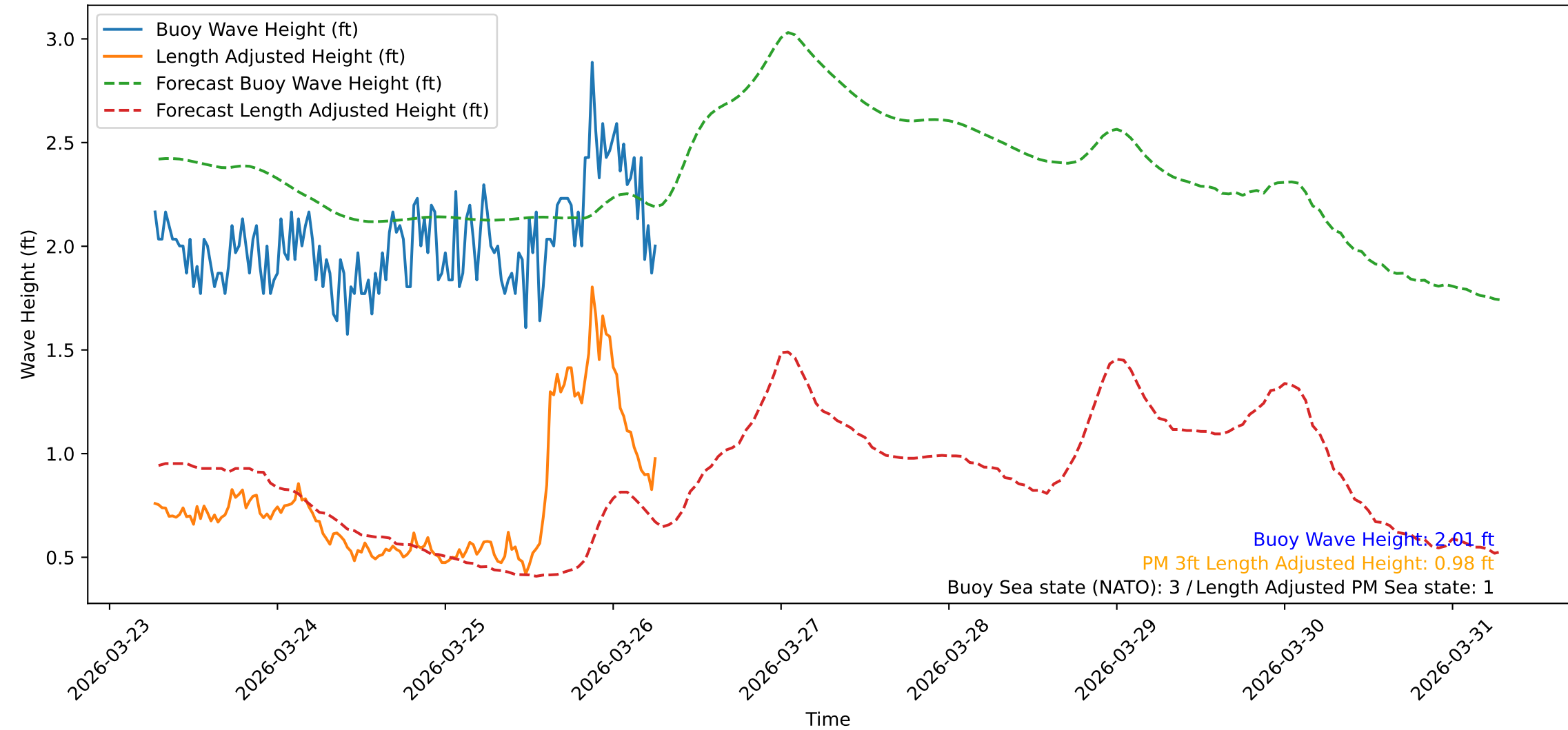
Wave Heights over Time for Oceanside Harbor at 2026-03-26 06:30:32
