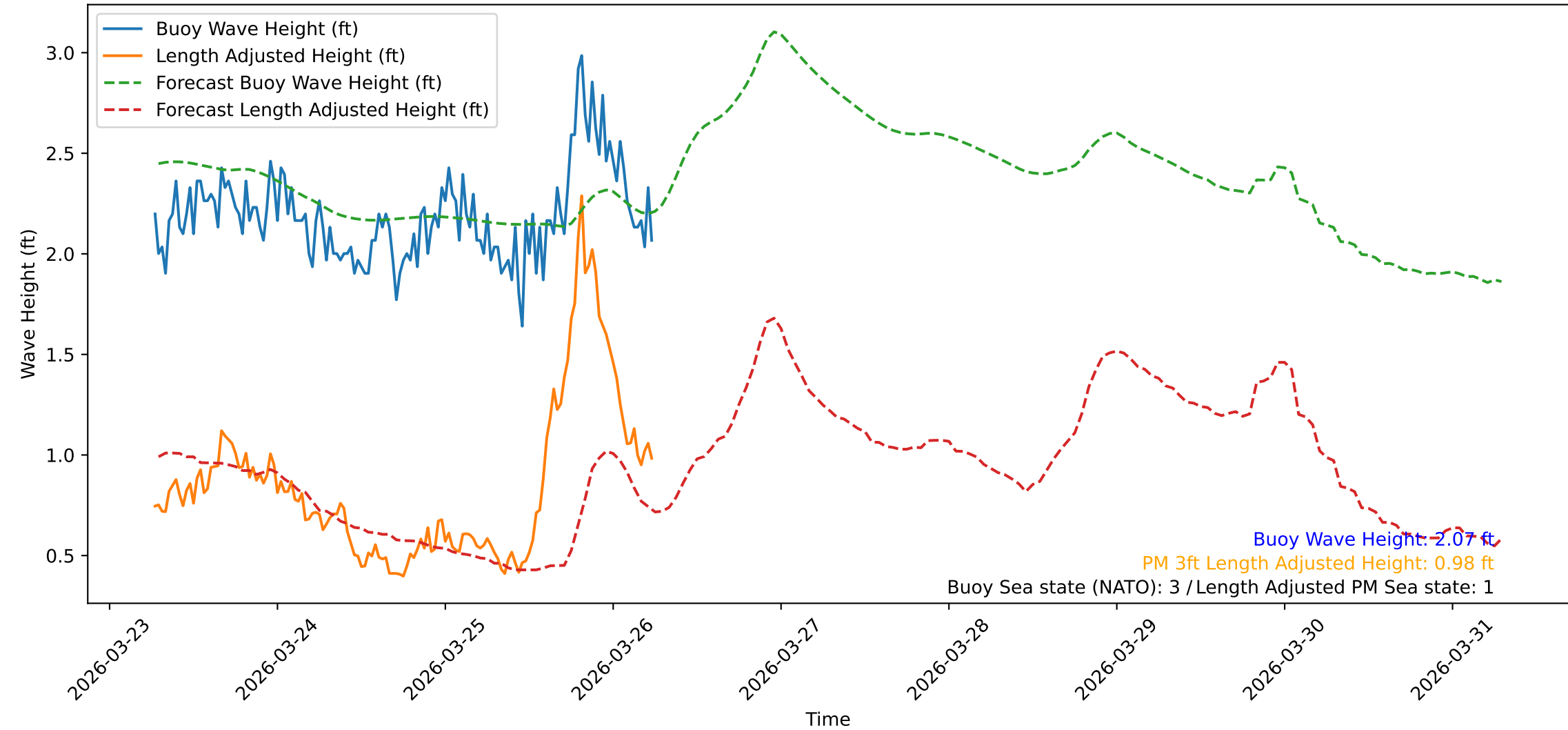
Wave Heights over Time for Green Beach at 2026-03-26 06:31:10
