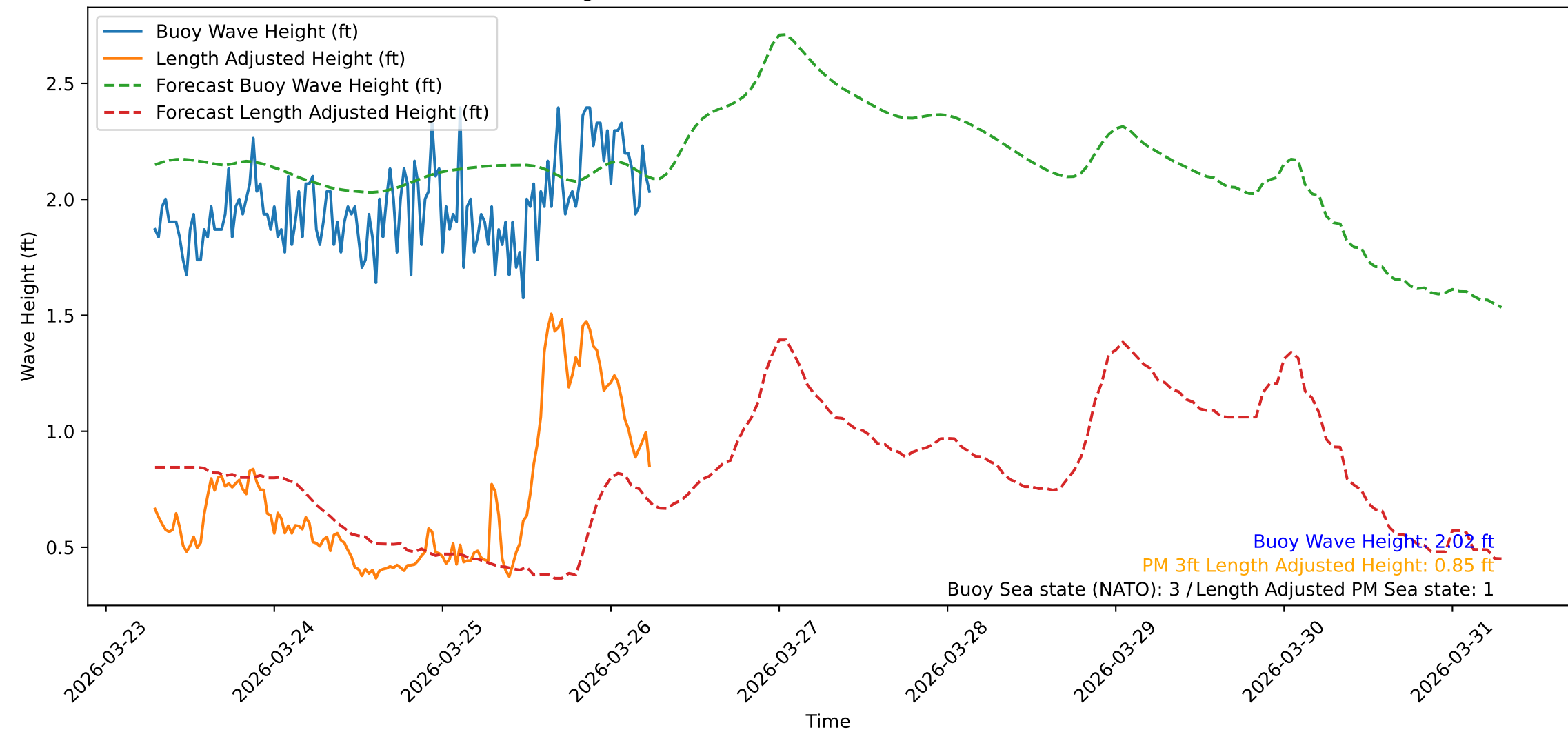
Wave Heights over Time for Red Beach at 2026-03-26 06:30:48
