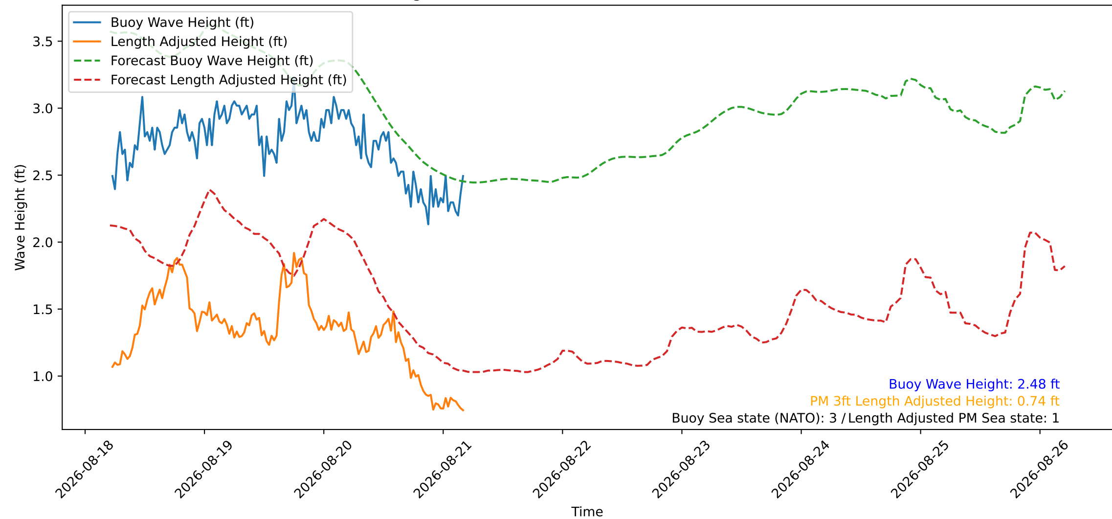
Wave Heights over Time for Red Beach at 2026-08-21 05:00:45
