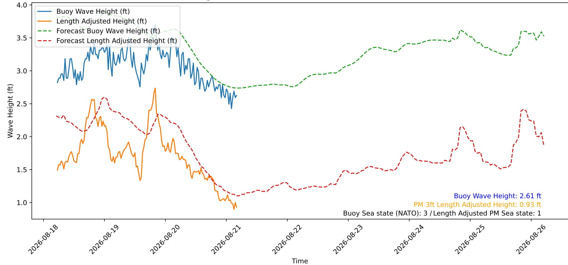
Wave Heights over Time for Green Beach at 2026-08-21 05:01:07
