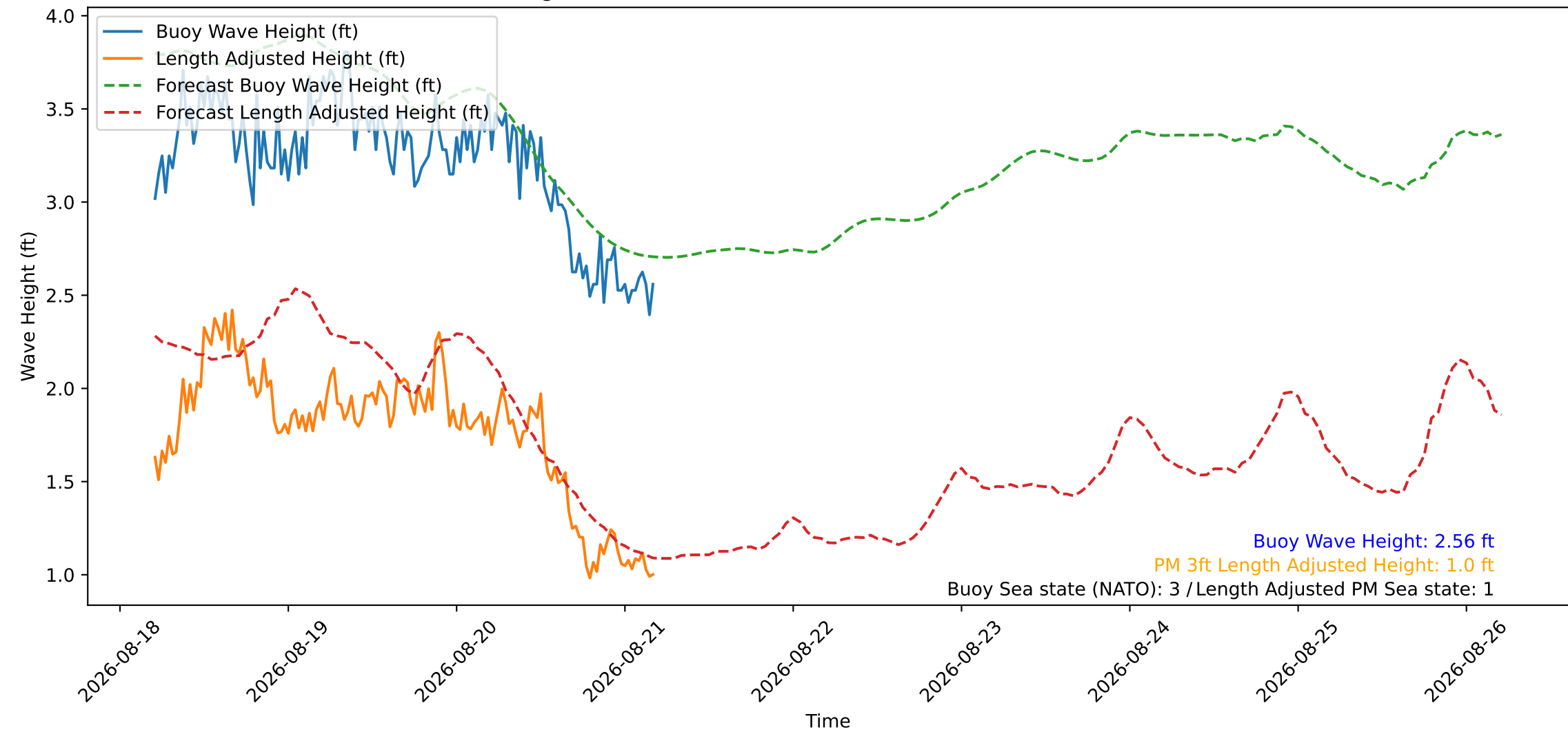
Wave Heights over Time for Oceanside Harbor at 2026-08-21 05:00:26
