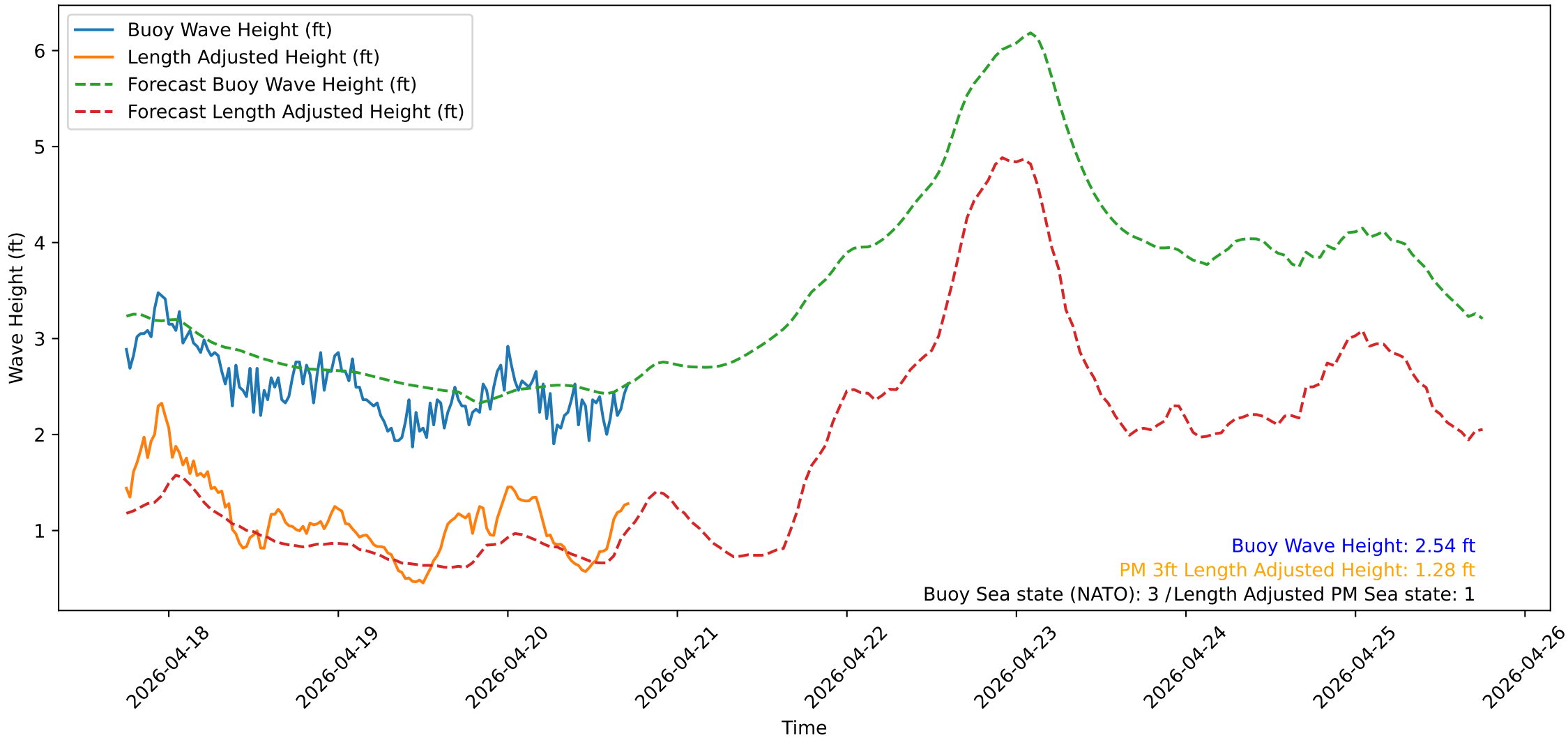
Wave Heights over Time for Green Beach at 2026-04-20 18:01:14
