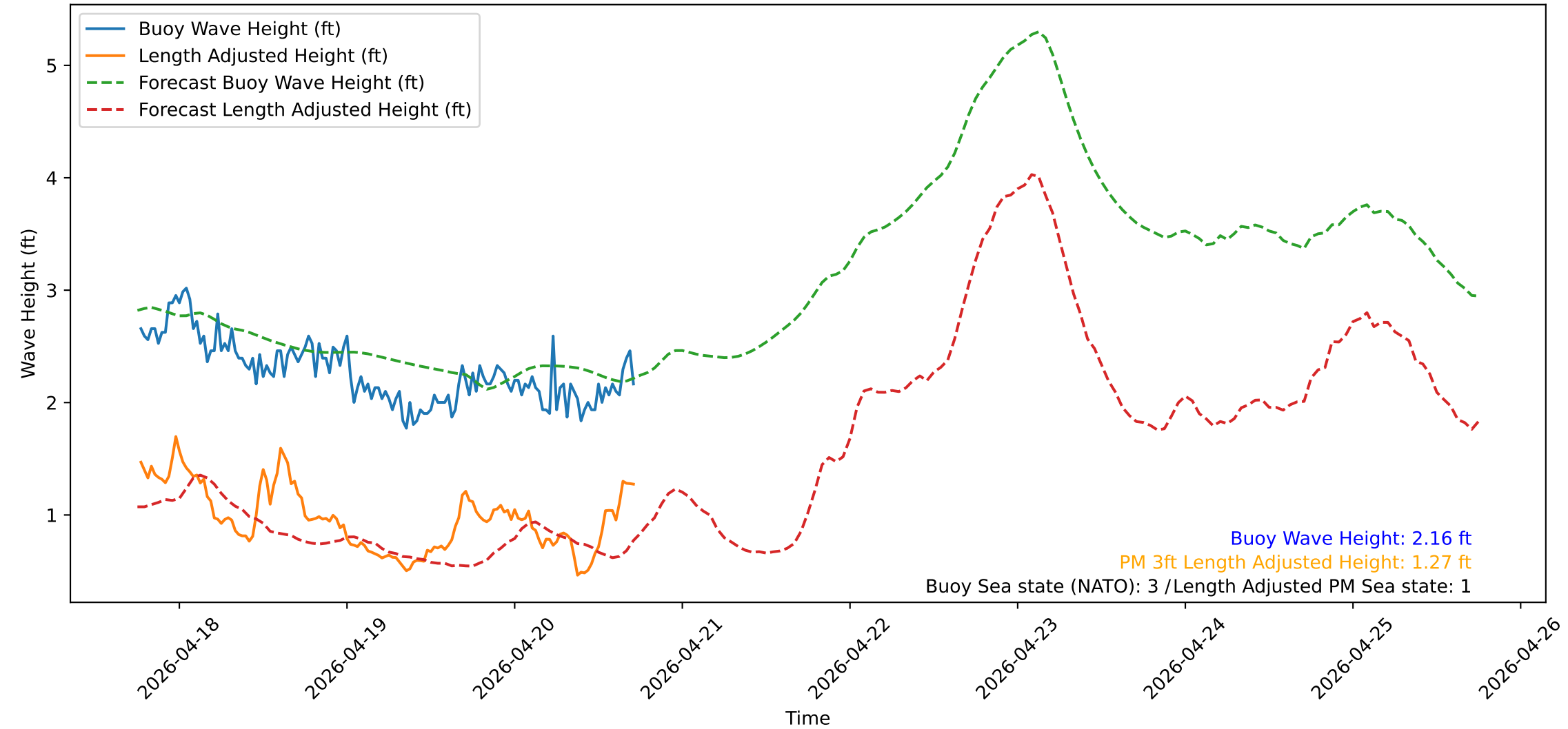
Wave Heights over Time for Red Beach at 2026-04-20 18:00:52
