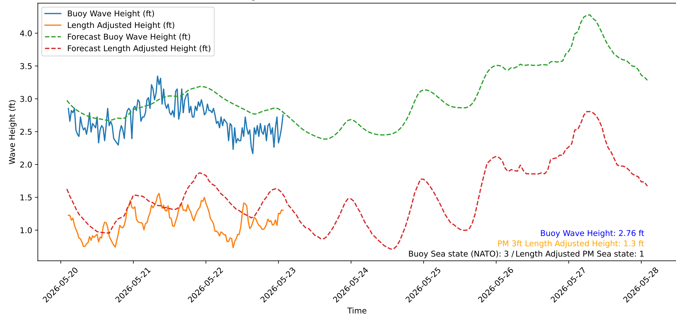
Wave Heights over Time for Red Beach at 2026-05-23 02:10:52
