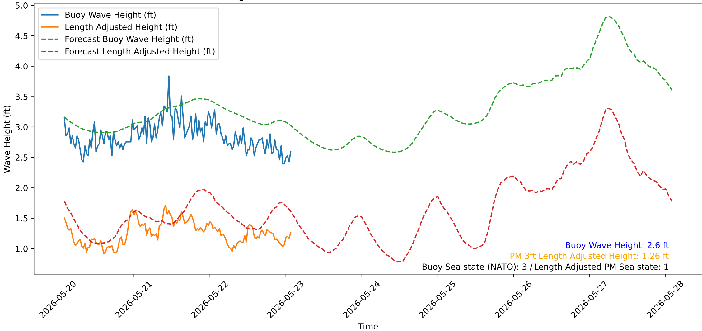
Wave Heights over Time for Oceanside Harbor at 2026-05-23 02:10:32
