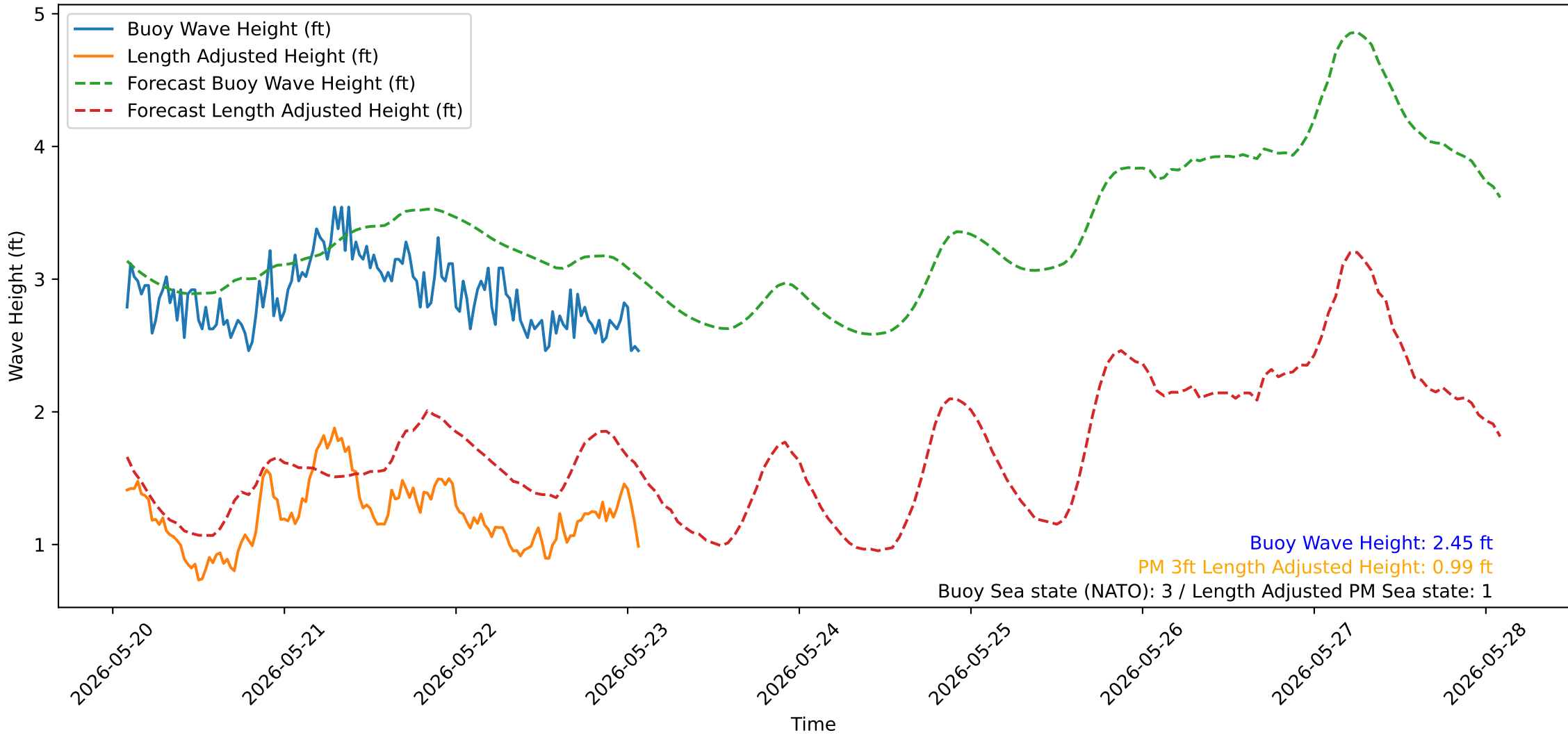
Wave Heights over Time for Green Beach at 2026-05-23 02:11:14
