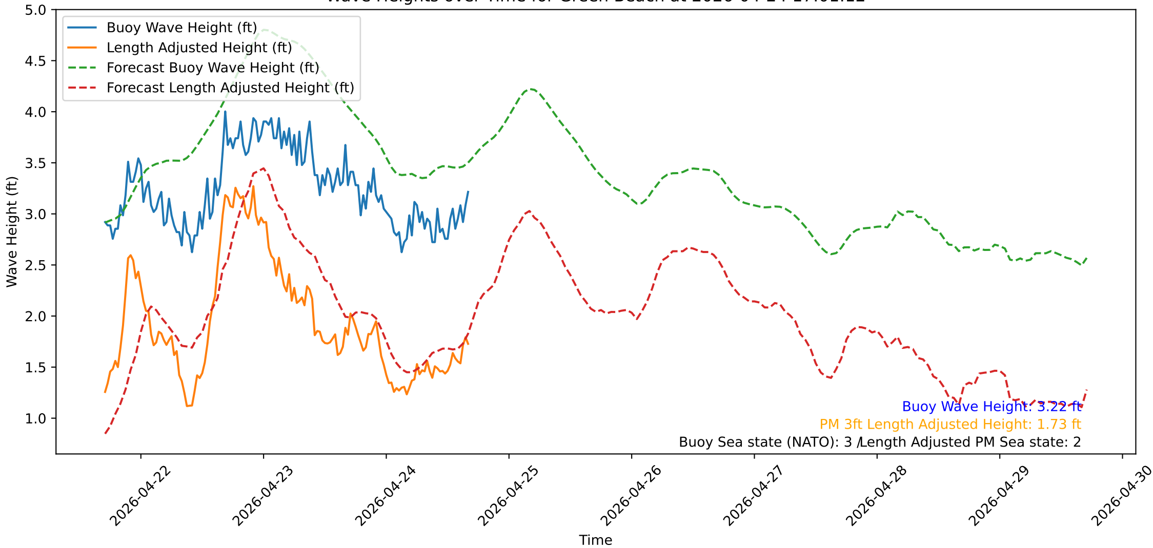
Wave Heights over Time for Green Beach at 2026-04-24 17:01:12
