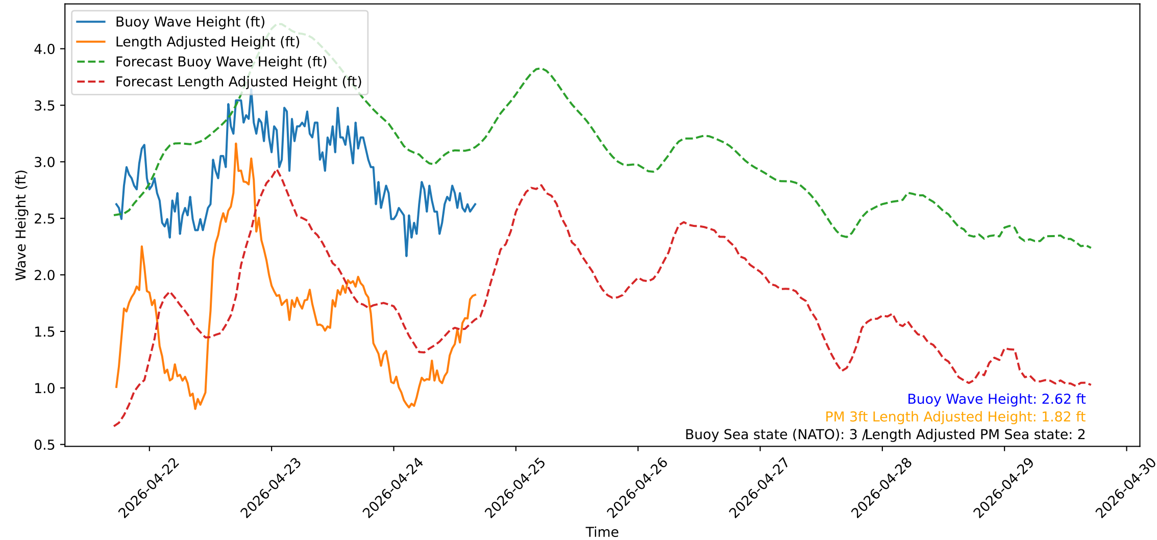
Wave Heights over Time for Red Beach at 2026-04-24 17:00:50
