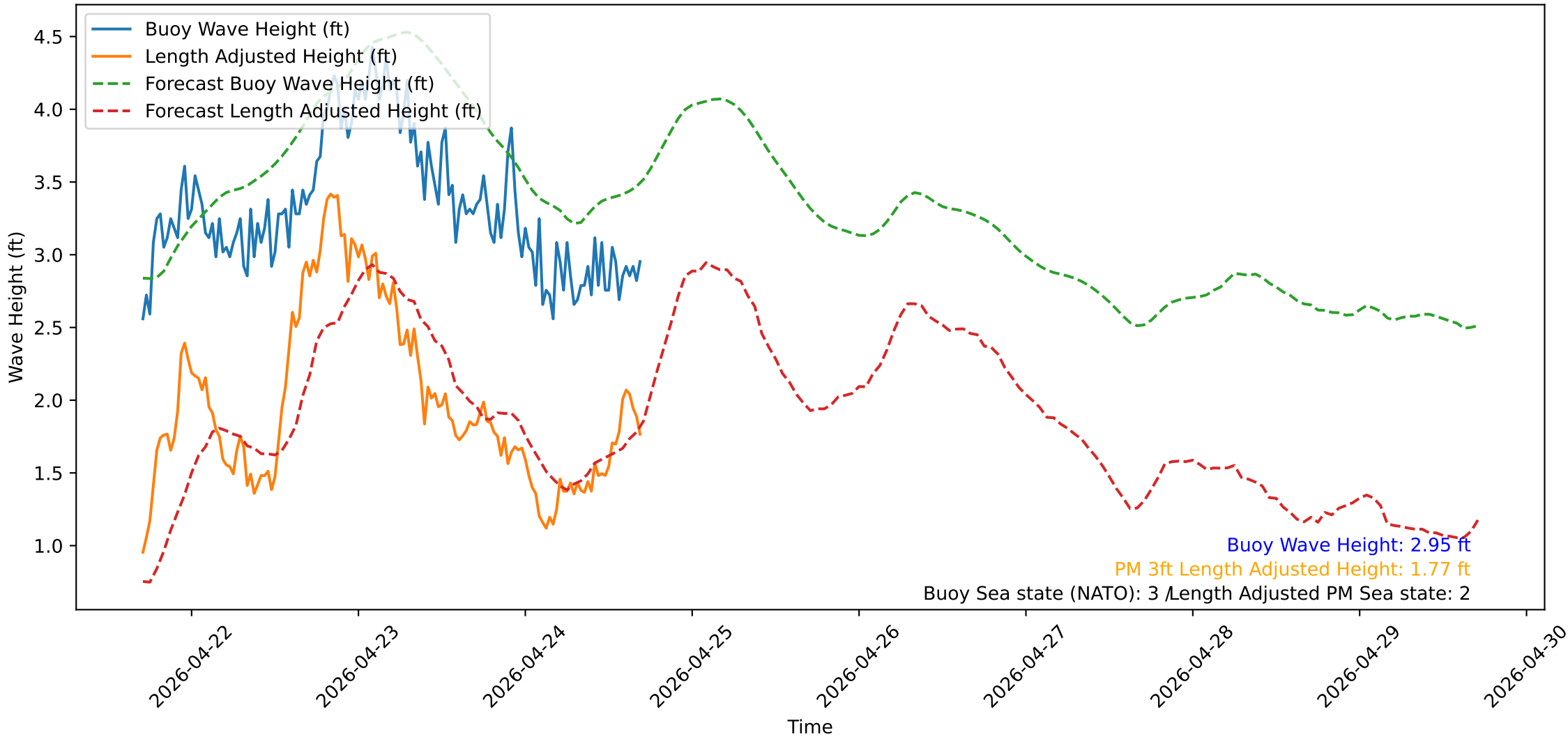
Wave Heights over Time for Oceanside Harbor at 2026-04-24 17:00:31
