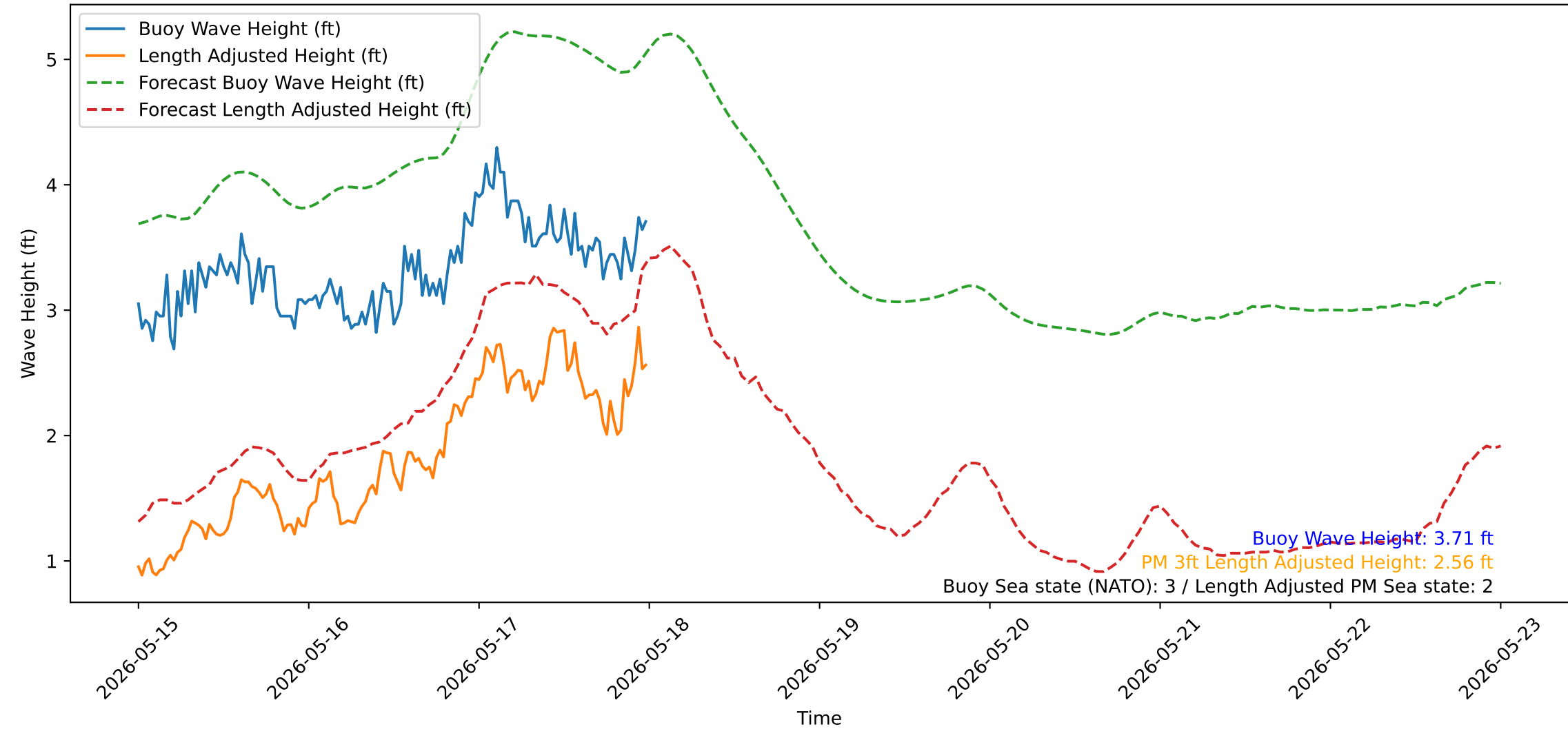
Wave Heights over Time for Oceanside Harbor at 2026-05-18 00:00:32
