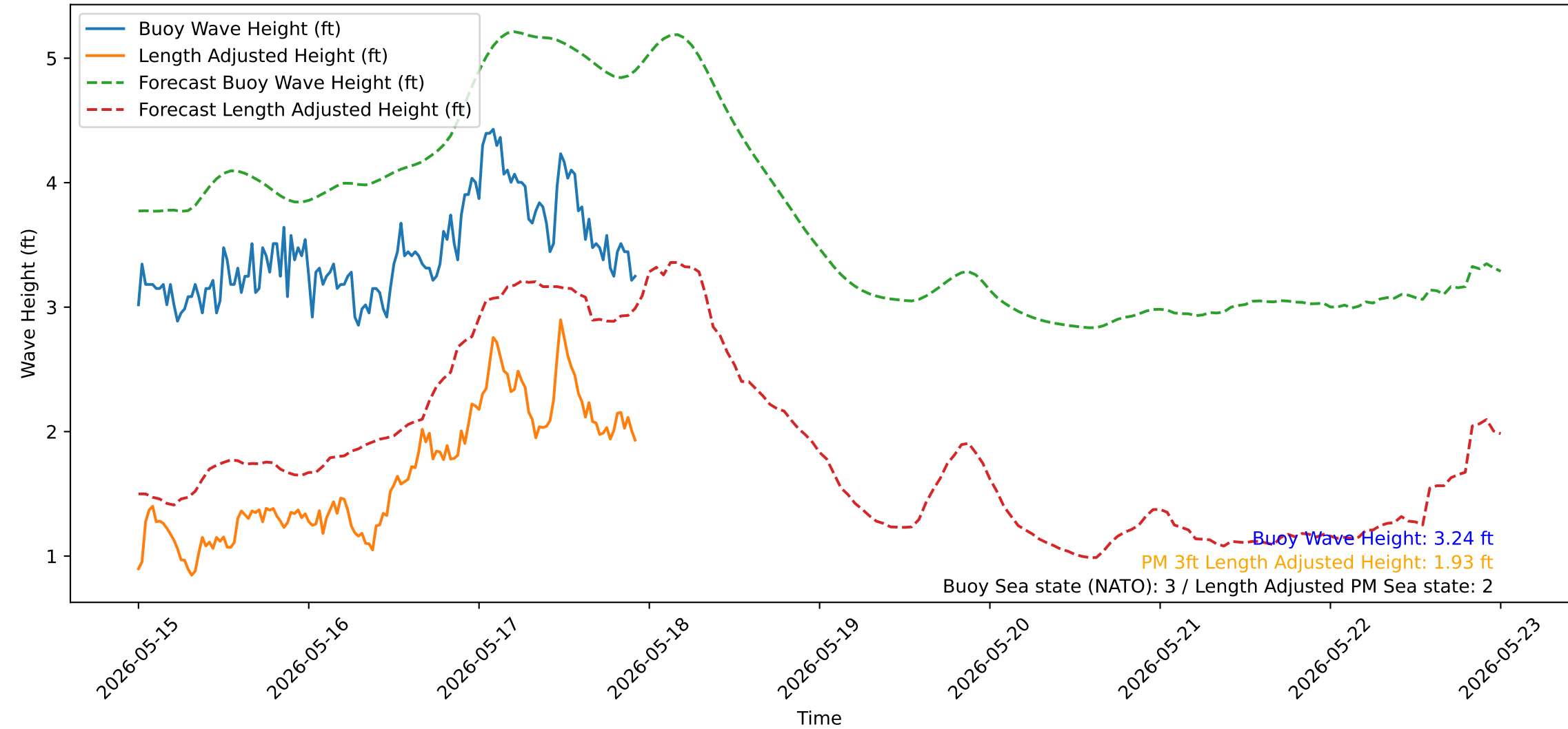
Wave Heights over Time for Green Beach at 2026-05-18 00:01:13
