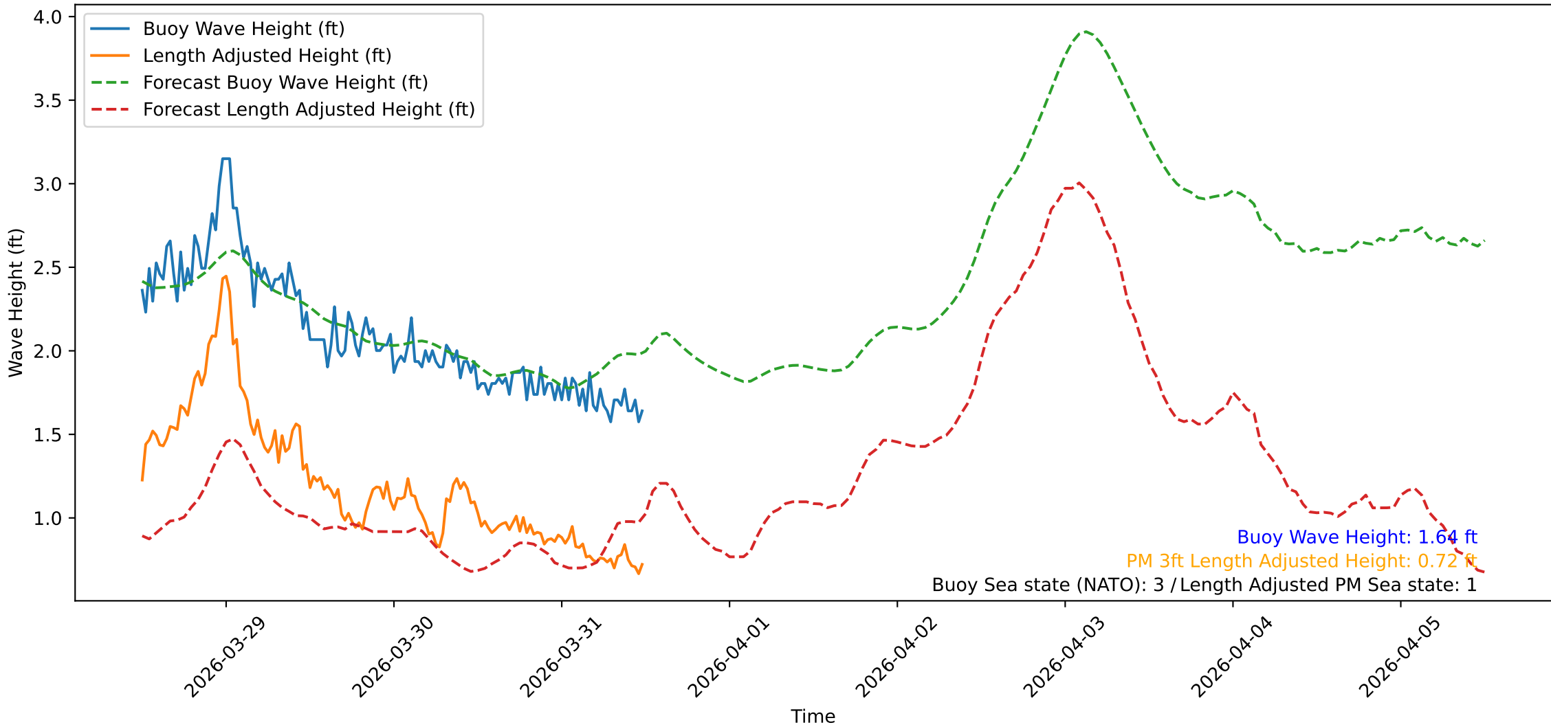
Wave Heights over Time for Oceanside Harbor at 2026-03-31 12:10:31
