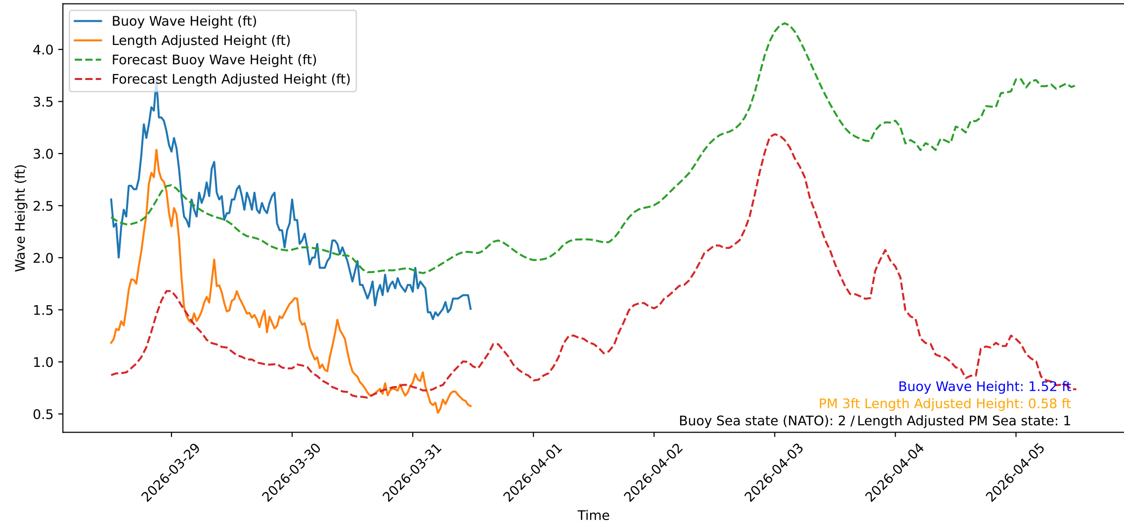
Wave Heights over Time for Green Beach at 2026-03-31 12:11:10
