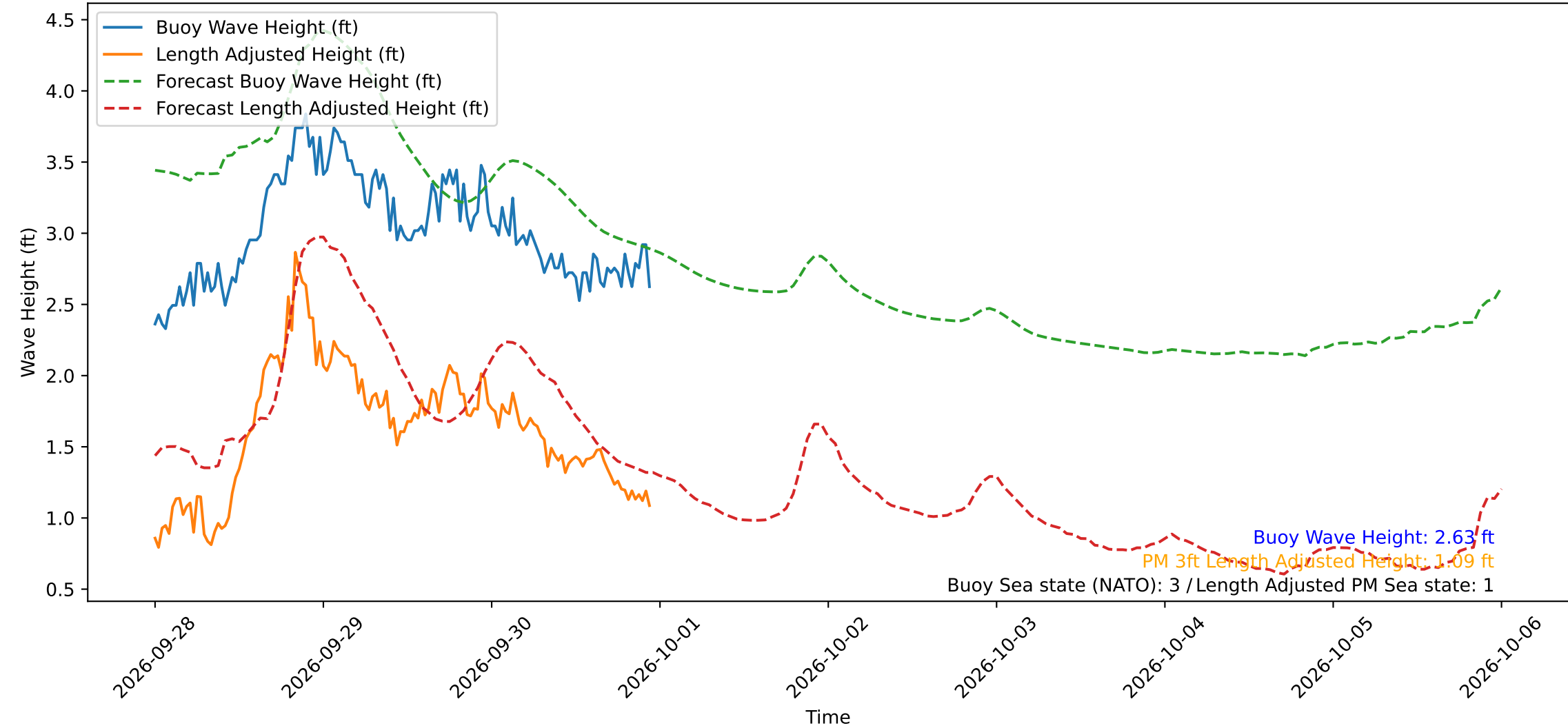
Wave Heights over Time for Red Beach at 2026-09-30 23:30:50
