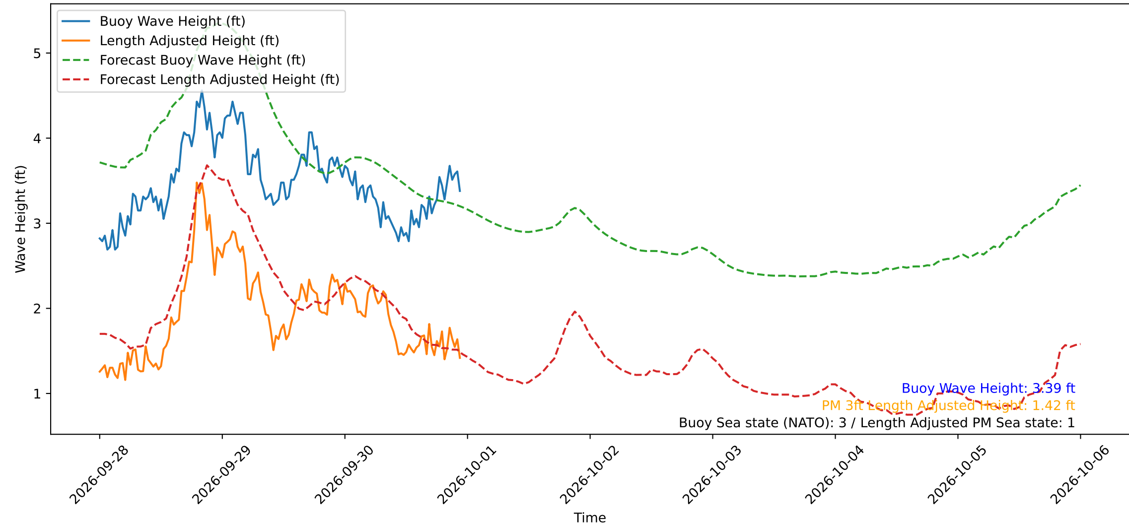
Wave Heights over Time for Green Beach at 2026-09-30 23:31:12
