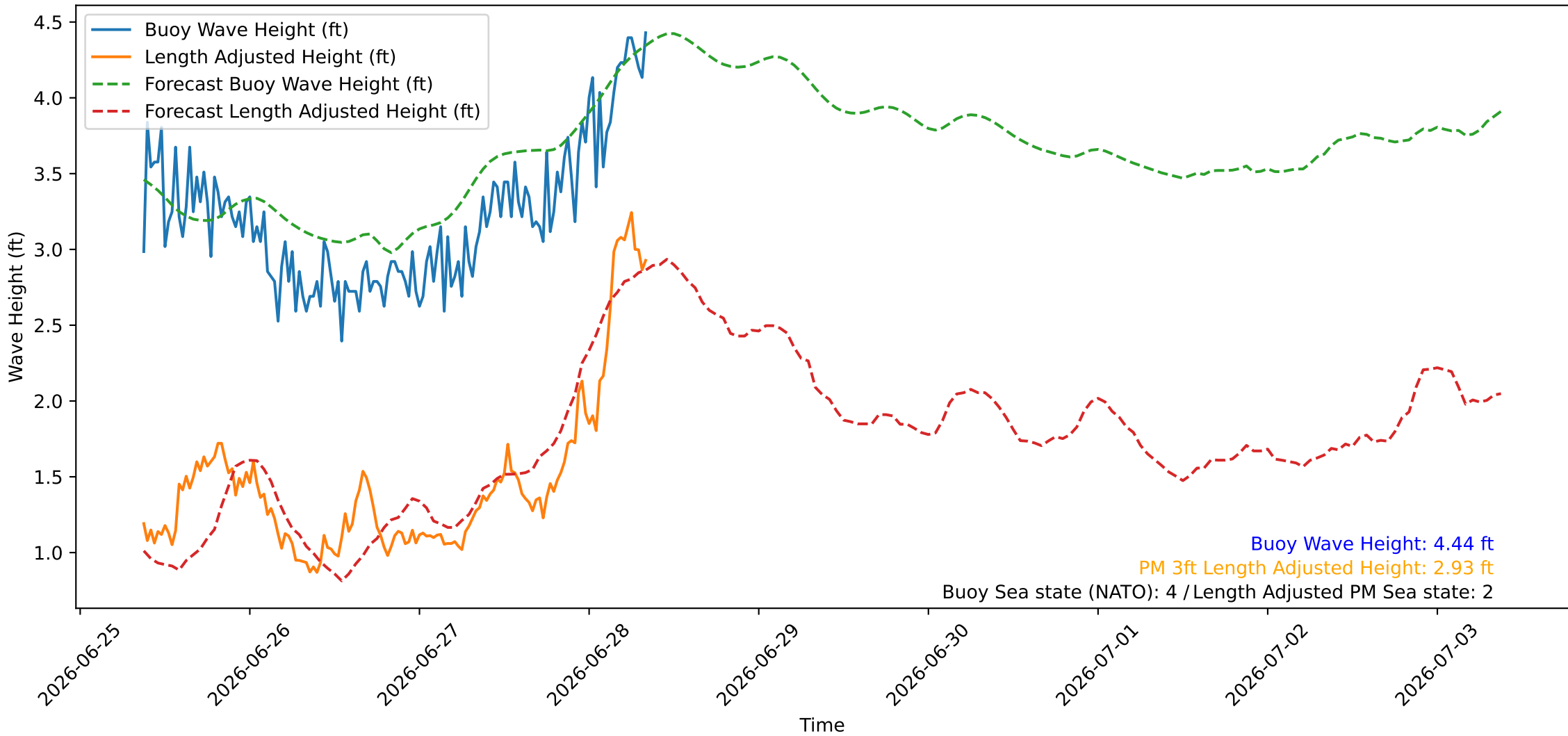
Wave Heights over Time for Oceanside Harbor at 2026-06-28 09:00:26
