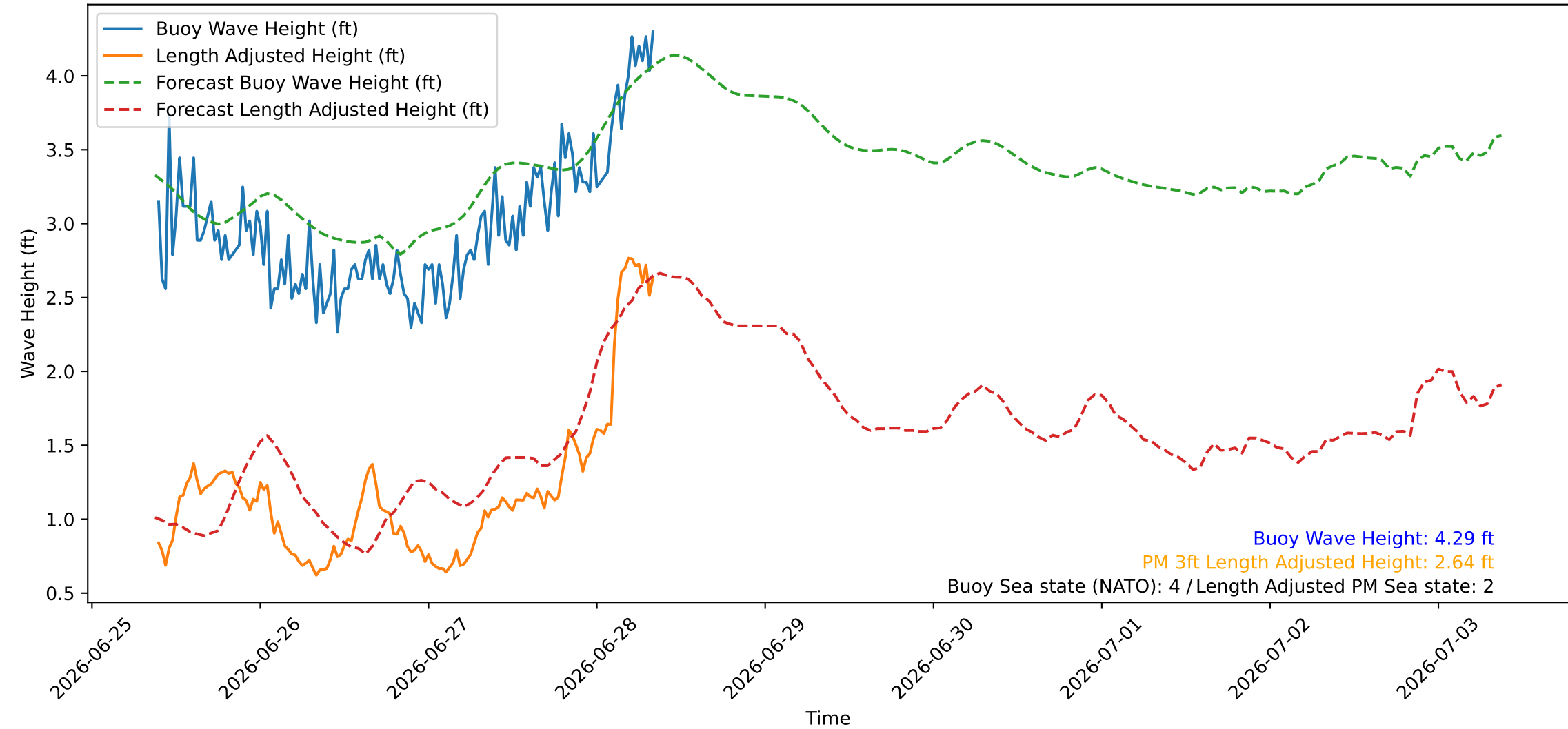
Wave Heights over Time for Red Beach at 2026-06-28 09:00:45
