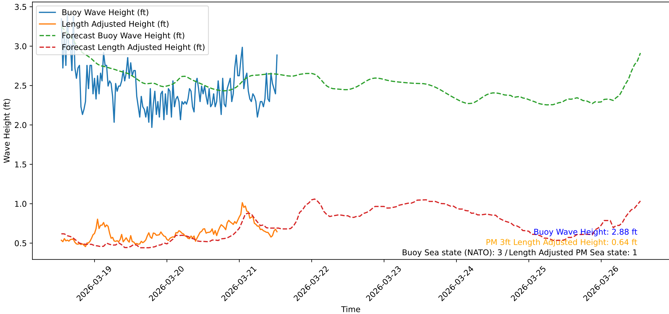
Wave Heights over Time for Oceanside Harbor at 2026-03-21 13:10:31
