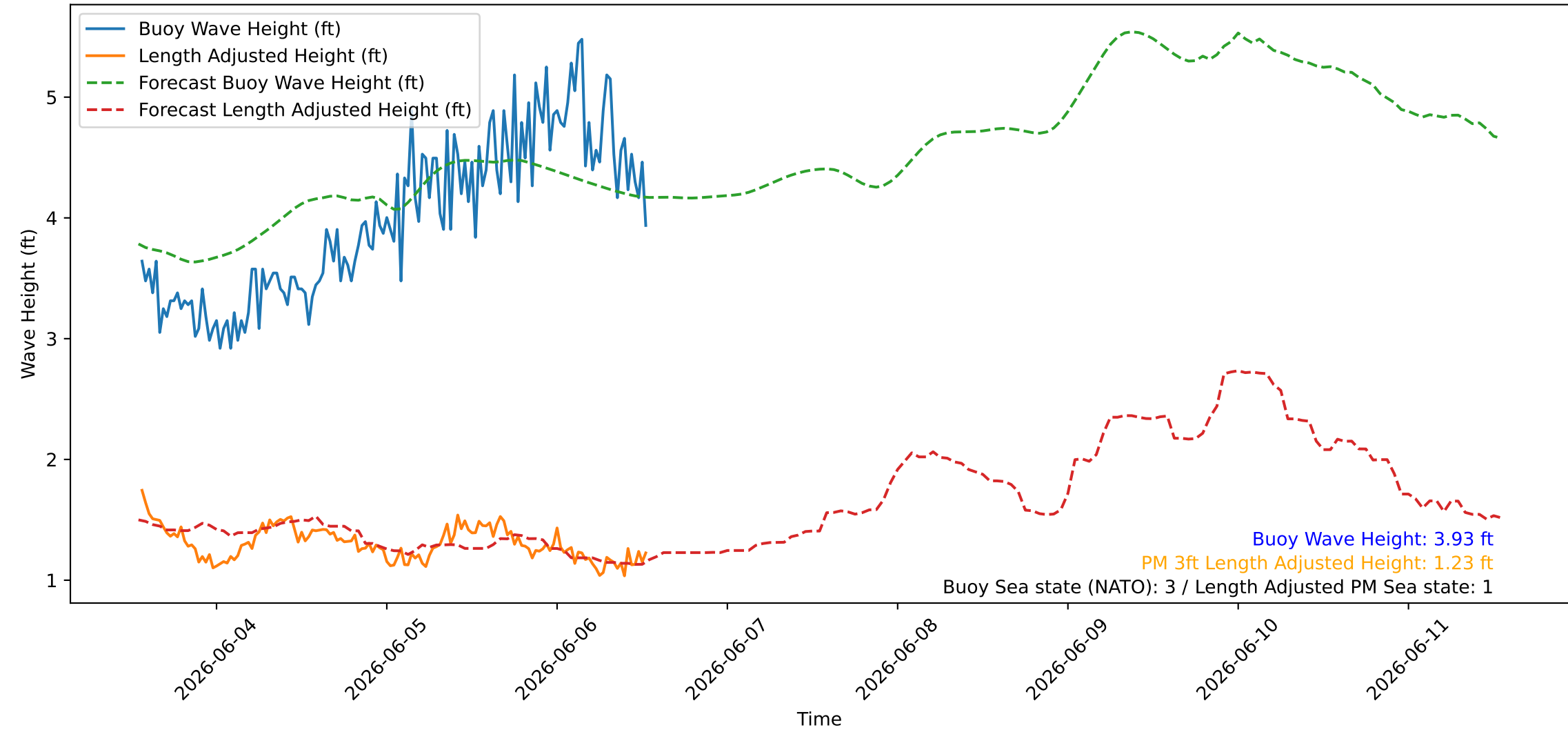
Wave Heights over Time for Oceanside Harbor at 2026-06-06 13:20:26
