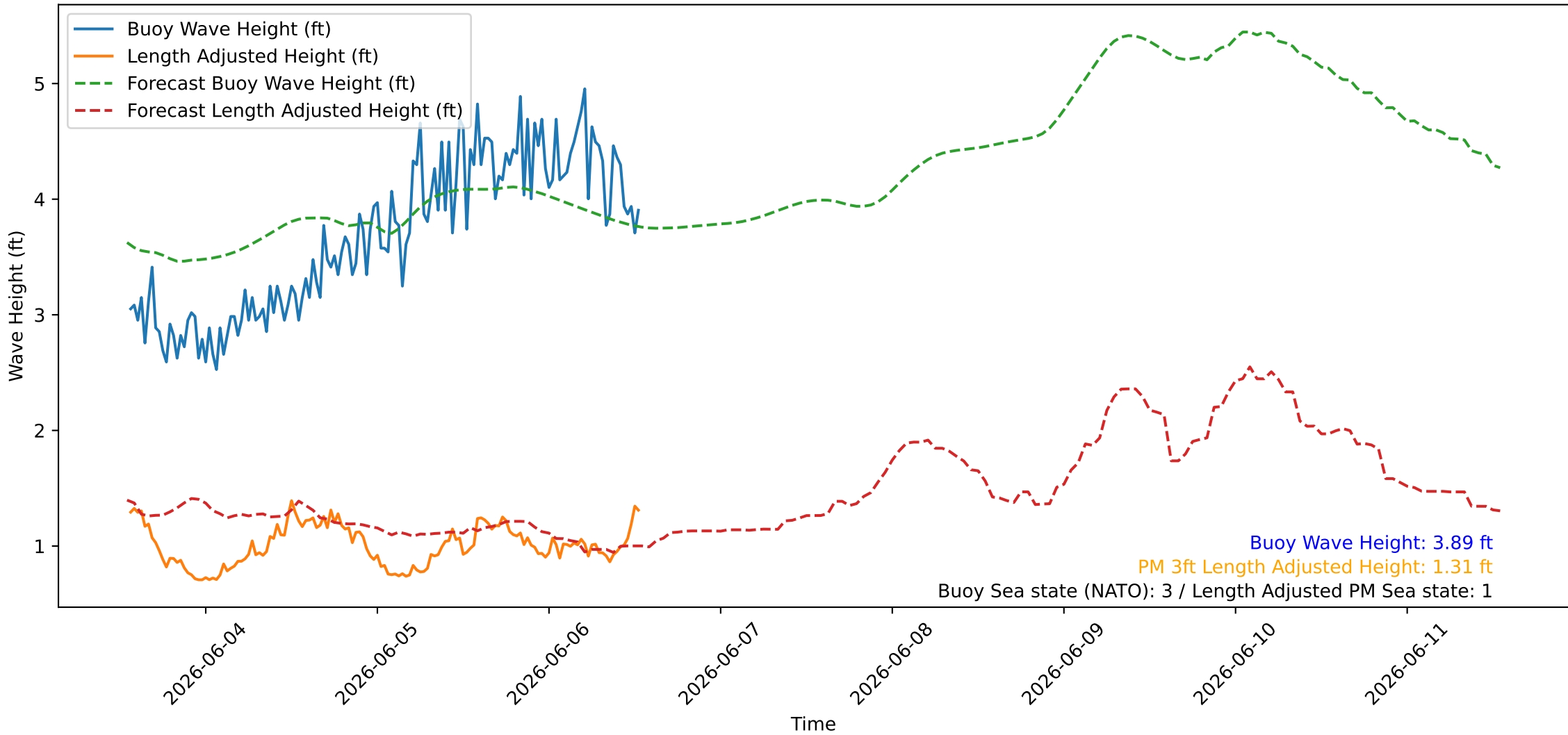
Wave Heights over Time for Red Beach at 2026-06-06 13:20:47
