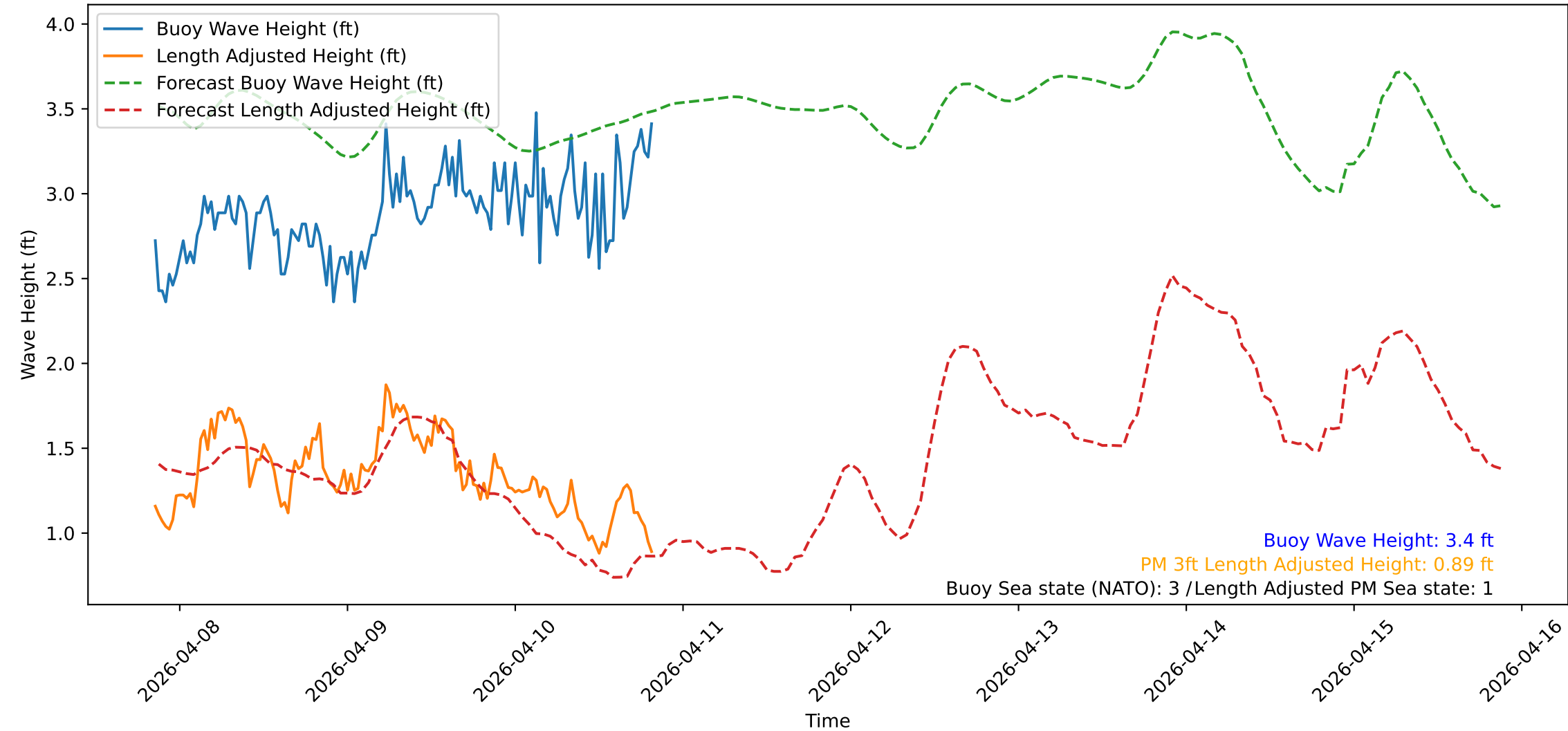
Wave Heights over Time for Green Beach at 2026-04-10 20:31:13
