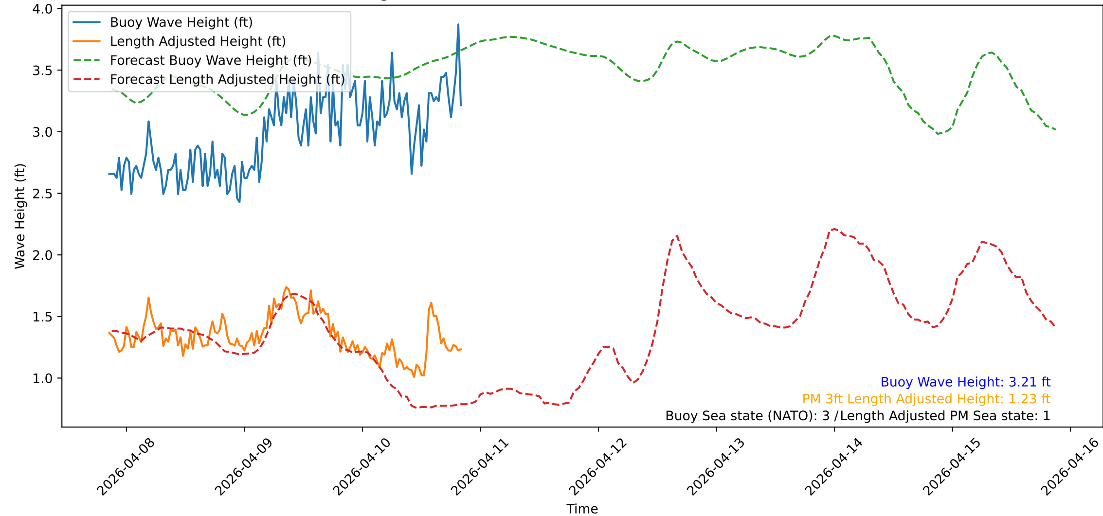
Wave Heights over Time for Oceanside Harbor at 2026-04-10 20:30:31
