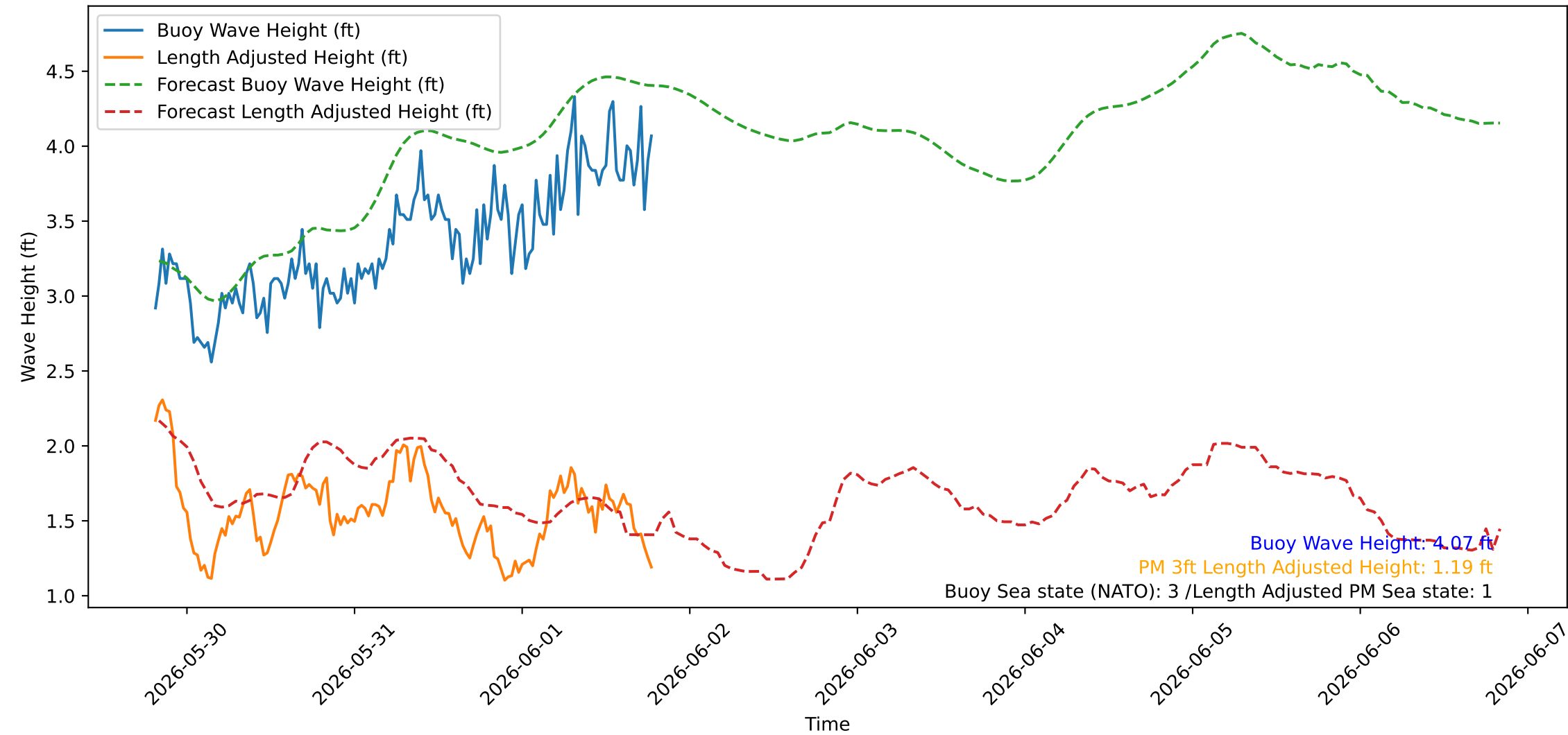
Wave Heights over Time for Green Beach at 2026-06-01 19:31:08
