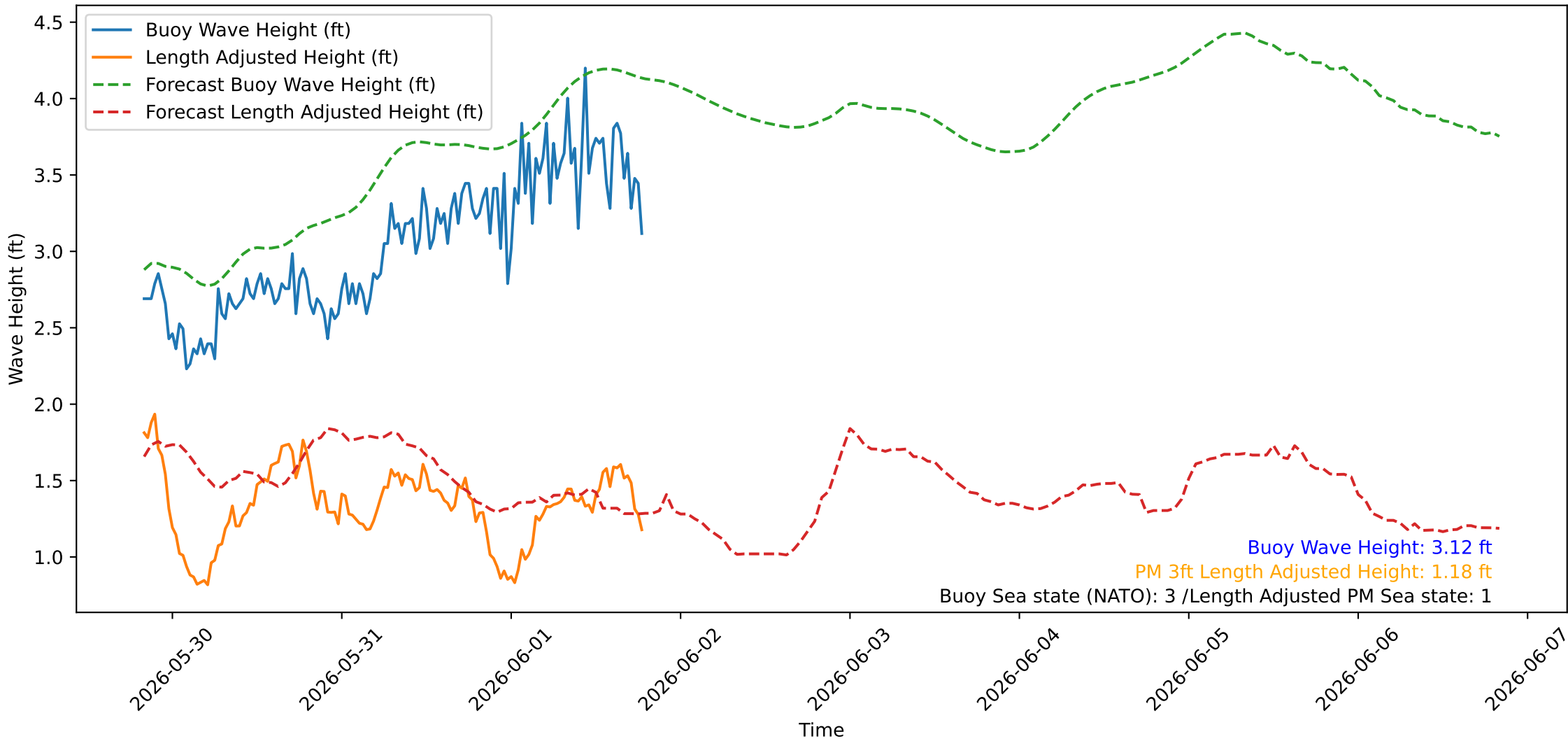
Wave Heights over Time for Red Beach at 2026-06-01 19:30:45
