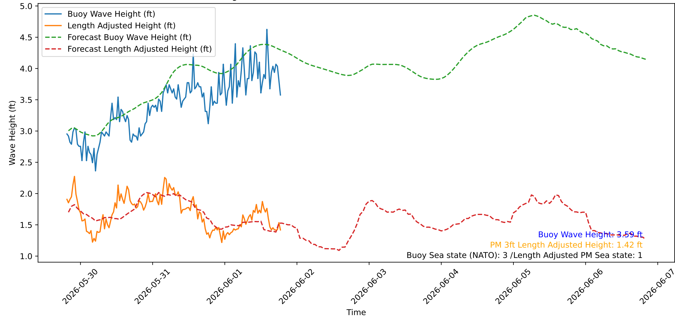
Wave Heights over Time for Oceanside Harbor at 2026-06-01 19:30:26
