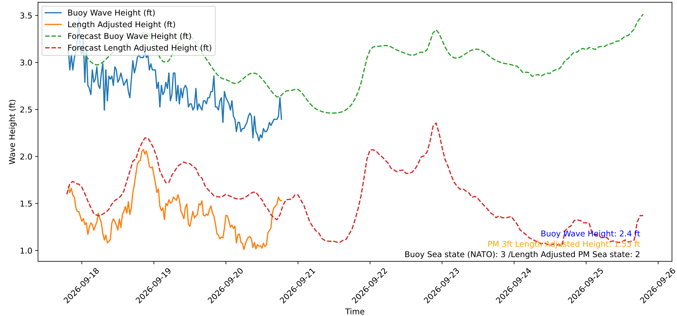
Wave Heights over Time for Green Beach at 2026-09-20 19:21:13
