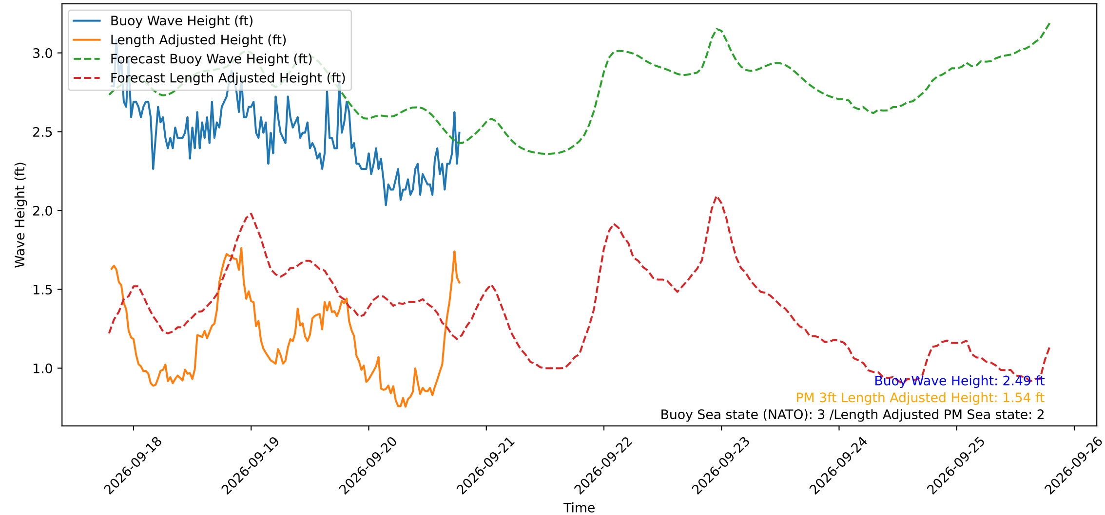
Wave Heights over Time for Red Beach at 2026-09-20 19:20:50
